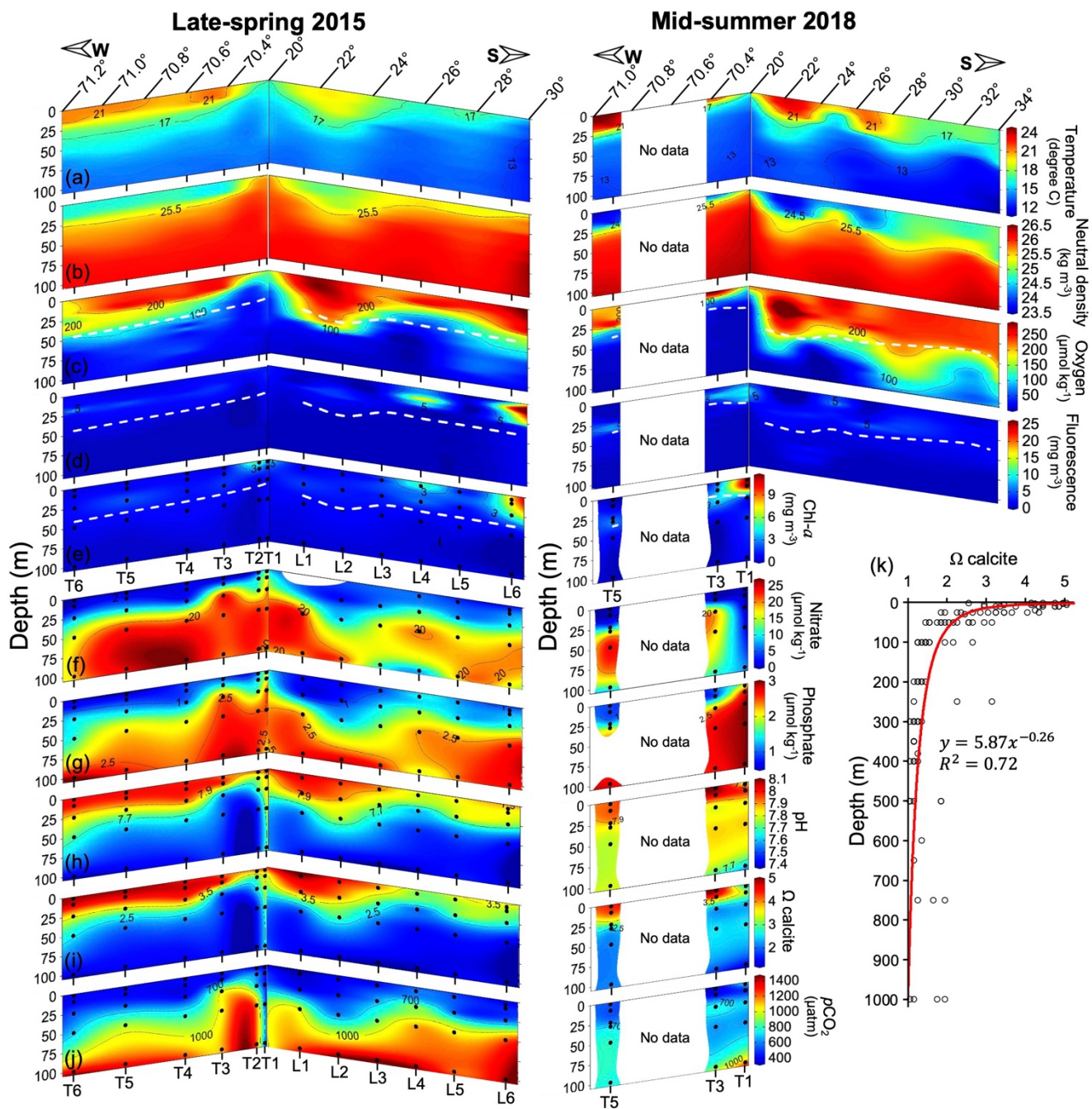
Figure 3: Spatial variation in temperature (a), neutral density (b), \text{O}_2 (c), fluorescence (d), \text{Chl-}a (e), nitrate (f), phosphate (g), pH (h), \Omega_{\text{calcite}} (i), and p\text{CO}_2 (j) within the upper 100 m, along with vertical distribution of \Omega_{\text{calcite}} down to 1000 m depth (k) during 2015 and 2018. In panels (e-j) sample locations are indicated by solid black circles. Continuous profiles in panels (a-d) are 1-m binned. Dashed white lines in panels (c-e) indicate the estimated euphotic depth. The red line in panel (k) represents a power trend curve.
