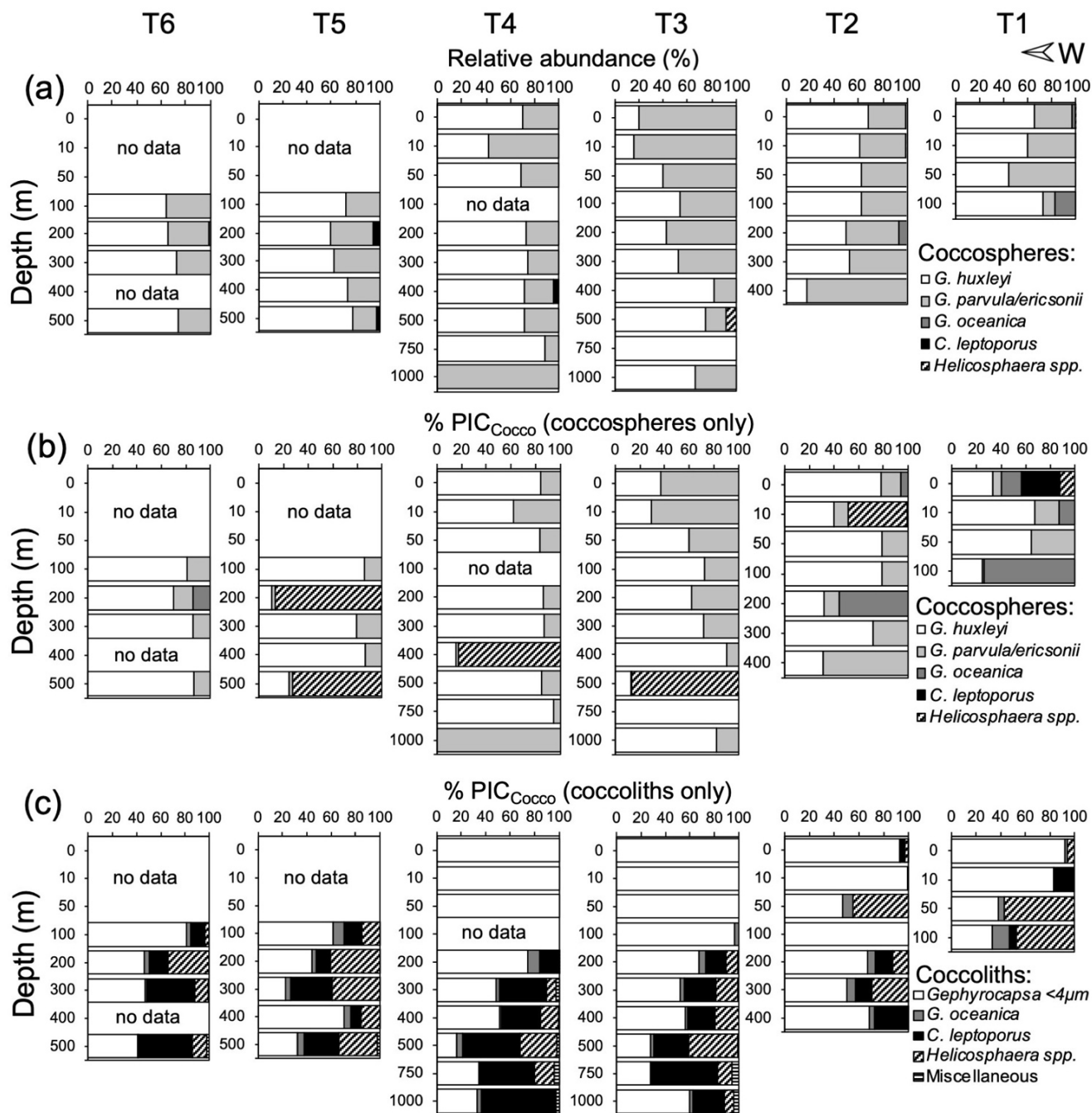
265 Figure 4: Relative abundance of coccospheres (a), and estimated PIC masses from coccospheres (b) and detached coccoliths (c) off Iquique (20° S) in 2015. (b-c) Taxonomic breakdown of the relative contributions of coccospheres and detached coccoliths to PIC Cocco quotas, expressed as percentages of the total PIC Cocco pool. The PIC Cocco pool estimate is based on abundances obtained via scanning electron microscopy.
