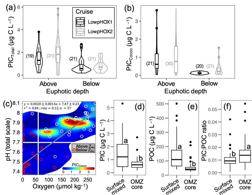
345 Figure 6: Violin plots showing the variation in \text{PIC}_{\text{Total}} (a) and \text{PIC}_{\text{Cocco}} (b), as well as \text{PIC}_{\text{Cocco}} in relation to \text{O}_2 and pH levels (c), above and below the euphotic depth in 2015 and 2018. Panels (d-f) display the values of PIC, POC, and PIC:POC ratios above and within the OMZ core during the same years. Only samples from the upper 100 m are included in panels (a-c). In panels (a-b), the number of samples per category is indicated in parentheses. In panel (c), horizontal and vertical white lines represent the projected pH for the year 2100 and the \text{O}_2 threshold for the Eastern Equatorial Pacific Ocean proposed by Stramma et al. (2008), respectively; the grey line indicates the least-squares model fit. In panels (d-f), all raw data are shown, with group comparisons based on robust two-sample bootstrapped tests (see Methods).
