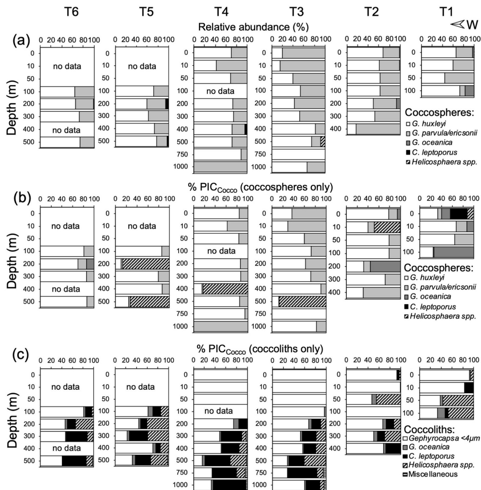
285 Figure 4: Relative abundance of coccospheres (a), and estimated PIC masses from coccospheres (b) and detached coccoliths (c) off Iquique (20° S) in 2015. (b-c) Taxonomic breakdown of the relative contributions of coccospheres and detached coccoliths to PIC Cocco quotas, expressed as percentages of the total PIC Cocco pool. The PIC Cocco pool estimate is based on abundances obtained via scanning electron microscopy.
