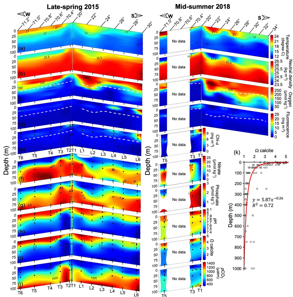
Figure 3: Spatial variation in temperature (a), neutral density (b), O 2 (c), fluorescence (d), Chl- a (e), nitrate (f), phosphate (g), pH (h), Ω calcite (i), and pCO 2 (j) within the upper 100 m, along with vertical distribution of Ω calcite down to 1000 m depth (k) during 2015 and 2018. In panels (e-j) sample locations are indicated by solid black circles. Continuous profiles in panels (a-d) are 1-m binned. Dashed white lines in panels (c-e) indicate the estimated euphotic depth. The red line in panel (k) represents a power trend curve.
