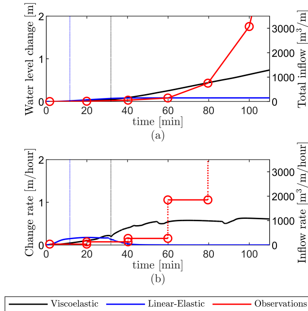
Figure 12. Model results using a linear-elastic (blue) and viscoplastic viscoelastic (black) ice rheology are compared to the reference observations (red, circles) from Das et al. (2008): (a) lake water level versus time (b) rate of water level change versus time. The vertical dotted line indicates the moment the vertical crevasse reaches the base of the ice sheet. For all lines, the vertical axis report the values in \text{m}^3/\text{m} , as directly resulting from simulations, on the right and on the left in \text{m} water-level change, converted using A_{\text{lake}} = 5.6 \text{ km}^2 and W_{\text{op}} = 3.2 \text{ km} .
