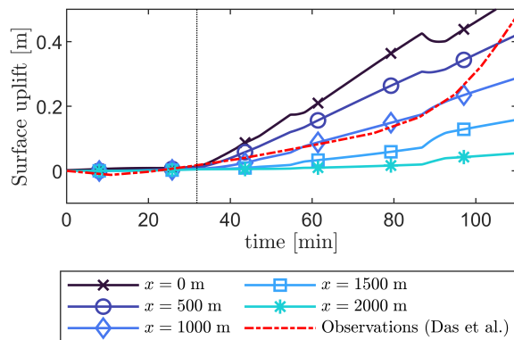
Figure 11. Vertical uplift of the ice sheet surface over time at set distances from the crevasse ( x = 0 m is at the crevasse and x = 500 m is 500 meters to the left/right of it), using the viscoplastic viscoelastic rheology. For comparison, observational data from Das et al. (2008) is included. The vertical dotted line indicates the moment the crack reaches the base of the ice sheet. (Linear-elastic uplift provided in the supporting information)
