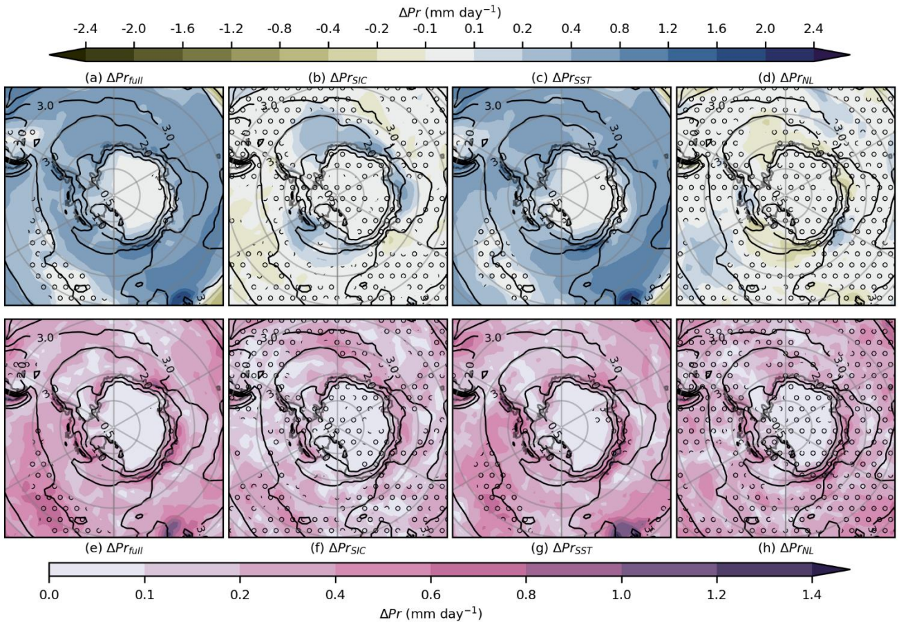
Figure 6. Difference in precipitation (Pr) in austral winter (JJA) between the SSP585 simulation and Baseline ( \Delta Pr_{full} , a, e), between SIC_SSP585 and Baseline ( \Delta Pr_{SIC} , b, f), between SST_SSP585 and Baseline ( \Delta Pr_{SST} , c, g) and the nonlinear ( \Delta Pr_{NL} residual) contribution (d, h). The upper row shows the multi-model mean and the lower row the maximum difference between models.
