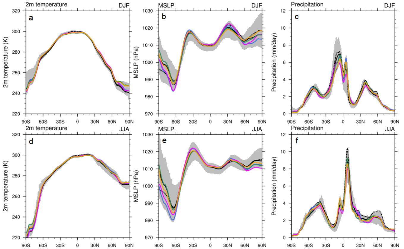
Figure 2. Seasonal means of zonal mean of 2m temperature (left, a, d), mean sea level pressure (middle, b, e), and precipitation (right, c, f), in the Baseline simulations and in the CMIP6 historical simulations (years 1950-1969). The blue (CESM2), magenta (NorESM2), green (EC-Earth3) and yellow (OpenIFS) lines show the models applied in the present study and the black solid line shows the CMIP6 multi-model mean and black dashed line shows ACCESS-ESM1.5 CMIP6 simulation where sea ice cover and SST were taken. The gray area shows the range between the minimum and maximum of the 23 CMIP6 models. The upper row shows mean values for northern hemisphere winter (DJF) and the lower row shows mean values for southern hemisphere winter (JJA).
