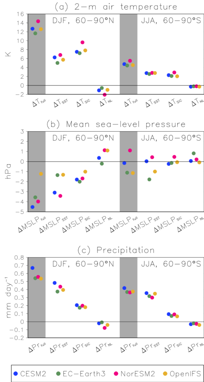
Figure 3. Area-mean differences between the SSP585 simulation and Baseline ( \Delta X_{full} , grey shading), between SIC_SSP585 and Baseline ( \Delta X_{SIC} ), between SST_SSP585 and Baseline ( \Delta X_{SST} ), and the nonlinear (residual) contribution ( \Delta X_{NL} ) for (left) northern high latitudes (60-90°N) in the northern hemisphere winter (DJF) and (right) southern high latitudes (60-90°S) in the southern hemisphere winter (JJA) for (a) 2m temperature, (b) mean sea-level pressure, and (c) precipitation.
