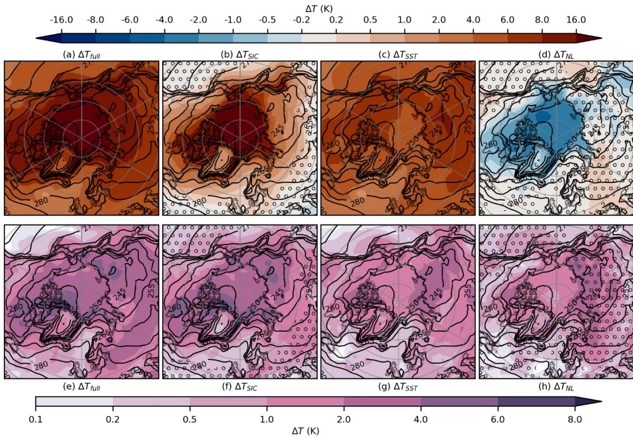
Figure 7. Difference in 2m temperature (T) in winter (DJF) between the SSP585 simulation and Baseline ( \Delta T_{full} , a, e), between SIC_SSP585 and Baseline ( \Delta T_{SIC} , b, f), between SST_SSP585 and Baseline ( \Delta T_{SST} , c, g) and the nonlinear ( \Delta T_{NL} residual) contribution (d, h). The upper row shows the multi-model mean and the lower row the maximum difference between models. Stippling indicates that all models do not agree on the direction of the change and contours show the 2m temperature in Baseline simulation.
