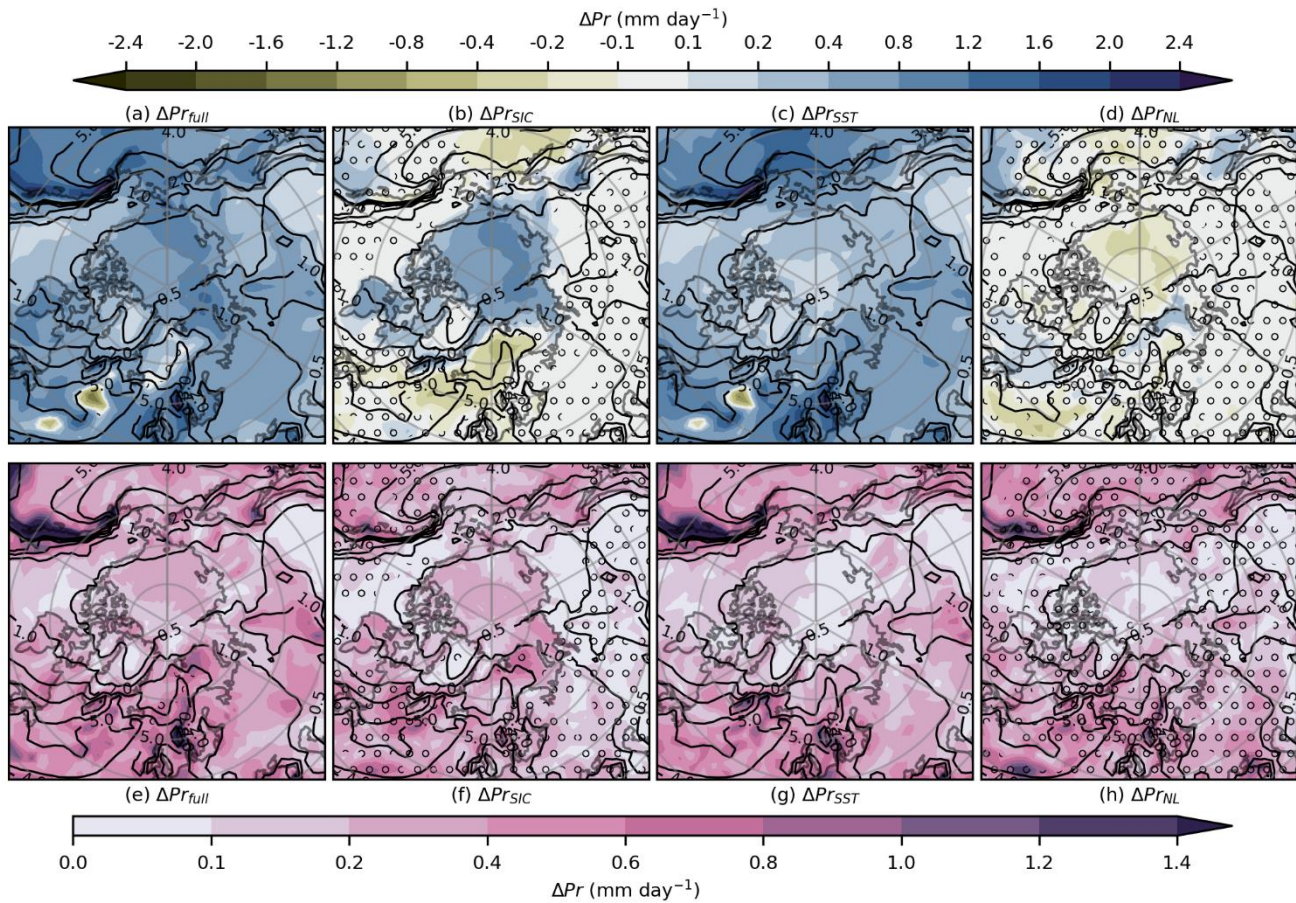
Figure 9. Difference in precipitation (Pr) in winter (DJF) between the SSP585 simulation and Baseline ( \Delta Pr_{full} , a, e), between SIC_SSP585 and Baseline ( \Delta Pr_{SIC} , b, f), between SST_SSP585 and Baseline ( \Delta Pr_{SST} , c, g) and the nonlinear ( \Delta Pr_{NL} residual) contribution (d, h). The upper row shows the multi-model mean and the lower row the maximum difference between models. Stippling indicates that all models do not agree on the direction of the change and contours show the precipitation in Baseline simulation.
