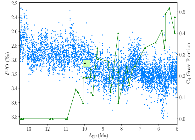
Figure 9. \text{C}_4 grassland expansion, inferred from plant wax carbon isotopes in marine sediments (Polissar et al., 2019), shown alongside \delta^{18}\text{O} values. The estimated breakpoint, \text{BP}_{10} (black dot), and its confidence interval (light green bar), align with this ecological transition.
