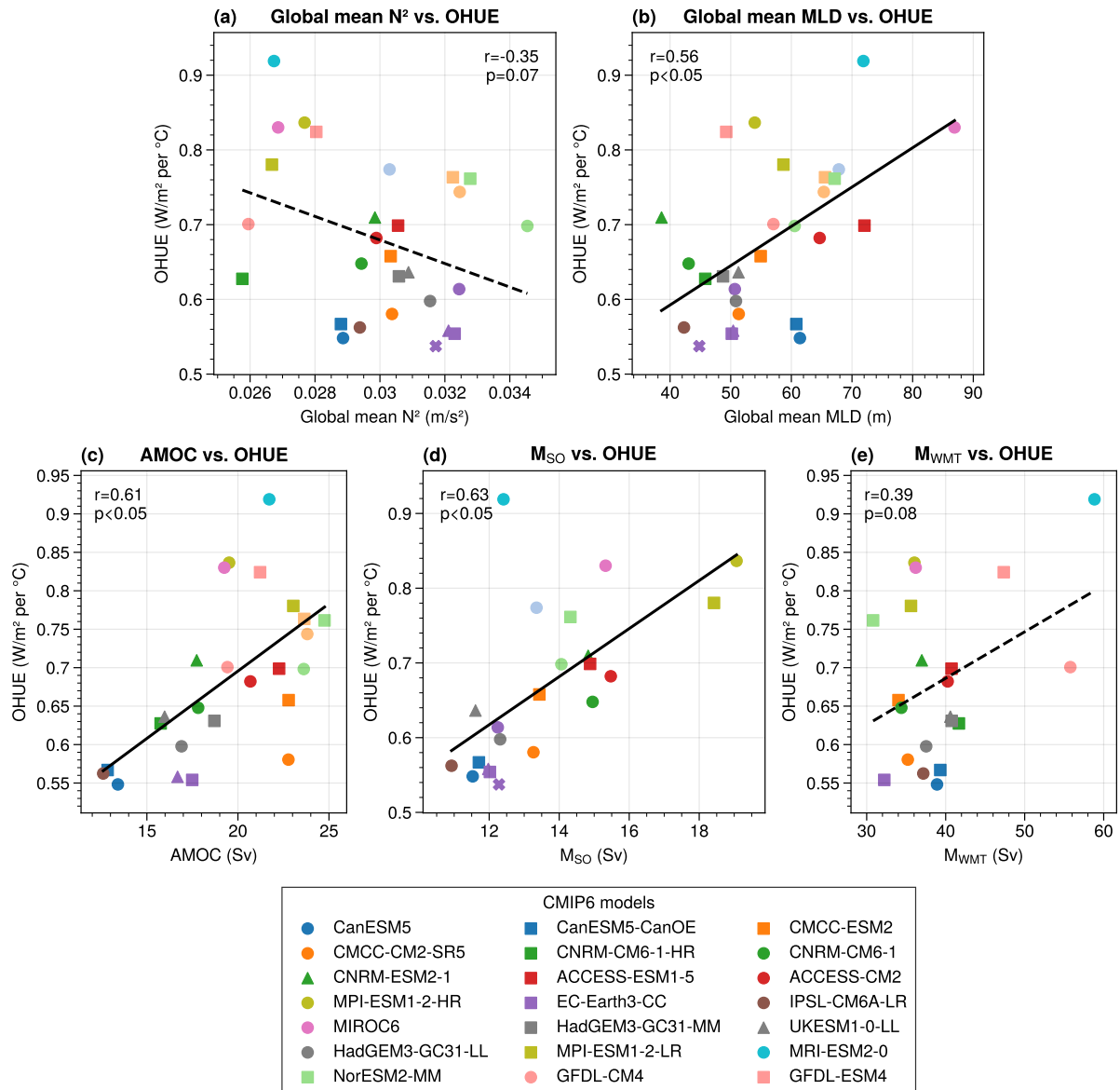
Figure 1. Proposed controls on ocean heat uptake efficiency (OHUE). Scatter plot between OHUE and (a) preindustrial global mean upper ocean (0–1500 m) stratification ( N^2 ), (b) preindustrial global mean mixed layer depth (MLD), (c) preindustrial mean AMOC strength, (d) Southern Ocean upper cell strength, and (e) Southern Ocean surface buoyancy flux inferred overturning. In panels (c)–(e), only a subset of models is included due to output availability (see Table A1).
