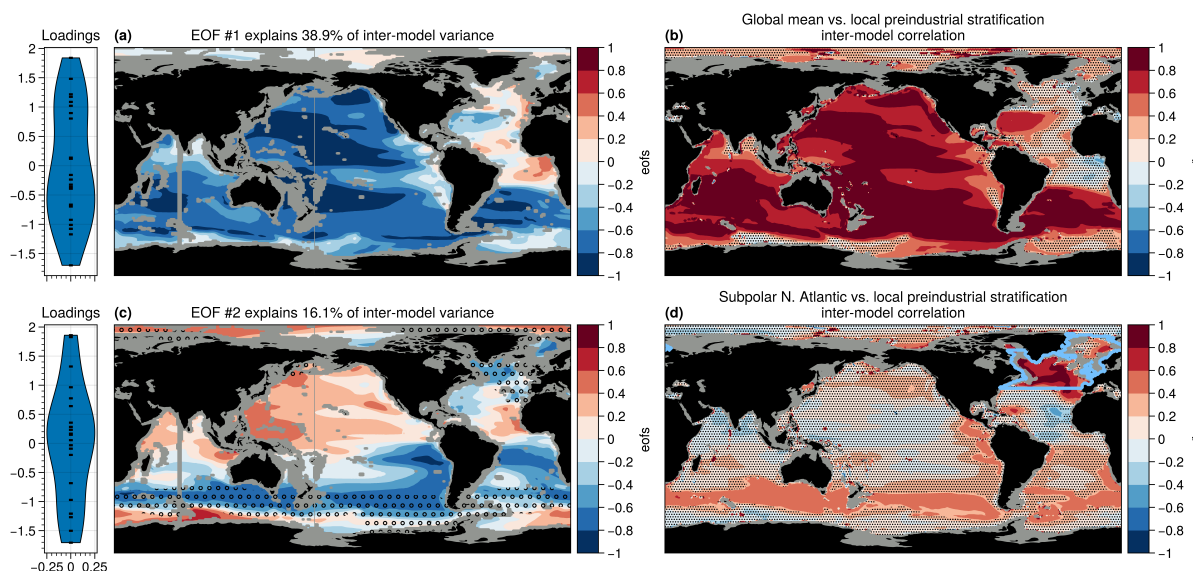
Figure 5. Regional coherence of inter-model stratification spread. Panels (a) and (c) show respectively the first and second mode of inter-model EOF analysis on preindustrial annual mean upper ocean stratification (see Methods). The violin plots in panels (a) and (c) show the ensemble distribution of the normalized loadings for each EOF. In panel (c), stippling indicates areas with surface density in the range 25.75 \text{ kg m}^{-3} < \sigma_0 < 27 \text{ kg m}^{-3} . Panels (b) and (d) show the inter-model correlation between the local preindustrial stratification and either (b) the global mean preindustrial stratification or (d) the subpolar North Atlantic mean preindustrial stratification. The subpolar North Atlantic region used in panel (d) is indicated by the blue contour.
