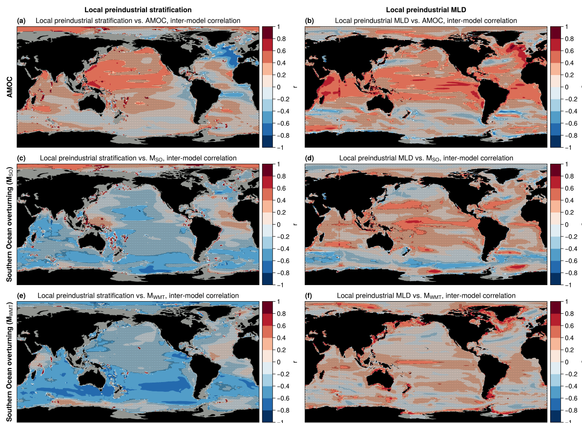
Figure 3. Local upper-ocean controls on meridional overturning strength in CMIP6. Left column: maps of inter-model Pearson correlation coefficient across 28 CMIP6 models between local preindustrial annual mean upper ocean (0–1500 m) stratification and (a) preindustrial mean AMOC strength, (c) Southern Ocean upper cell strength, and (e) Southern Ocean surface buoyancy flux inferred overturning. Right column [(b), (d), (f)]: as left column, but for local preindustrial annual mean mixed layer depth.
