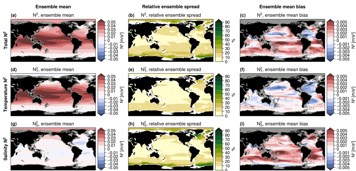
Figure 4. Ensemble mean stratification and bias relative to observations. (a) CMIP6 ensemble mean total historical stratification integrated over the 0–1500 m depth range. (b), Inter-model coefficient of variation (ratio of ensemble standard deviation to ensemble mean) of total stratification. (c), Bias in total stratification between CMIP6 ensemble mean and the ECCO state estimate. (d)–(f), As (a)–(c) but for temperature stratification. (g)–(i), As (a)–(c) but for salinity stratification. For both the model ensemble and the state estimate, stratification is averaged over the historical period 1992–2017.
