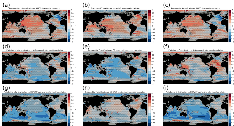
Figure A2. Inter-model relation between stratification and overturning cells. (a)–(c): inter-model correlation between preindustrial 0–1500 m stratification and AMOC for total (left column), temperature (middle column), and salinity (right column) stratification. (d)–(f): as in (a)–(c) but for the Southern Ocean upper cell in density coordinates. (g)–(i): as in (a)–(c) but for the Southern Ocean overturning strength inferred from surface buoyancy fluxes (see Methods). Note that the first column of this figure is the same as the first column of Fig. 3 in the main text.
