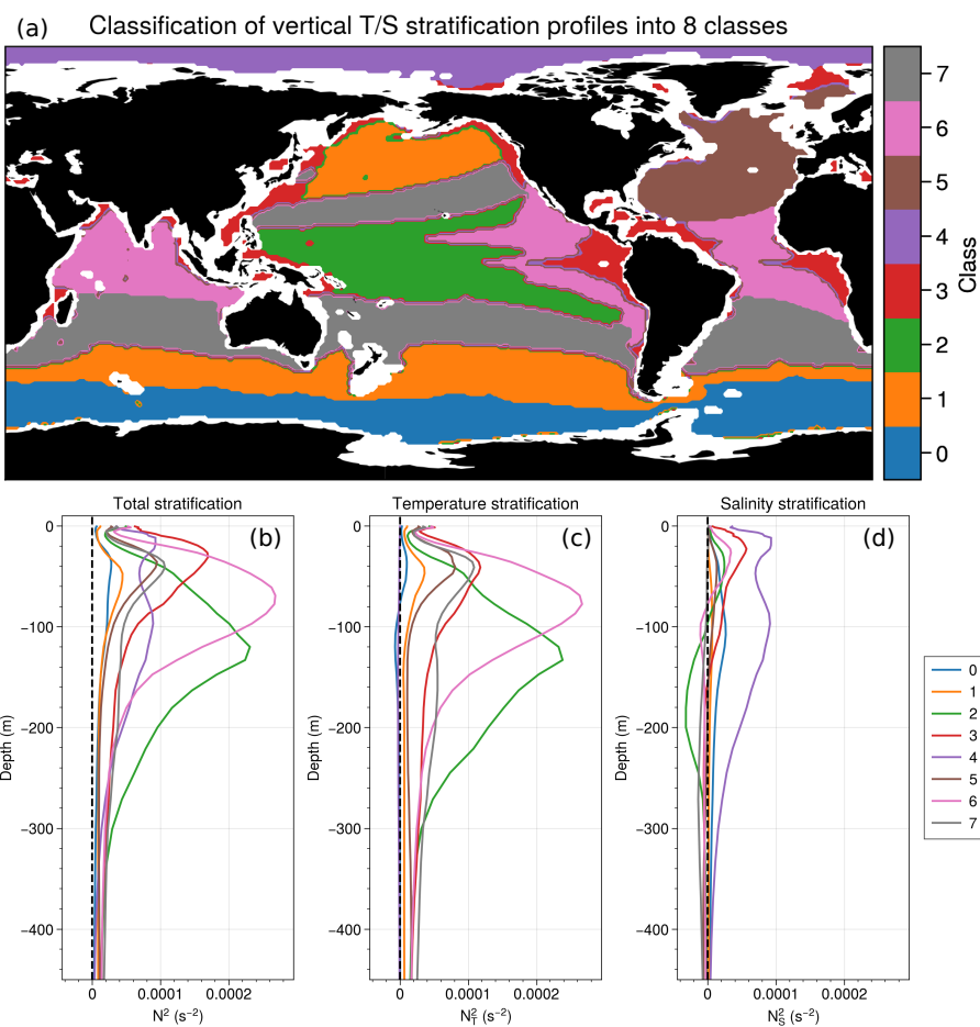
Figure A7. Classification of vertical stratification profiles. (a), map showing the geographical location of identified classes. (b)–(d), median vertical stratification profiles of each class (for total, temperature, and salinity stratification).
