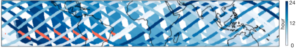
Figure 1. Illustration of the temporal and spatial match between Aqua–AIRS and TRMM–PR orbits. Orange represents the satellite trace segments, coincident within a time window of \pm 20 minutes, for one specific day. The narrow swaths represent TRMM–PR orbits, while the broader swaths represent Aqua–AIRS orbits. Shades of blue indicate variations in sampling time difference.
