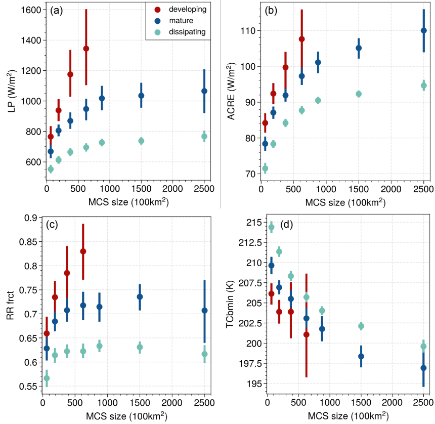
Figure 13. LP (a), ACRE (b), rainy area fraction (c) and minimum cloud top temperature within the convective core (d), as a function of the CS size, separately for developing, mature and dissipating CSs (distinguished by convective core fraction: 0.6–0.9, 0.4–0.6 and 0.2–0.4, respectively). All size intervals except the first two include exclusively MCSs. Choosing the coldest part of the core avoids to include parts of the thicker anvil. CSs over ocean, 1:30 AM/PM local time, 2004–2018, 25°N–25°S.
