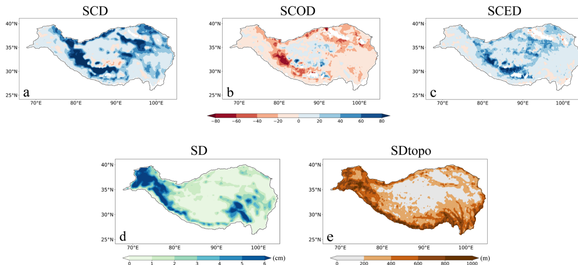
385 Figure 9. Spatial distribution of differences in (a) snow cover duration (SCD), (b) snow cover onset days (SCOD), and (c) snow cover end day (SCED) extracted by the snow dynamic threshold method and the traditional fixed threshold method on the Tibetan Plateau. Unit is DOHY (Day of the Hydrological Year). Spatial distribution of (d) multi-year mean snow depth (SD) and (e) standard deviation of topography (SDtopo) on the Tibetan Plateau (TP).
