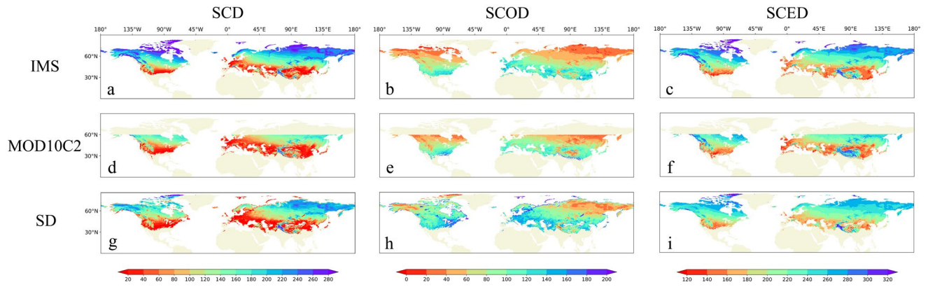
Figure 2. Spatial distribution of snow phenology extracted by the fixed threshold method over the Northern Hemisphere for the hydrological years 2000-2018. (a) Multiyear averaged snow cover duration (SCD), (b) snow cover onset day (SCOD), (c) snow cover end day (SCED) based on the IMS dataset. (d, e, f) Same as (a, b, c) but for the MOD10C2 dataset. (g, h, i) Same as (a, b, c) but for the SD dataset. The unit DOHY is an abbreviation for day of the hydrological year, defined as September 1 through August 31 of the following year.
