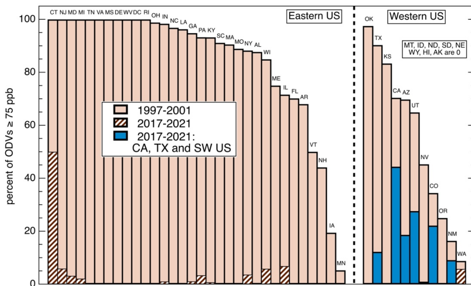
1075 Figure 9: Comparison of percentage of ODVs greater than or equal to 75 ppb recorded at all sites in individual states over two 5-year periods: 2017-2021 (hatched and dark blue bars) and a period 20 years earlier - 1997-2001 (light-colored bars). Individual states are indicated by their two letter abbreviations (defined in Table S6). States are arbitrarily divided between eastern and western regions. Southwestern states, Texas and California are indicated by solid dark blue bars. Eight rural states, all in the western region, reported no ODVs greater than or equal to 75 ppb in either period.
