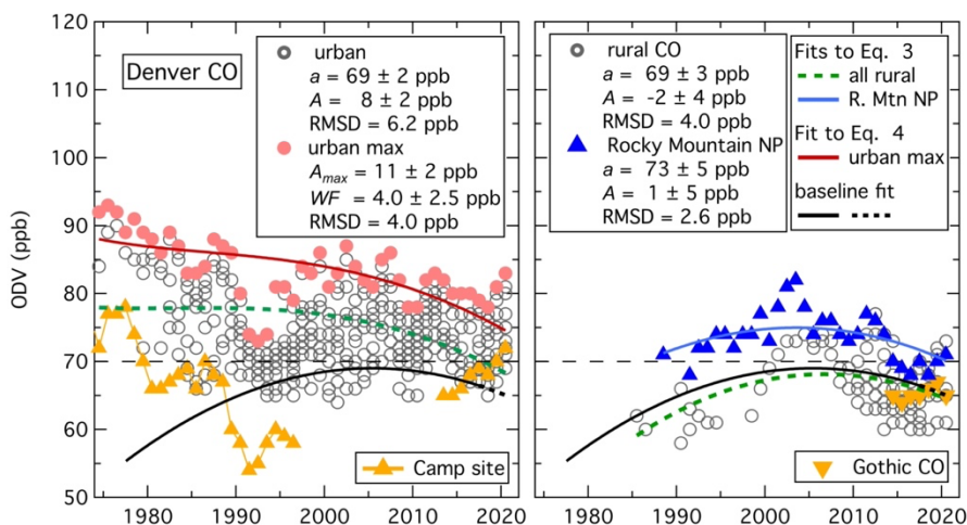
1050 Figure 5: Time series of ODVs recorded in Colorado at the urban sites (left graph) whose locations are shown in Figure 4, and at rural sites (right graph, excluding the Four Corners area) whose locations are shown in Figure S1. Open symbols indicate all ODVs recorded in each area, and solid symbols indicate ODVs from three specific sites and the maximum Denver urban ODVs. As indicated by an annotation on the right graph, green dashed curves indicate fits of Equation 3 to all plotted ODVs (excluding the Camp and Rocky Mountain NP sites, blue curve on right indicates Rocky Mountain NP fit of Equation 3, and red solid curve on left indicates fit of Equation 4 to the maximum Denver urban ODVs; parameters derived in these fits are annotated in the graphs. The black solid curves with dashed extensions indicate the fit to the baseline data included as the grey curve in Figure 1. The light dashed lines indicate the 70 ppb ozone NAAQS. 1055
