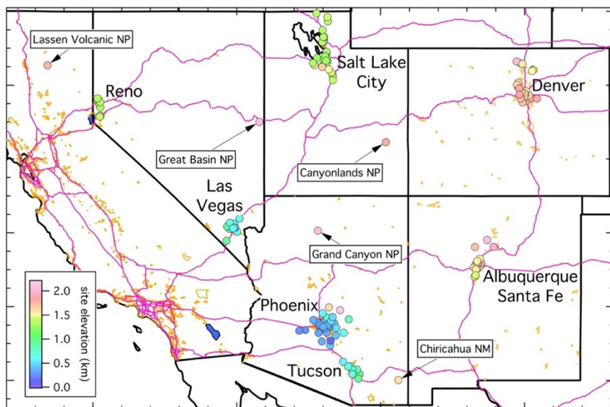
1045 Figure 4: Map of southwestern US urban monitoring sites; the symbols are color-coded according to site elevation as indicated in the annotation. Lines indicate outlines of southwestern US states (black), urban areas (gold) and interstates and selected other major highways (violet). Seven urban areas, whose sites are analyzed together as separate data sets, are labelled. Locations of five of the isolated rural CASTNET sites are also included.
