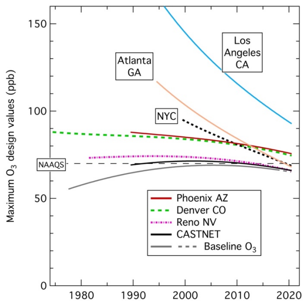
115 Figure 13: Comparison of fits of Equation 4 to time series of maximum ODVs recorded in three of the nation’s largest urban areas and three southwestern urban areas, with the fits to normalized rural western CASTNET ODVs and baseline ozone from Figure 1. The fitted urban curves are taken from Figure 2 of Parrish et al. (2022) for Los Angeles, Figure S6 for New York City (i.e., NYC) and Atlanta GA, Figure 5 for Denver CO, Figure 6 for Phoenix AZ and Reno NV, and Figure 1 for CASTNET and baseline ozone.
