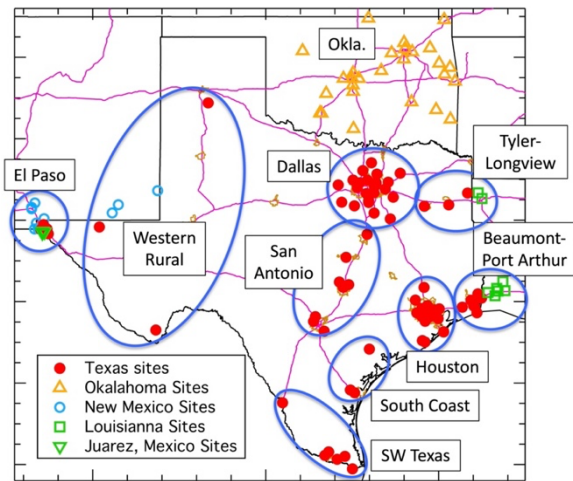
1065 Figure 7: Map of monitoring sites within the Texas region; the symbols are color-coded according to state as indicated in the annotation. Lines indicate outlines of southwestern US states (black), urban areas (gold) and interstates (violet). Nine Texas regions, whose sites are analyzed together as separate data sets, are indicated.
