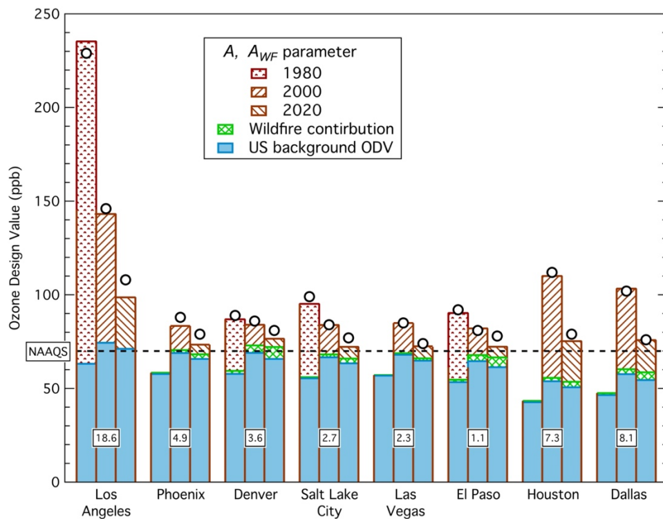
1105 Figure 12: Derived apportionment of maximum ODVs for 3 years at 20-year intervals for the Crestline site in Los Angeles, four southwestern US and three Texas urban areas. The lower, solid blue bars indicate the US background ODV; they exclude estimated wildfire contributions, which are separately indicated by the middle, cross-hatched green bar segments. The top, brown patterned bars indicate the estimated US anthropogenic ODV enhancements, again excluding the wildfire contribution. For four cities the US anthropogenic ODV enhancements and wildfire contributions are missing in 1980 since the tabulated ODVs are inadequate to estimate that parameter that early in the monitoring record. The 2020 populations of the urban areas are annotated in millions. The circles indicate the actual maximum ODVs recorded in the respective years in each area.
