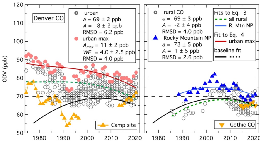
1015 Figure 5: Time series of ODVs recorded in Colorado at the urban sites (left graph) whose locations are shown in Figure 4, and at rural sites (right graph, excluding the Four Corners area) whose locations are shown in Figure S1. Open symbols indicate all ODVs recorded in each area, and solid symbols indicate ODVs from three specific sites and the maximum Denver urban ODVs. As indicated by an annotation on the right graph, green dashed curves indicate fits of Equation 3 to all plotted ODVs (excluding the Camp and Rocky Mountain NP sites, blue curve on right indicates Rocky Mountain NP fit of Equation 3, and red solid curve on left indicates fit of Equation 4 to the maximum Denver urban ODVs; parameters derived in these fits are annotated in the graphs. The black solid curves with dashed extensions indicate the fit to the baseline data included as the grey curve in Figure 1. The light dashed lines indicate the 70 ppb ozone NAAQS. 1020
