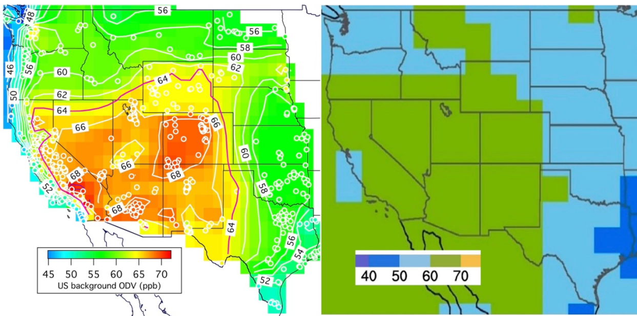
1050 Figure 10: Two estimates of the spatial variability of US background ODVs over the western US. (Left) Contour map of estimated US background ODV for year 2000. The US background ODV excludes estimated wildfire contributions. The 64 ppb contour is colored violet to indicate the extensive area of largest values. Symbols in the contour map indicate individual monitoring sites included in the analysis with the same color coding as the contour map. Results from Parrish et al. (2017; 2022) and estimates for California’s Central Valley (Faloona et al., manuscript in preparation) are included. (Right) Annual 4th highest MDA8 ozone concentration averaged over 2010–2014, from a GFDL-AM3 model simulation with North American anthropogenic emissions zeroed out (figure reproduced from a section of Figure 3 of Jaffe et al., 2018).
