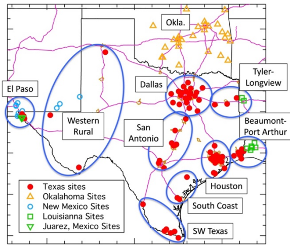
1030 Figure 7: Map of monitoring sites within the Texas region; the symbols are color-coded according to state as indicated in the annotation. Lines indicate outlines of southwestern US states (black), urban areas (gold) and interstates (violet). Nine Texas regions, whose sites are analyzed together as separate data sets, are indicated.
