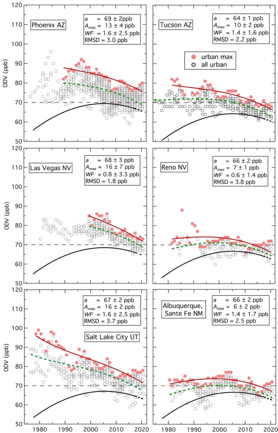
1025 Figure 6: Time series of ODVs recorded in six southwestern US urban areas shown in Figure 4. Open symbols indicate all ODVs recorded in each area, and the solid symbols indicate the maximum ODVs in each year in each area. As in Figure 5 green dashed curves indicate fits of Equation 3 to all ODVs; red solid curves indicate fits of Equation 4 to the maximum ODVs, with the parameters derived in this fit annotated. The black solid curves with dashed extensions indicate the fit to the baseline data from Figure 1, normalized to the respective a parameter values. The light dashed lines indicate the 70 ppb ozone NAAQS.
