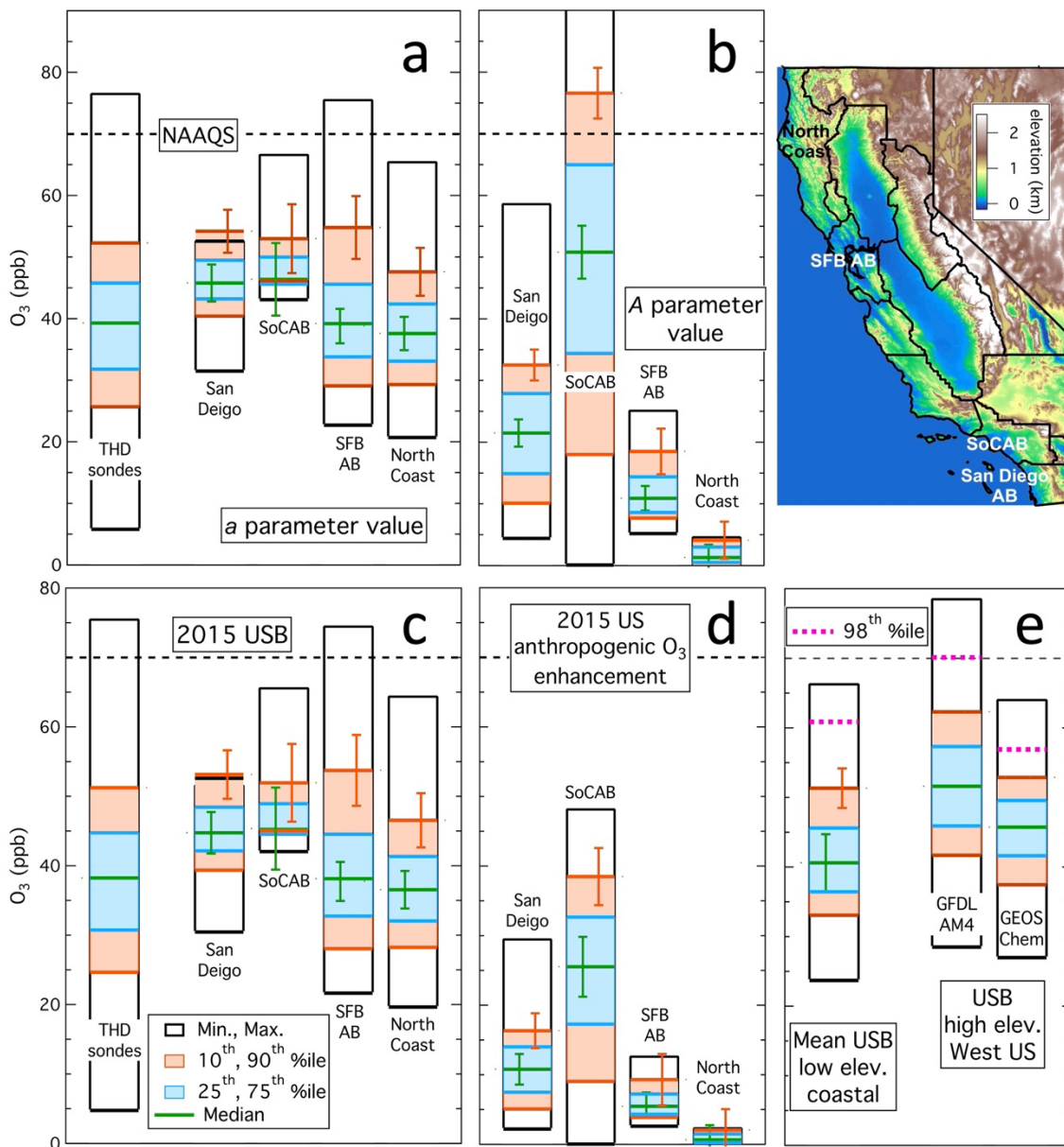
Figure 3. Comparisons of estimates of MDA8 ozone component distributions in 4 coastal California air basins; the inset map identifies the 4 air basins, with the black lines indicating air basin boundaries. (a) Comparison of ozone concentrations measured between 0.6 and 1 km altitude by sondes launched from Trinidad Head from May through September, 1997-2017 and derived a parameter values. (b) Comparison of derived A parameter values. (c) Comparison of the same sonde ozone measurements and year 2015 USB distribution. (d) Comparison of year 2015 distributions of US anthropogenic enhancements. (e) Comparison of the mean of the five, year 2015 USB distributions illustrated in (c) with the distributions of daily MDA8 USB for April–June 2017 at western US high-elevation sites simulated by two global models; these latter bar graphs were derived from Figure 17 of Zhang et al. (2020). Error bars on the median and 90 th percentile lines indicate estimated uncertainties of the determination of the USB and the US anthropogenic ozone enhancement percentiles, and the standard deviations of the means from the five USB determinations.
