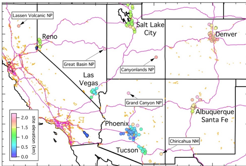
1010 Figure 4: Map of southwestern US urban monitoring sites; the symbols are color-coded according to site elevation as indicated in the annotation. Lines indicate outlines of southwestern US states (black), urban areas (gold) and interstates and selected other major highways (violet). Seven urban areas, whose sites are analyzed together as separate data sets, are labelled. Locations of five of the isolated rural CASTNET sites are also included.
