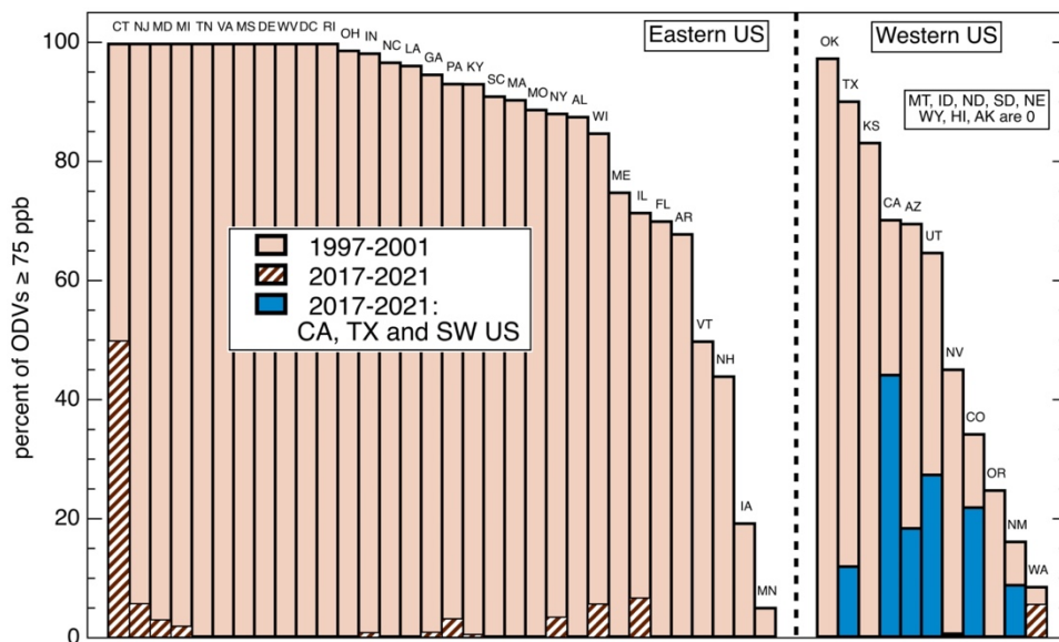
1040 Figure 9: Comparison of percentage of ODVs greater than or equal to 75 ppb recorded at all sites in individual states over two 5-year periods: 2017-2021 (hatched and dark blue bars) and a period 20 years earlier - 1997-2001 (light-colored bars). Individual states are indicated by their two letter abbreviations (defined in Table S6). States are arbitrarily divided between eastern and western regions. Southwestern states, Texas and California are indicated by solid dark blue bars. Eight rural states, all in the western region, reported no ODVs greater than or equal to 75 ppb in either period.
