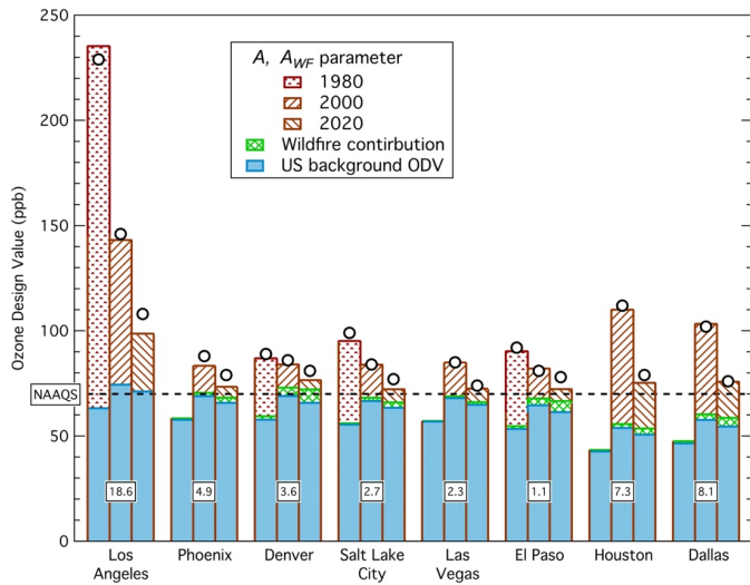
Figure 12: Derived apportionment of maximum ODVs for 3 years at 20-year intervals for the Crestline site in Los Angeles, four southwestern US and three Texas urban areas. The lower, solid blue bars indicate the US background ODV; they exclude estimated wildfire contributions, which are separately indicated by the middle, cross-hatched green bar segments. The top, brown patterned bars indicate the estimated US anthropogenic ODV enhancements, again excluding the wildfire contribution. For four cities the US anthropogenic ODV enhancements and wildfire contributions are missing in 1980 since the tabulated ODVs are inadequate to estimate that parameter that early in the monitoring record. The 2020 populations of the urban areas are annotated in millions. The circles indicate the actual maximum ODVs recorded in the respective years in each area.
