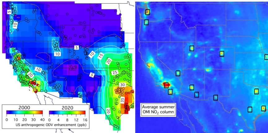
1815 Figure 11: US anthropogenic ODV enhancement over the western US compared to mean summertime OMI NO 2 columns. 1820 (Left) Contour map of estimated US anthropogenic ODV enhancement for year 2000 over the western US. Symbols in the contour map indicate individual monitoring sites included in the analysis with the same color coding as the contour map. A second color scale is included for interpretation of the colors as the year 2020 US anthropogenic ODV enhancement. Results from Parrish et al. (2017; 2022) and estimates for California's Central Valley (Faloona et al., manuscript in preparation) are included. (Right) The OMI NO 2 columns measured in April – September 2005-2014 are reproduced from Figure 1a of Lu et al. (2015) by cropping and changing the aspect ratio of that figure to approximate that of the contour map.
