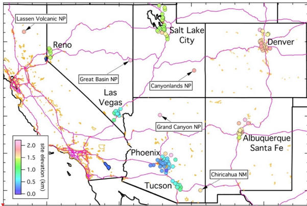
Figure 4: Map of southwestern US urban monitoring sites; the symbols are color-coded according to site elevation as indicated in the annotation. Lines indicate outlines of southwestern US states (black), urban areas (gold) and interstates and selected other major highways (violet). Seven urban areas, whose sites are analyzed together as separate data sets, are labelled. Locations of five of the isolated rural CASTNET sites are also included.
