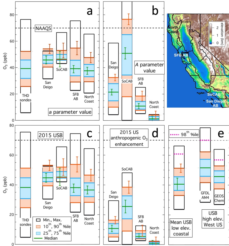
Figure 3. Comparisons of estimates of MDA8 ozone component distributions in 4 coastal California air basins; the inset map identifies the 4 air basins, with the black lines indicating air basin boundaries. (a) Comparison of ozone concentrations measured between 0.6 and 1 km altitude by sondes launched from Trinidad Head from May through September, 1997-2017 and derived a parameter values. (b) Comparison of derived A parameter values. (c) Comparison of the same sonde ozone measurements and year 2015 USB distribution. (d) Comparison of year 2015 distributions of US anthropogenic enhancements. (e) Comparison of the mean of the five, year 2015 USB distributions illustrated in (c) with the distributions of daily MDA8 USB for April–June 2017 at western US high-elevation sites simulated by two global models; these latter bar graphs were derived from Figure 17 of Zhang et al. (2020). Error bars on the median and 90 th percentile lines indicate estimated uncertainties of the determination of the USB and the US anthropogenic ozone enhancement percentiles, and the standard deviations of the means from the five USB determinations.
