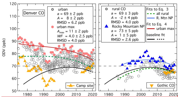
Figure 5: Time series of ODVs recorded in Colorado at the urban sites (left graph) whose locations are shown in Figure 4, and at rural sites (right graph, excluding the Four Corners area) whose locations are shown in Figure S1. Open symbols indicate all ODVs recorded in each area, and solid symbols indicate ODVs from three specific sites and the maximum Denver urban ODVs. As indicated by an annotation on the right graph, green dashed curves indicate fits of Equation 3 to all plotted ODVs (excluding the Camp and Rocky Mountain NP sites, blue curve on right indicates Rocky Mountain NP fit of Equation 3, and red solid curve on left indicates fit of Equation 4 to the maximum Denver urban ODVs; parameters derived in these fits are annotated in the graphs. The black solid curves with dashed extensions indicate the fit to the baseline data included as the grey curve in Figure 1. The light dashed lines indicate the 70 ppb ozone NAAQS.
