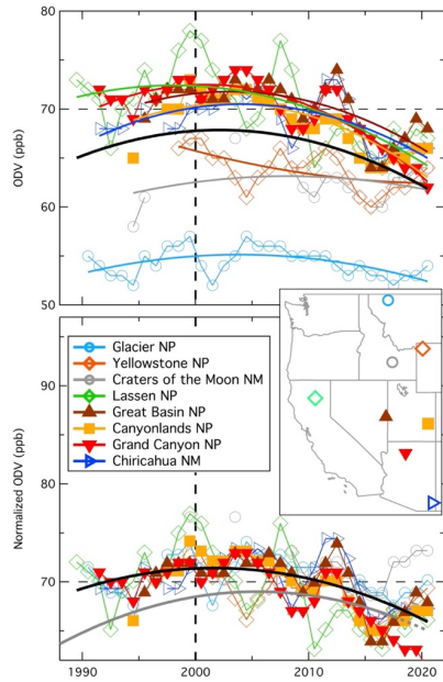
1630 Figure 1: Time series of ODVs recorded at the eight rural western CASTNET sites shown in the inset map. Solid symbols indicate the three sites used for the normalization. Solid curves indicate the fits of Equation 1 to the individual site data (upper panel, including the black curve fit to all data) and to all normalized data (black curve, lower panel). The lower grey curve in the lower panel is the Parrish et al. (2020) fit to baseline data, normalized to 68.5 ppb (the a parameter value derived in a fit of Equation 3 to the normalized CASTNET data) in the year 2000; dashed line shows extrapolation of that fit to 2021.
