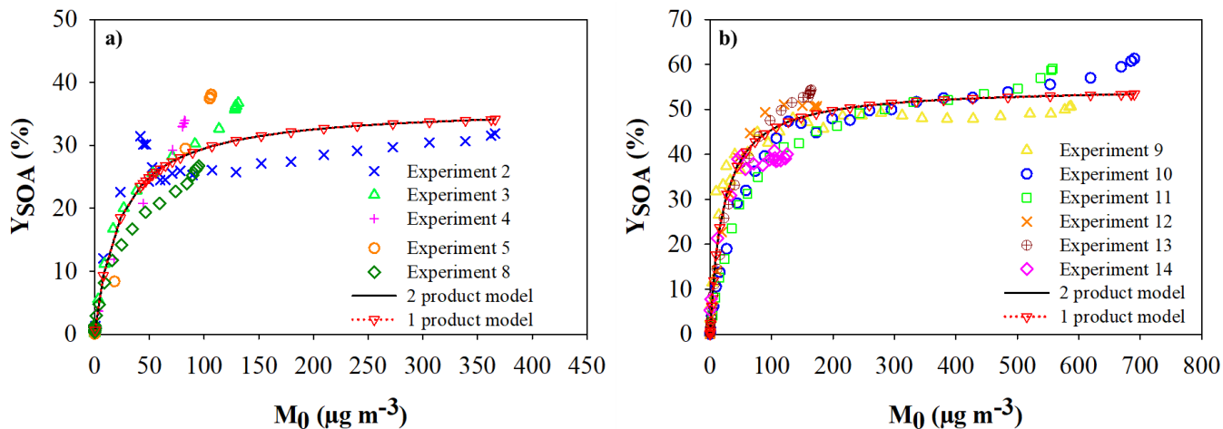
Figure 2: SOA yields as a function of the SOA mass concentration measured for: a) \alpha -phellandrene and b) \beta -phellandrene. Data points from different experiments are shown with different colors and Odum parametrization corresponds to the black solid curves (Eq. 4).
