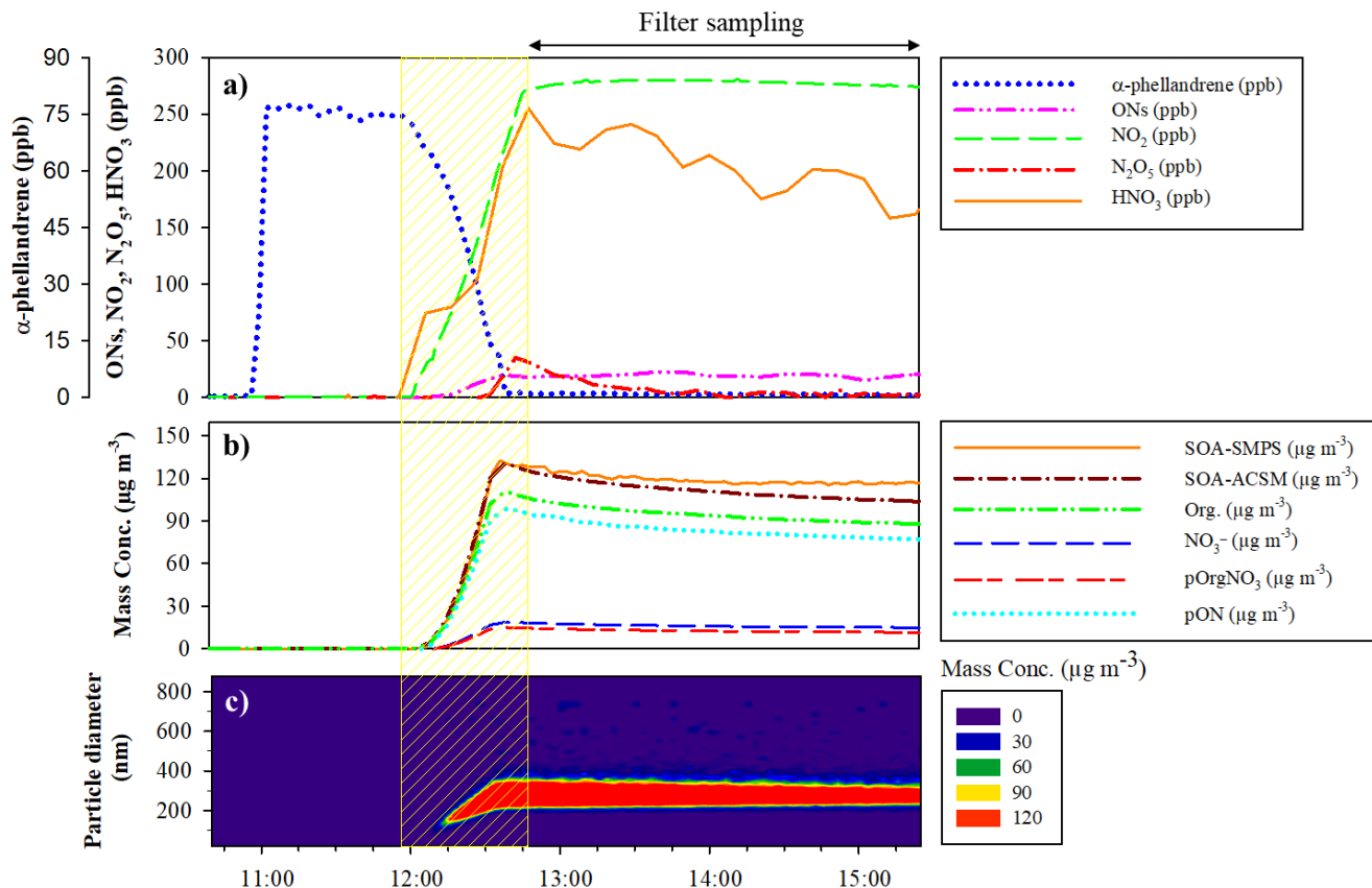
Figure 1: Time series of reactants and products during a typical experiment of \text{NO}_3 -initiated oxidation of \alpha -phellandrene (Experiment 7). (a) Gaseous species mixing ratios, (b) Aerosol mass concentration and chemical composition (with Org. is the total mass concentration of organics, \text{NO}_3^- is the total nitrate functionality mass concentration, pOrg \text{NO}_3 is the mass concentration of the nitrate group within particulate organic nitrates-pON), and (c) Aerosol size distribution and mass concentration. All plots are corrected from dilution. The \text{N}_2\text{O}_5 injection period is shown by the yellow hatched area.
