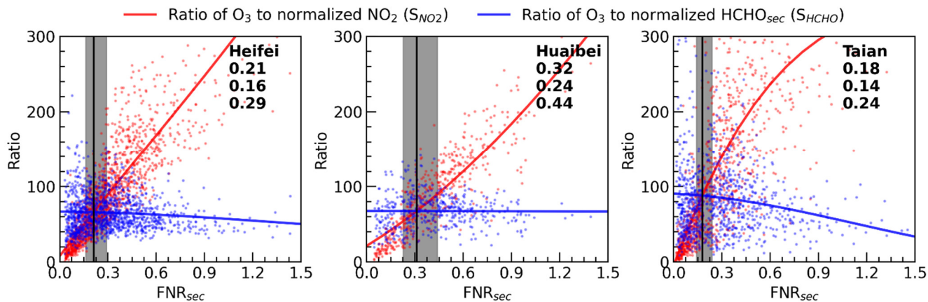
Fig.7. Three-order fitting of ratios of O 3 VMRs versus normalized NO 2 VMRs and ratios of O 3 VMRs versus normalized secondary HCHO VMRs in different FNR sec values in Hefei, Huaibei, and Tai'an during May–September based on MAX–DOAS observations. The intersect at FNR sec indicated by the black solid line. The vertical shadow indicates the relative difference between the ratios of O 3 VMRs versus normalized NO 2 VMRs and ratios of O 3 VMRs versus secondary HCHO VMRs within 25% (transition regime). The labels at the top right of each panel represent the intersect FNR sec values and the thresholds for the NO x –limited regime (high) and VOC–limited regime (low) in Hefei, Huaibei, and Tai'an, respectively.
