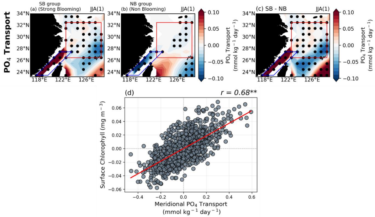
Figure 6. (a-c) Composite maps exhibiting meridional PO 4 transport anomalies during the El Niño decaying summer season for both groups, as well as the difference between the two groups. (d) The relationship between area-averaged meridional PO 4 transport and SCHL anomalies over the target region. All figures show the GFDL-CM2.1 model results.
