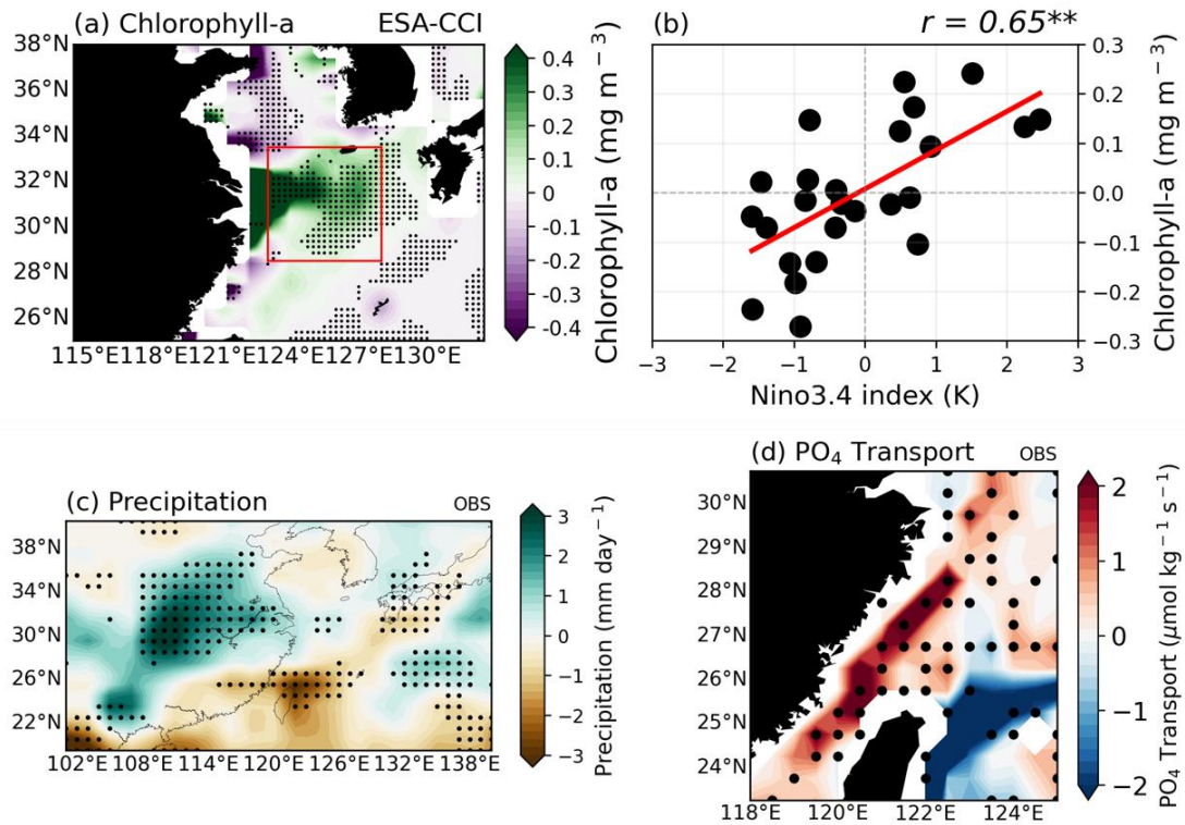
Figure 1. Composite maps exhibiting the 3-month average of (a) surface Chlorophyll-a (SCHL) anomalies using satellite data during the El Niño decaying summer season. (b) The relationship between the Niño3.4-DJF index which indicates the strength of El Niño mature phase and area-averaged SCHL anomalies over the research target area during the El Niño decaying summer season (Red box in Fig. 1a; 28.5°N-33.5°N / 123°E-128°E). (c) Precipitation anomalies for El Niño decaying summer season (June-July-August; JJA) of all El Niño cases, using re-analysis and satellite data. (d) Meridional PO 4 transport anomalies through the Taiwan Strait (TS) for El Niño decaying summer season of all El Niño cases in reanalysis. All the black dots indicate where the responses are significant at the 90% confidence level by using the bootstrap method. ** marks indicate statistically significant correlation at the 99% confidence level.
