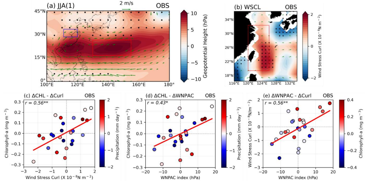
Figure 10. (a) The composite map exhibits the GPH anomalies over the WNP and 850hPa wind anomaly patterns during the El Niño decaying summer season for the available period of re-analysis data (1979-2022; 44 years). Red and blue boxes indicate the area-averaged WNPAC index (16.5°N-26.5°N, 130°E-155°E) and precipitation index (28.5°N-33.5°N, 111°E-120°E) respectively. Black dots indicate the insignificance at the 90% confidence level using the bootstrap method. (b) The composite map shows WSCL anomaly patterns and 850hPa wind anomaly patterns during the El Niño decaying summer season within the same period with Fig. 10a. The red box indicates the area-averaged WSCL index. Black dots indicate the significance at the 90% confidence level using the bootstrap method. (c-d) The relationship between SCHL anomalies in the target region and the WSCL index and the WNPAC index respectively. Colored scatters show the precipitation index over the eastern part of China. (e) The relationship between the WNPAC index and the WSCL index. Colored scatters show the magnitude of SCHL anomalies in the target region.
