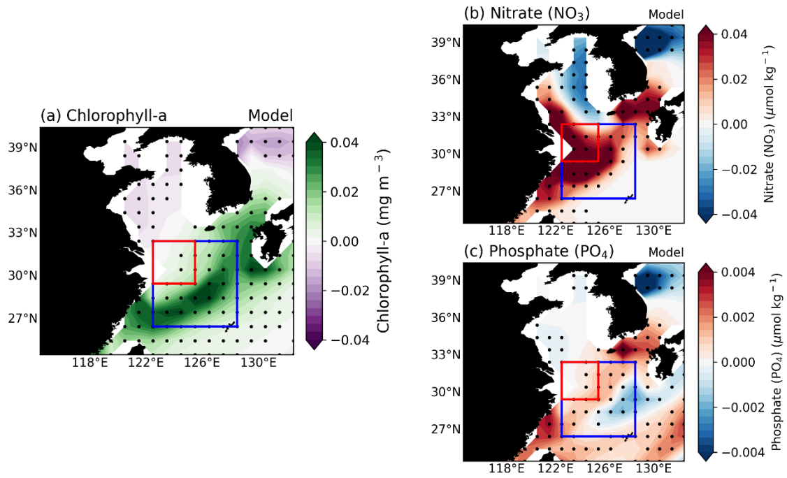
Figure 3. (a-c) Composite maps illustrate the SCHL, surface \text{NO}_3 , and surface \text{PO}_4 distribution of El Niño decaying summer season over the East China Sea (ECS) for all El Niño cases (176 years) which were selected in GFDL-CM2.1 ESM results. All the black dots indicate where the responses are statistically significant at the 95% confidence level, determined using the bootstrap method.
