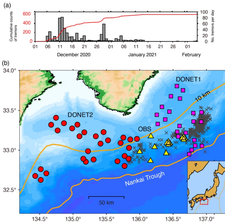
85 Figure 1: (a) Frequency of tremors that occurred between December 1, 2020, and February 5, 2021, with the cumulative numbers by the solid line and counts per day by the histogram. The tremors are the same as those used in the panel (b). (b) Map showing the locations of stations. Squares and circles represent DONET1 and DONET2 stations, respectively, and triangles show temporary OBSs. The two lines correspond to the Nankai Trough and the contour lines of 10 km for the Philippine Sea Plate (Baba et al. 2002; Hirose et al. 2008). Crosses indicate the locations of tremors that occurred between December 1st 2020 and February 5th, 2021 90 (Tamaribuchi et al. 2022), for which tremors with spatial errors \leq 0.1^\circ are plotted and 16% of tremors are preserved from the original catalog.
