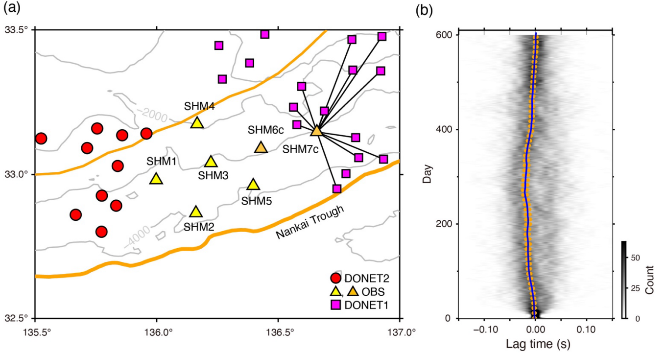
Figure 3: Clock deviations at SHM7c. (a) The locations of the pairs between SHM7c and DONET stations used for measuring the clock deviations, which are connected by solid lines. (b) The estimated clock deviations at SHM7c. The solid and dashed lines represent the weighted average and its standard deviations for the clock deviation. The background counts indicate the measurements of the clock deviations counted at bins of 0.01 s and 1 day.
