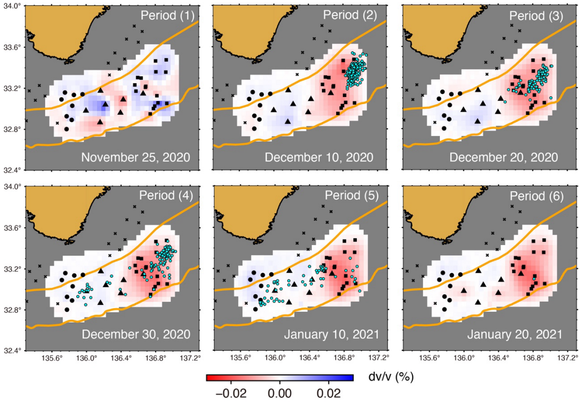
260 Figure 5: Spatio-temporal dv/v variations in Periods (1–6). Circles represent the tremor locations within \pm 5 days from the reference dates, as determined by Tamaribuchi et al. (2022), from which tremors with spatial errors \leq 0.1^\circ are plotted (16% of tremors from the original catalog). Squares and circles indicate the DONET1 and DONET2 stations, and triangles show temporary OBSs used in this analysis (KMB, KMC, KMD, MRD, MRE and temporary OBSs). Crosses represent the other stations.
