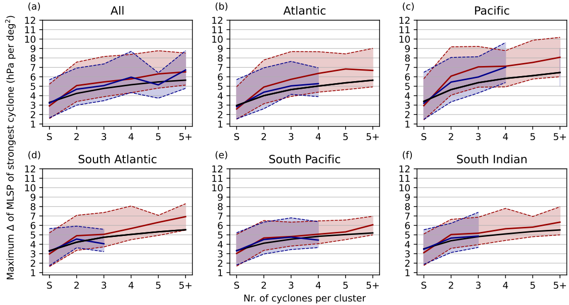
Figure 8. As Figure 7 but for Bjerknæs-sequential type (red solid line and shading, for mean and 10 to 90 % quantiles) and stagnant type (blue shading). Black line indicates expected value from randomly chosen clusters.
