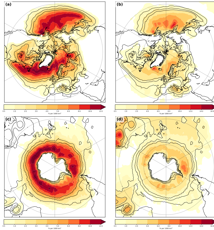
Figure 3. Densities for (left) Bjerknes-sequential type and (right) stagnant type cyclone clusters for (top) Northern Hemisphere and (bottom) Southern Hemisphere for the respective winter season. Shading denotes fraction of times of a clustered cyclone at a location in a 1000 km 2 area. Black contours indicate clustered densities (at 2, 4 & 6 % per 1000km 2 )
