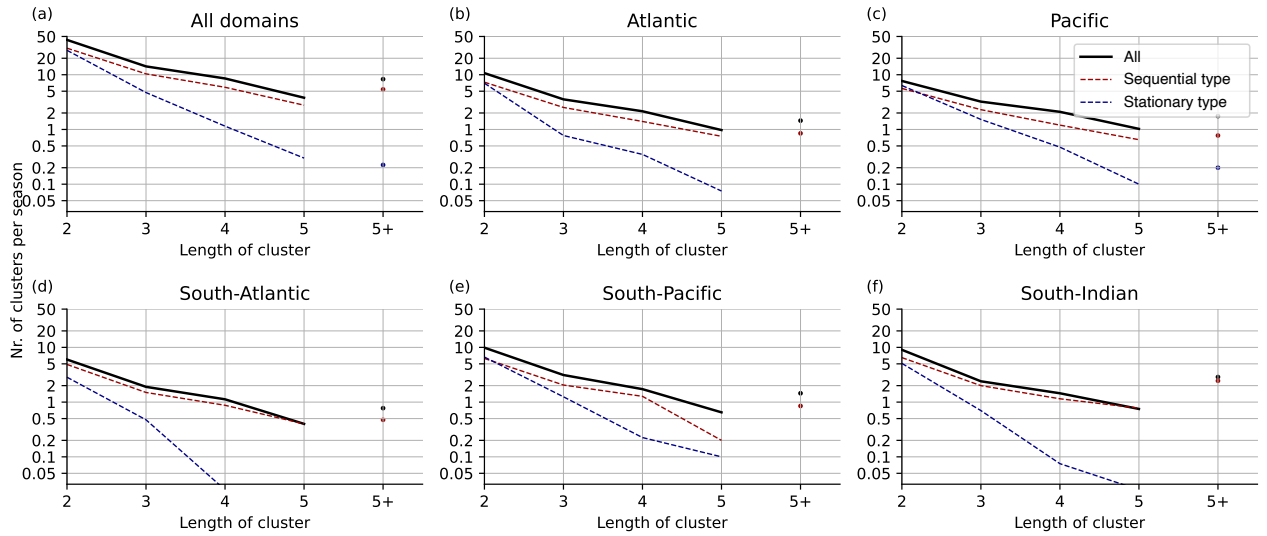
Figure 6. Number of clusters for the respective winter season as function of size of cluster for all clusters (black line), Bjerknes-sequential type (red line), and stagnant type (blue line). (a) Top left for all regions. (b-f) For Atlantic, Pacific, South Atlantic, South Pacific, and South Indian Ocean, respectively.
