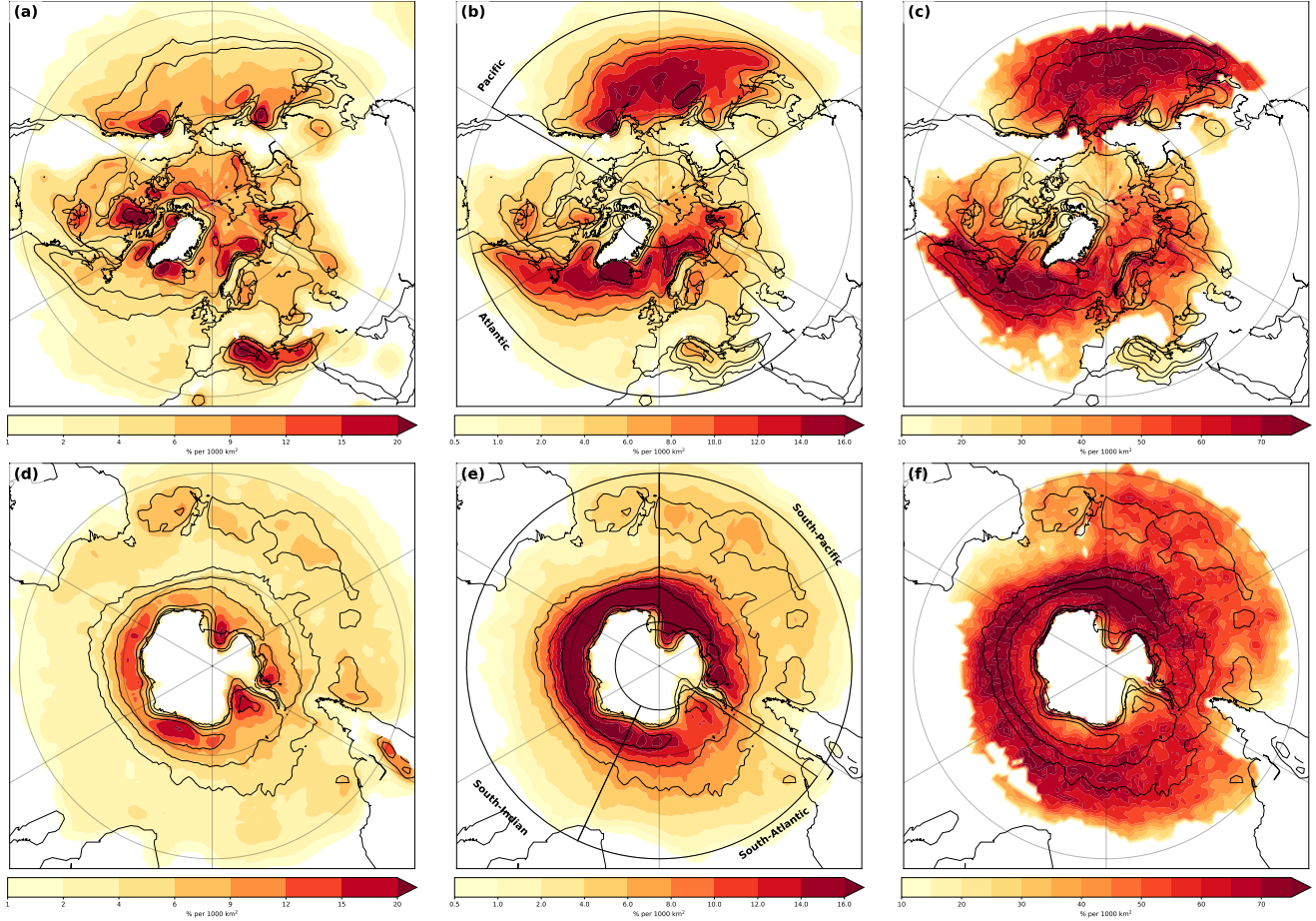
Figure 2. Cyclone densities defined as the fraction of time steps with a cyclone occurring per unit area of 1000 km 2 area. (a) Density of solo cyclones (not clustered) for DJF in the Northern Hemisphere. (b) and (c) as (a), but for clustered cyclones and Fractional density of clustered cyclones, respectively (shading). (d-f) as (a-c), but for JJA in the Southern Hemisphere. Black boxes in (b) and (e) indicate chosen regions in section 4, and black contours in each panel indicate climatological storm tracks of all cyclones (contours at 10, 15 & 25 % per 1000km 2 ).
