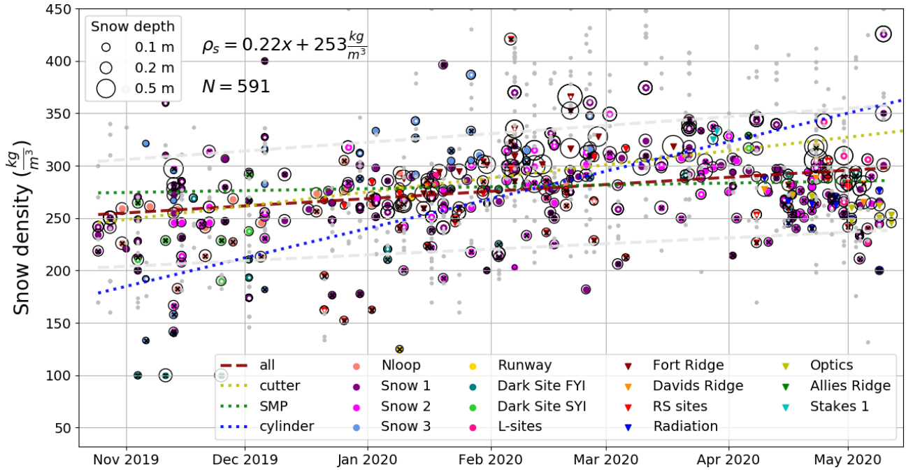
Figure 6. Bulk snow density from density cutters (N=243), SnowMicropenetrometer (SMP, N=182), and SWE cylinder (N=166), during the pre-melt period from MOSAiC snow pits. The red dashed line is a linear fit to all the data and grey dashed lines are the limits of lower and upper 20% values typical for depth hoar and wind slab. The yellow, blue, and green lines represent best linear fits for individual measurement subsets. Estimates from the SWE cylinder are identified using a black cross. Estimates from cutters have a white dot. Individual cutter values are displayed as small grey dots.
