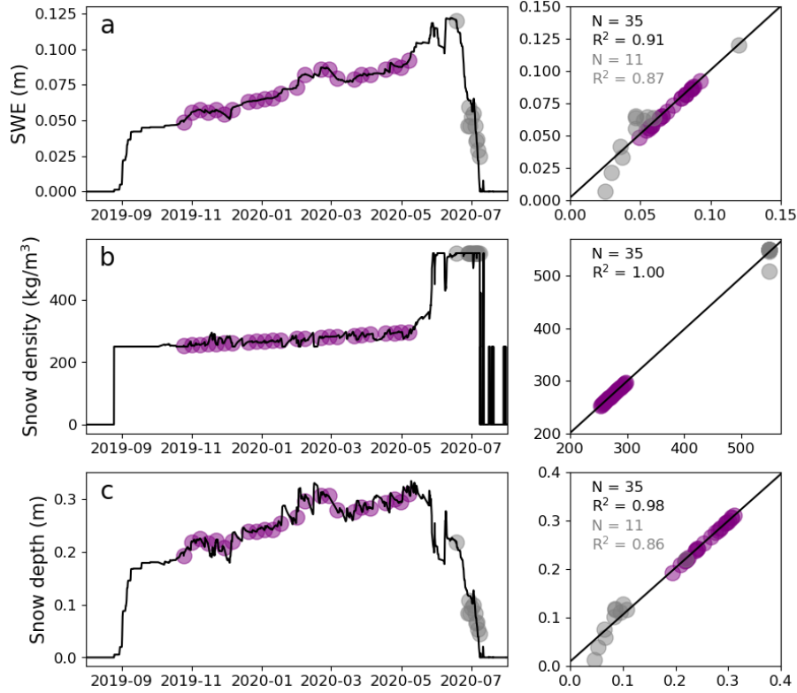
Figure 7. Nloop SnowModel-LG snow assimilation time series and scatter plots (x-axis for observations and y-axis for model) for a) SWE, b) bulk snow density, and c) snow depth in each of the figure rows. Assimilated observed values are represented by purple circles. Not assimilated observed values (melt period) are represented by grey circles. In the right column correlations for all data are printed in black and correlations for the melt period are written in grey. All correlations are significant.
