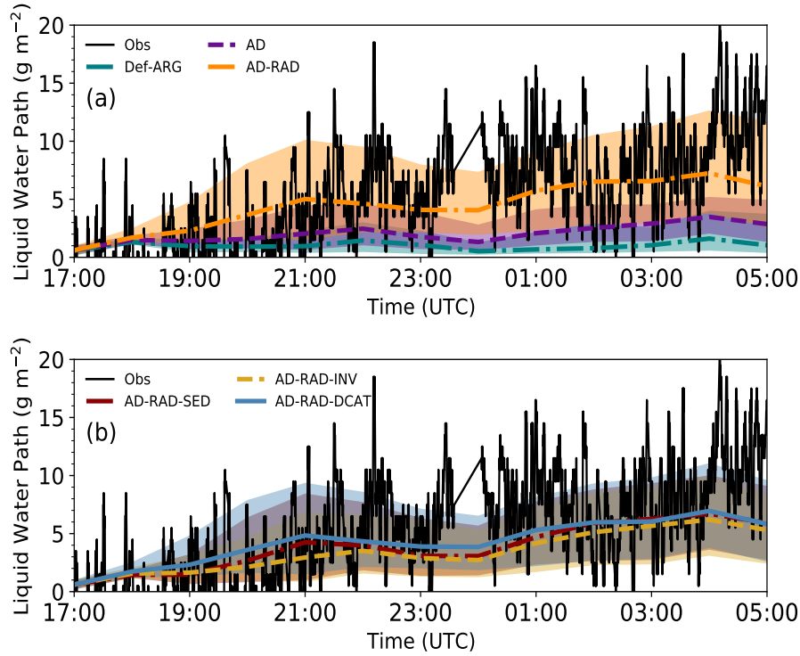
Figure 9. Time series of liquid water path during the LANFEX case study for different simulations. Top Panel: Def-ARG, AD and AD-RAD. Bottom Panel: AD-RAD-SED, AD-RAD-INV and AD-RAD-DCAT.
