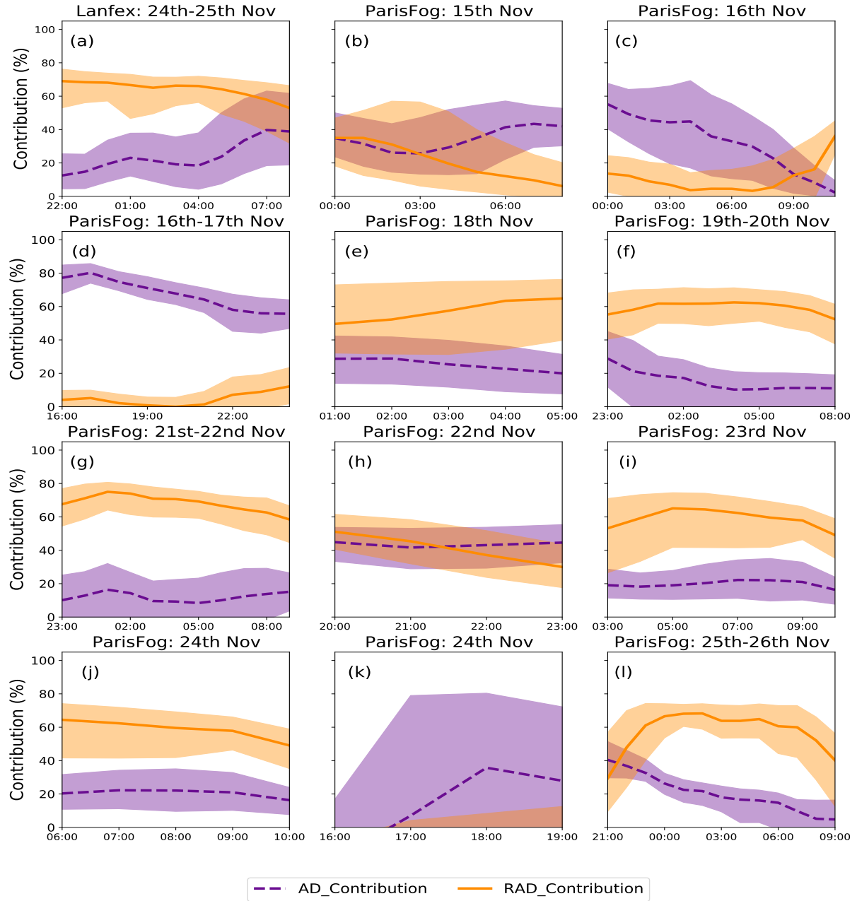
Figure 14. Timeseries (UTC) of the percentage contribution to droplet activation (at the surface) from radiative and adiabatic cooling, as simulated by our 500 m model across various fog cases during LANFEX (subplot a) and ParisFog (subplot b-l) campaigns. The dashed purple line represents the median fraction of droplets originating from adiabatic cooling, while the solid orange line represents those originating from radiative cooling. Shaded regions illustrate the interquartile ranges of these contributions. The AD-RAD simulation is compared with the simulations AD and RAD to generate this figure.
