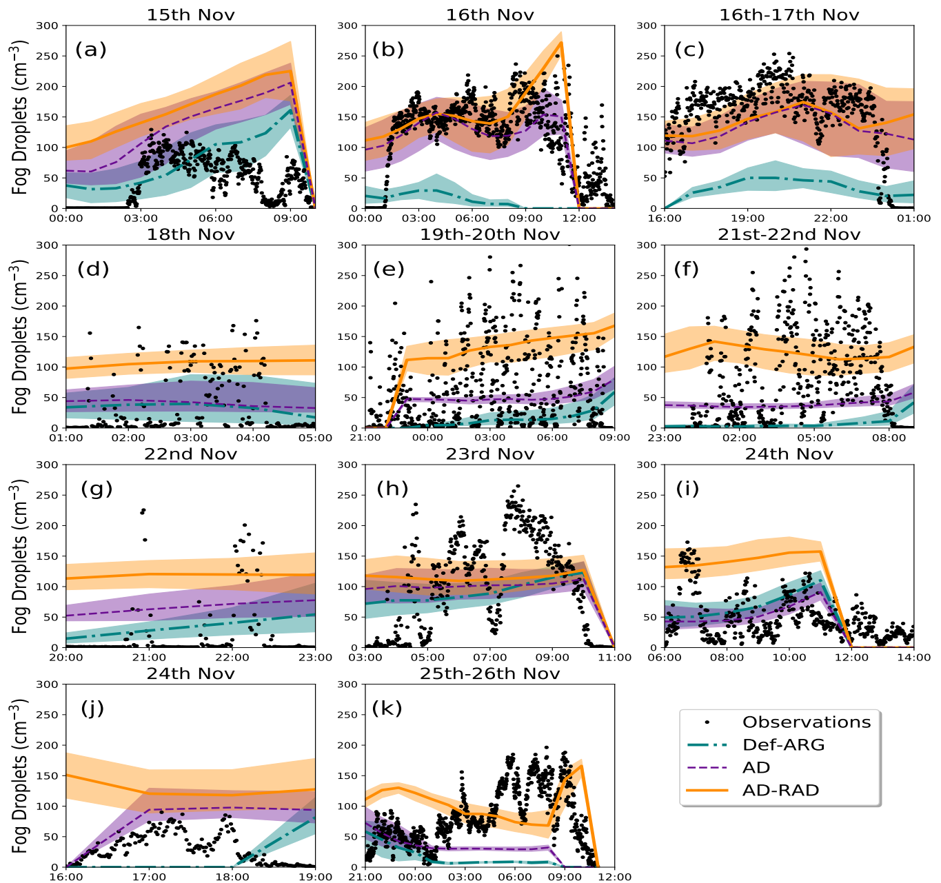
Figure 6. Variation of simulated and observed fog droplet number concentrations as a function of time for different fog events. The results of the 500 m model at 5 m altitude from the simulations Def-ARG, AD, and AD-RAD are compared with observations at the SIRTA observatory (UTC time). Lines represent the median value and the shaded regions represent the interquartile range over the foggy gridboxes.
