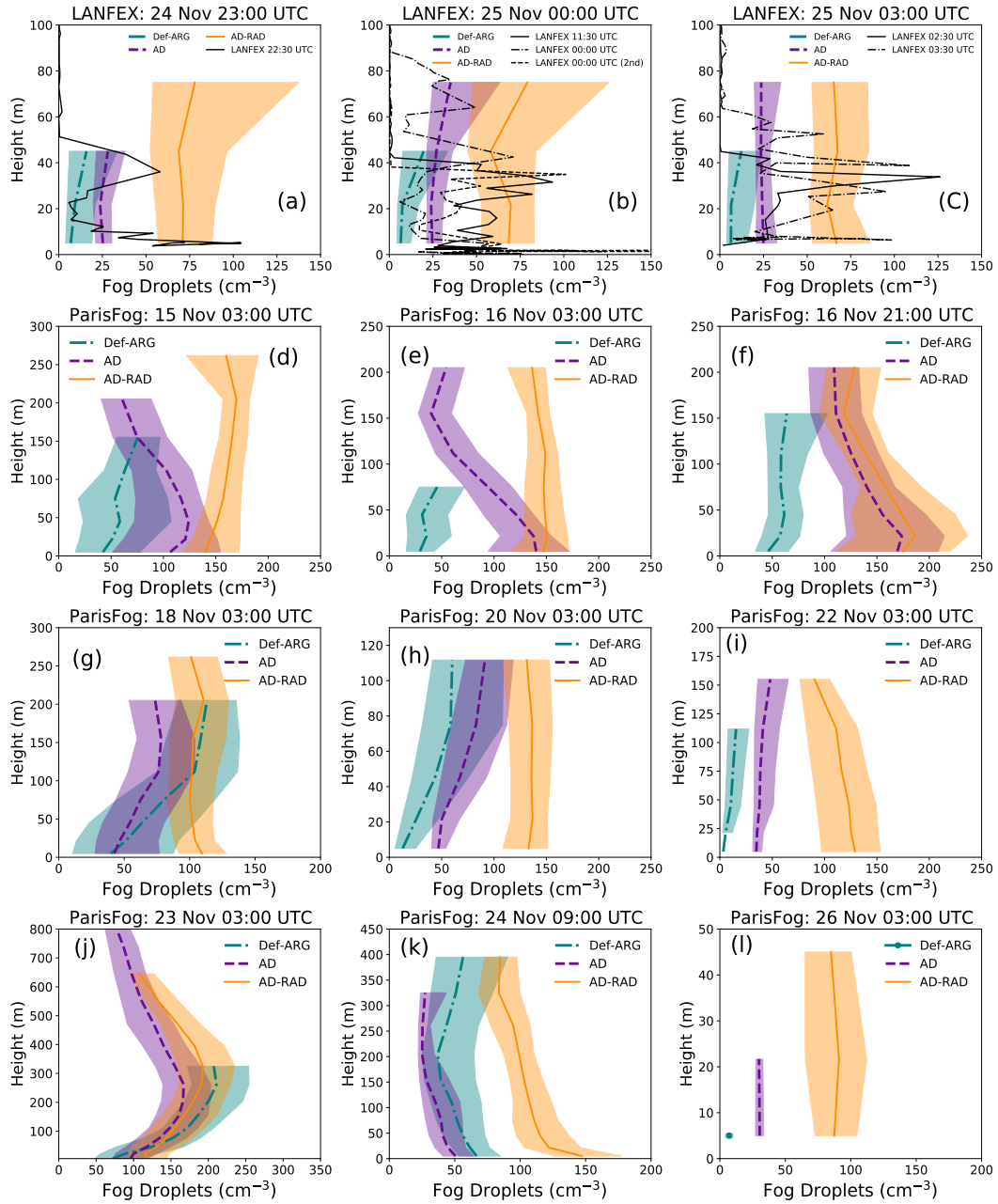
Figure 10. Vertical Profiles of N_d from the LANFEX case study and different days of the ParisFog case study. The results of the 500 m model for Def-ARG, AD, and AD-RAD simulations are shown. Observations during LANFEX are from the fog monitor on the tethered balloon. Note the different y axis scales of the different subfigures, reflecting the substantial variability in fog top height between fog cases.
