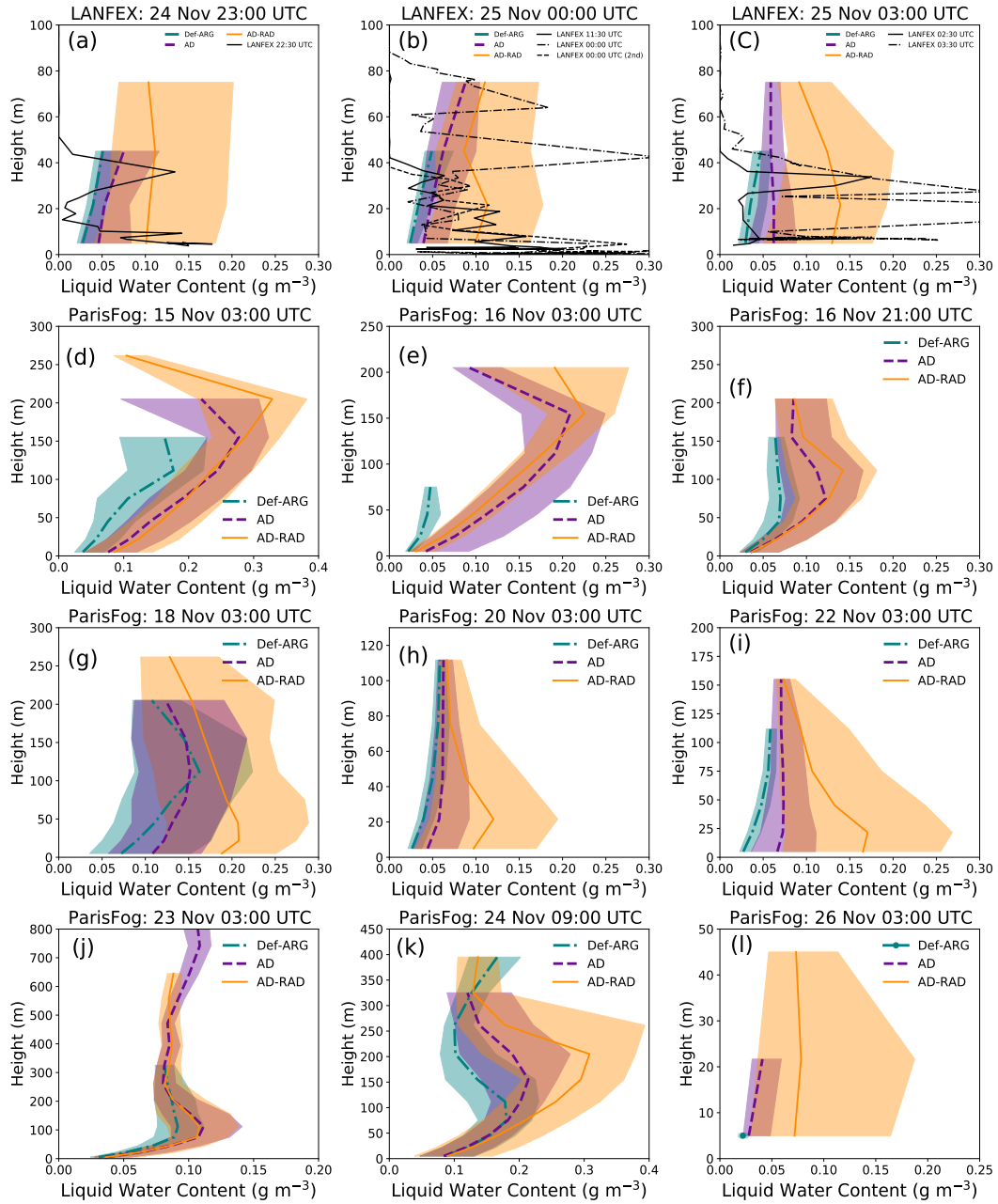
Figure 11. Vertical Profiles of LWC from the LANFEX case study and different days of the ParisFog case study. The results of the 500 m model for Def-ARG, AD, and AD-RAD simulations are shown here. Observations during LANFEX are from the fog monitor on the tethered balloon. Note the different y axis scales of the different subfigures, reflecting the substantial variability in fog top height between fog cases.
