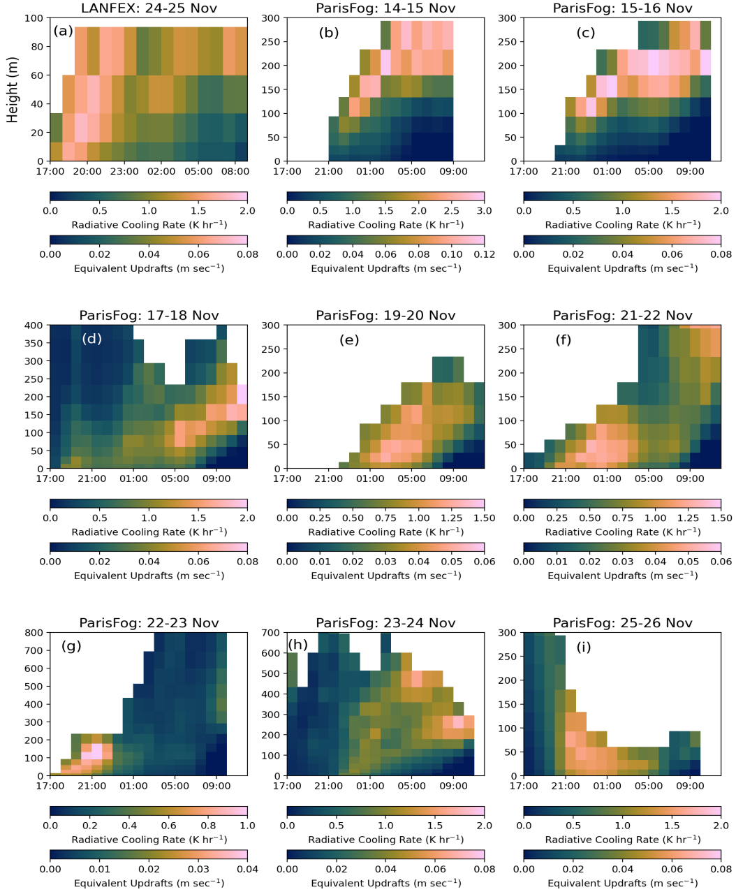
Figure 12. Vertical profile of radiative cooling rate in our 500 m AD-RAD simulation, as a function of time (UTC). Subfigure (a) represent the fog event from the LANFEX case, and subfigures (b)-(i) represent two events from the different ParisFog cases. The median cooling rates of all foggy gridboxes (at the surface and their vertical column following the algorithm described earlier ) are taken plotted. Equivalent updrafts (assuming a 6.5 \text{ K km}^{-1} temperature lapse rate) are also shown in the additional colorbar.
