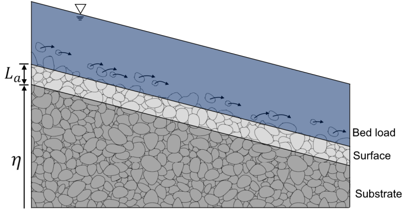
470 Figure 5: Schematic diagram of the model's three layers, used to represent the evolution of the surface and substrate grain size distribution.
