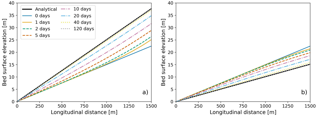
Figure 7: Changes in bed surface elevation for a case of a) pure aggradation and b) pure degradation. The analytical solution corresponds to the equilibrium slope given by Eq. 33. The small differences in bed elevation after 40 and 120 days indicate that the systems achieved an equilibrium state.
