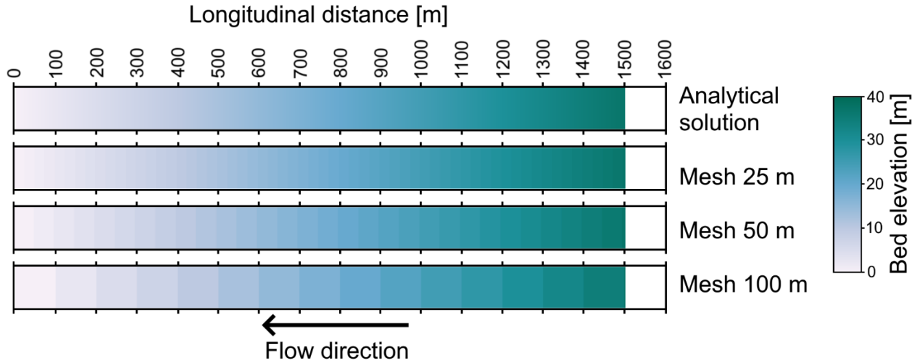
Figure 8: Sensitivity of the predicted bed elevations to the grid resolution after 120 days of simulation. Three different meshes were used and compared to the analytical solution.
