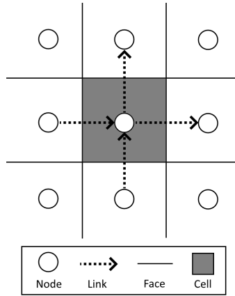
Figure 1: Elements of a Landlab grid used by our component, illustrating a typical grid segment. Information is stored in nodes and links. For instance, surface bed elevation data is held at the nodes, whereas the gradients of these elevations are stored in the links.
