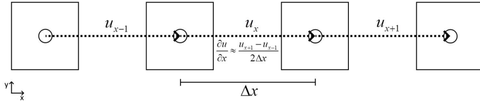
Figure 3: A representation of the stencil used to calculate the velocity gradient at links. Cells are separated only to highlight the definition of velocities at links. The gradient \partial u/\partial x at the location of the link with velocity u_x is estimated using a central difference scheme and considers the neighboring links. The same principle applies to calculate \partial v/\partial y but is not represented in this figure.
