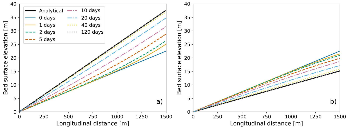
590 Figure 7: Changes in bed surface elevation for a case of a) pure aggradation and b) pure degradation. The analytical solution corresponds to the equilibrium slope given by Eq. 33. The small differences in bed elevation after 40 and 120 days indicate that the systems achieved an equilibrium state.
