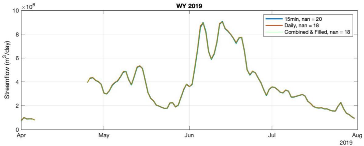
35 Figure S2. Time series of streamflow observations at the TGC gauge for April-July 2019. The blue line tracks the daily-aggregated 15-min data; the orange line tracks the daily data downloaded from CDEC; and the green line tracks the post-processed gap-filled time series.
