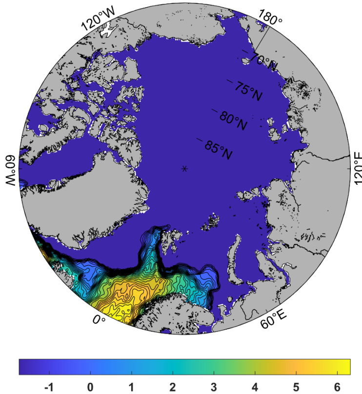
Figure 12: Sea surface temperature ( ^{\circ}\text{C} ) in intervals of 0.3^{\circ}\text{C} at 02:00 UTC on 25 February, 1987, from ERA5 reanalysis. Dark blue areas denote regions of sea ice. From ERA-5 reanalyses.
