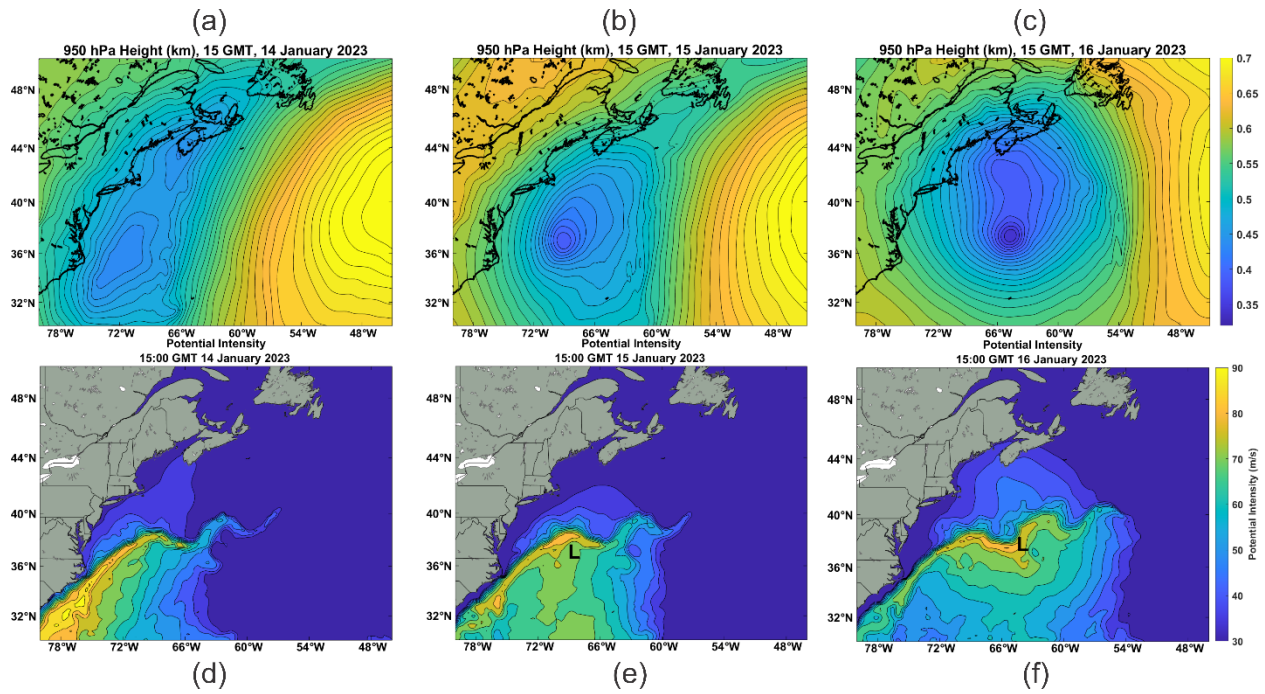
505 Figure 19: The 950 hPa geopotential height (km) at 15:00 UTC on January 14 th (a), 15 th (b), 16 th (c); the V_{pm} field in 506 increments of 5 ms -1 , on January 14 th (d), 15 th (e), and 16 th (f). In (e) and (f) the “L” shows the position of the 950 hPa 507 cyclone center at the time of the chart. From ERA-5 reanalysis.
