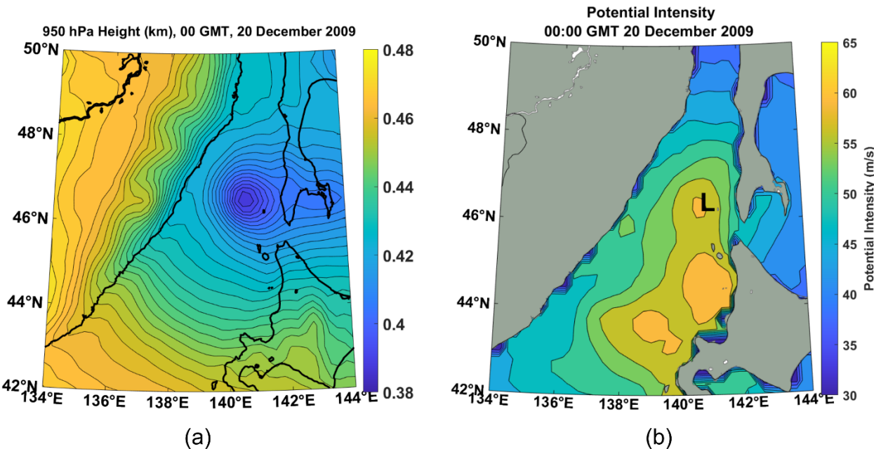
Figure 16: 950 hPa geopotential height (a; km) at intervals of 3 m, and V_{pm} at intervals of 3 m s -1 (b), at 00 UTC on 20 December, 2009. In (b), the “L” marks the satellite-derived surface cyclone center. From ERA-5 reanalysis.
