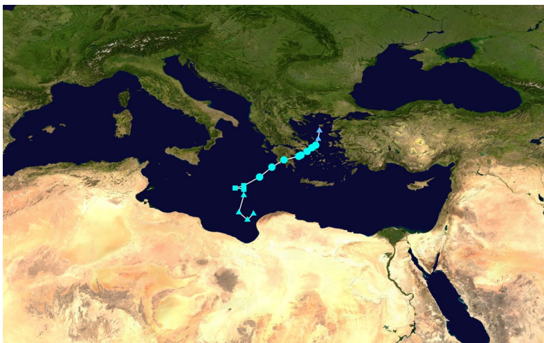
Figure 23: Track of Cyclone Zorbas, from 27 September through 2 October, 2018. (Image credit: Wikipedia Commons; https://commons.wikimedia.org/wiki/File:Zorbas_2018_track.png )
