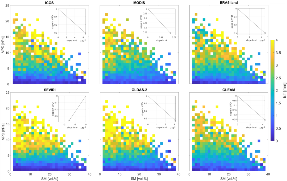
446 447 Figure 10: ET [mm] relative to SMAP SM [vol.%] and in-situ VPD [hPa] for all investigated ET products and averaged over all investigated 448 ICOS stations in 2017. The inset plots provide the corresponding median slope in SM and VPD changes.
