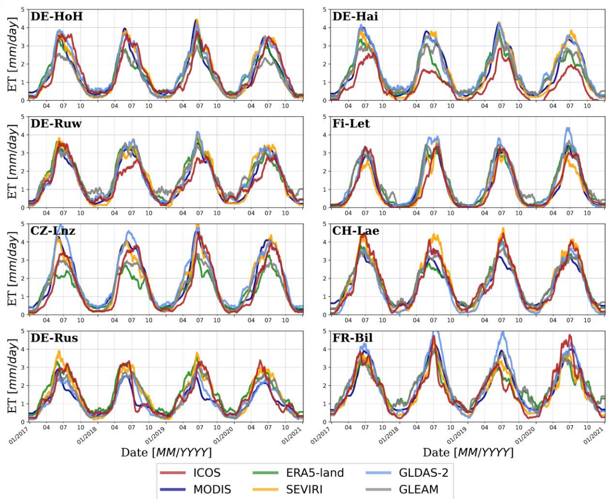
Figure 4: Comparison of seasonal dynamics of ET [mm] products for the period 2017-2020 at investigated ICOS stations. All time series were cleaned for daily and weekly dynamics using a Savitzky-Golay (Savitzky and Golay, 1964) filter with a window size of 31 days.
