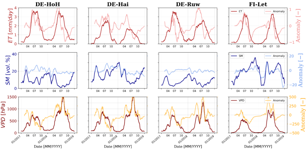
380 Figure 7: Time series of daily ICOS ET [mm/day], SMAP SM [vol.%], and in-situ VPD [hPa] for 2017 and 2018 at DBF (DE-HoH, DE- 381 Hai), and ENF (DE-Ruw, FI-Let) stations compared to their respective anomalies (see Sec. 2.3.2). All time series were cleaned for daily and 382 weekly dynamics using a Savitzky-Golay (Savitzky and Golay, 1964) filter with a window size of 31 days.
