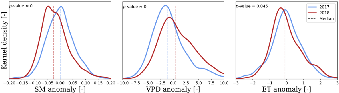
400 401 Figure 8: Kernel density estimates of daily SMAP SM, in-situ VPD, and ICOS ET anomalies (see Sec. 2.3.2) during April to October of 402 2017 and 2018 across all investigated stations. The dashed lines represent the seasonal median of respective parameters and years. The p - 403 values of a two-sided Wilcoxon rank-sum test indicate the acceptance ( > 0.05 ) or rejection ( < 0.05 ) of the null hypothesis regarding 404 continuous distributions with equal medians at the 5 % significance level.
