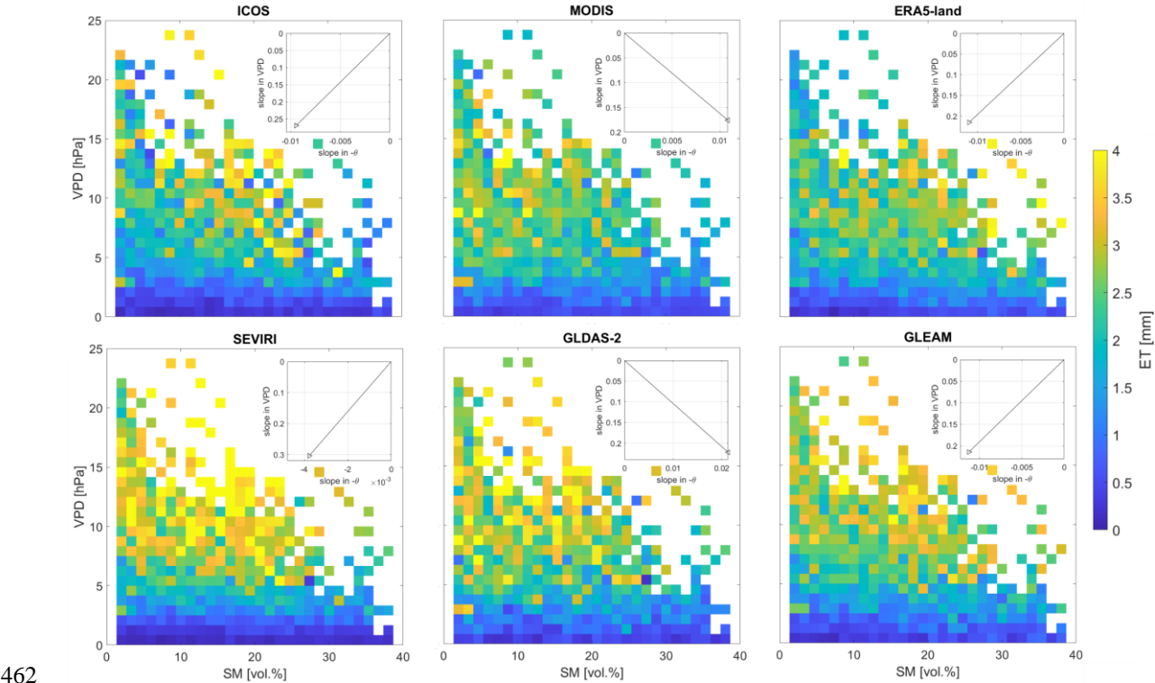
Figure 11: ET [mm] relative to SMAP SM [vol.%] and in-situ VPD [hPa] for all investigated ET products and averaged over all investigated ICOS stations in 2018. The inset plots provide the corresponding median slope in SM and VPD changes.
