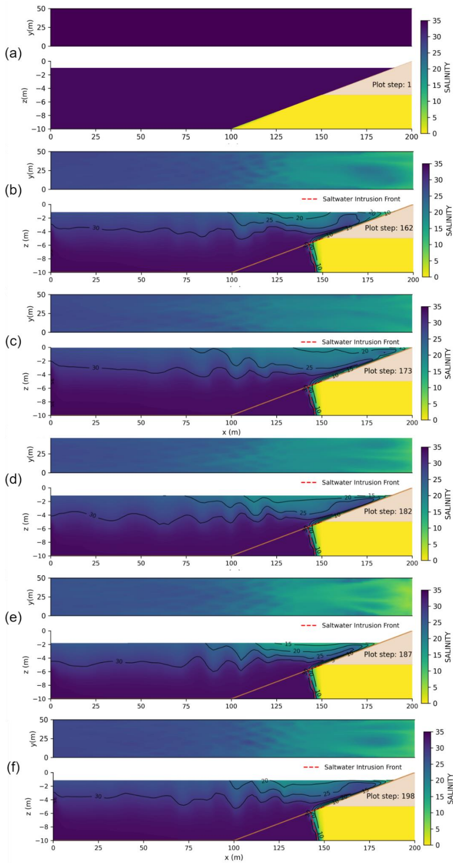
Fig. 5 Coupling model simulation of salinity patterns throughout tidal cycles depicted in top and vertical views (a)Initial moment (b)Tidal Start (c) High Tide (d)Mid-Tide (Flood) (e) Low Tide (f) Mid-Tide (Ebb)
