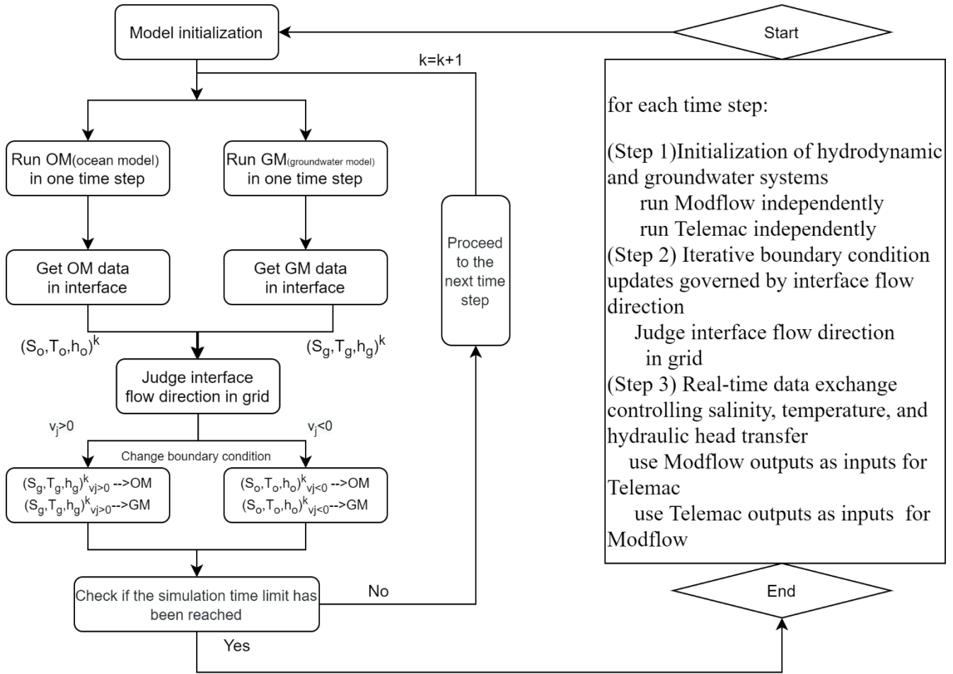
Fig. 1 Flowchart and Pseudo-code Illustrating the Process of Coupled Models
