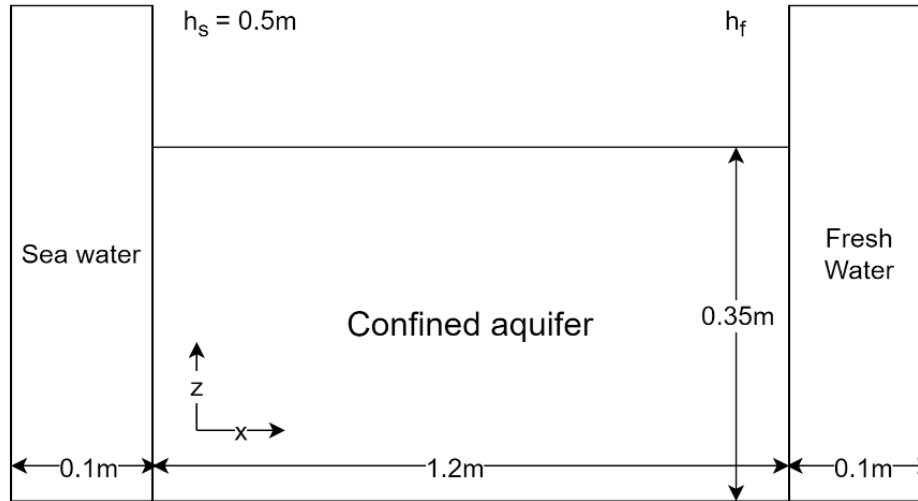
Fig. 2 Schematic of the coupled ocean-groundwater model: Ocean model (TELEMAC-3D) simulating seawater, groundwater model (MODFLOW6) representing a confined aquifer, with no-flow and constant freshwater head boundary conditions.
