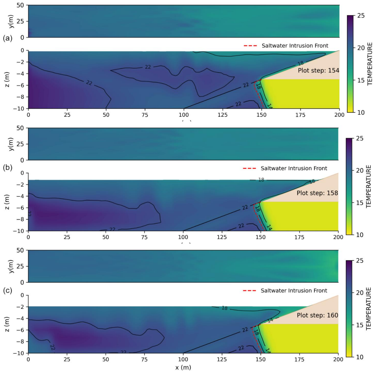
Fig. 6 Temperature patterns throughout tidal cycles depicted in top and vertical views (a) High Tide moment (b) Mid-Tide (Ebb) (c) Low Tide moment
