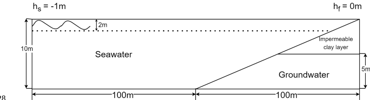
29 Fig. 4 Initial and boundary conditions of the tide numerical model
