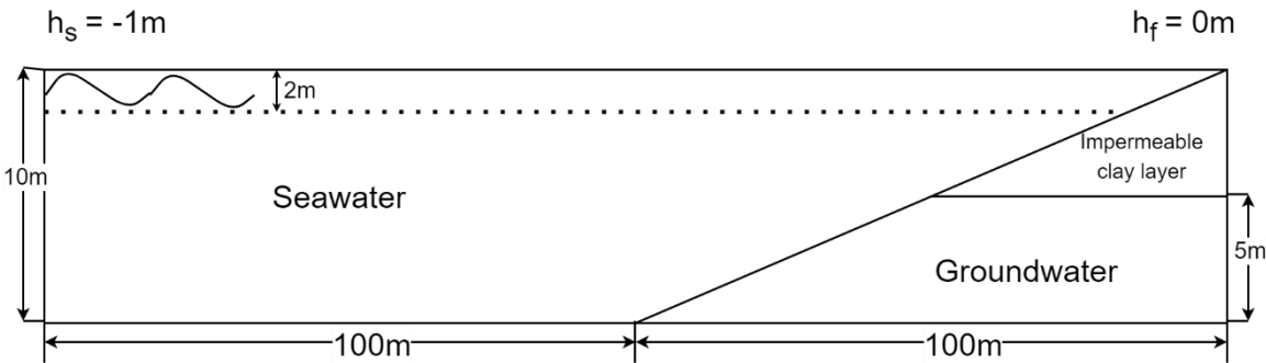
29 Fig. 4 Initial and boundary conditions of the tide numerical model
