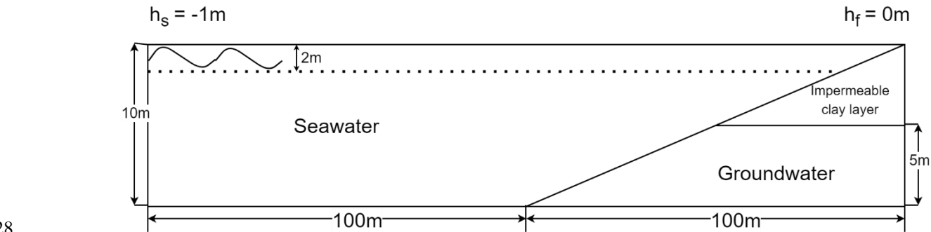
29 Fig. 4 Initial and boundary conditions of the tide numerical model
