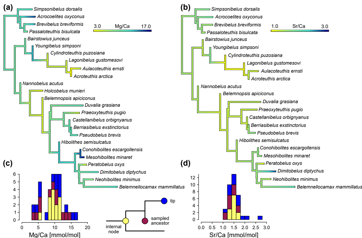
Figure 8. Ancestral state reconstructions of elemental ratios, based on MCC tree. (a) Mg/Ca ratio. (b) Sr/Ca ratio. (c) Histogram of Mg/Ca values, coloured by internal node, sampled ancestor and tip. (d) Histogram of Sr/Ca values, coloured by internal nodes, sampled ancestors and tips. Note that values at tips and sampled ancestors are directly measured, while internal nodes use average values from ancestral state reconstruction.
