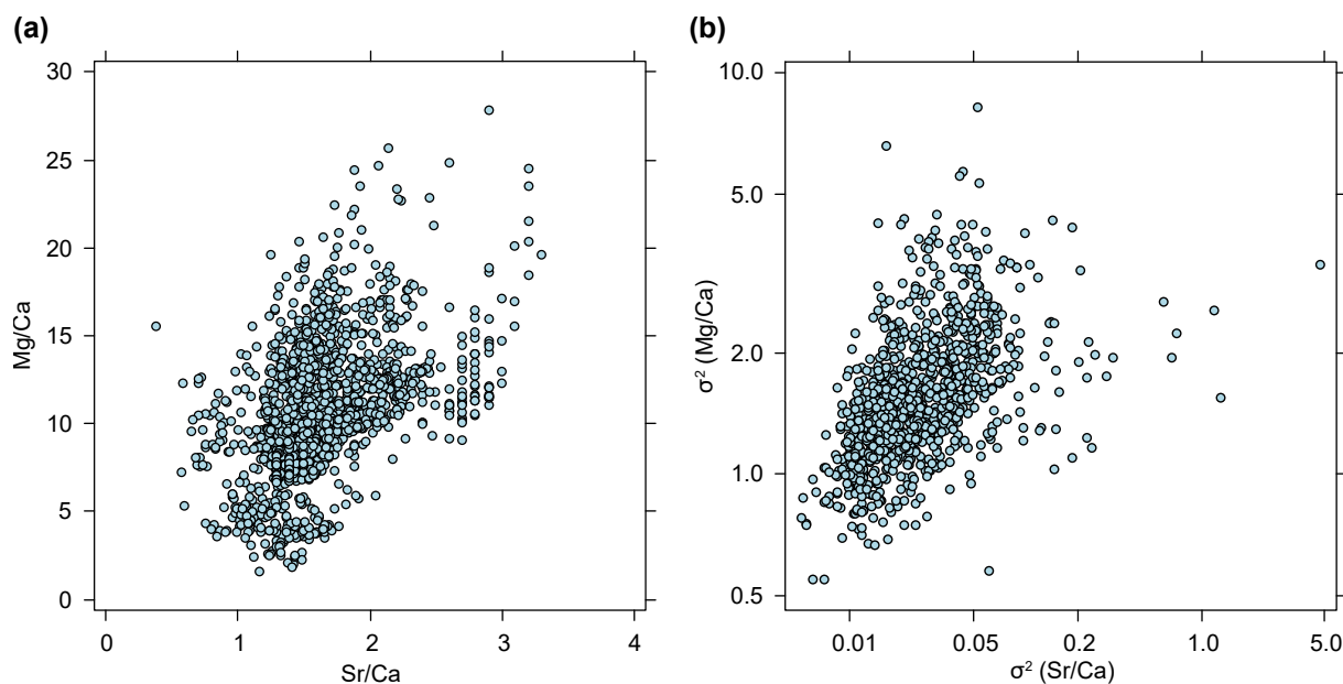
Figure 11. Correlation between element ratios and their evolutionary rates. (a) Element ratios as raw values, taken from entire data set, i.e., each point represents a single measurement from a belemnite rostrum ( n = 2241 ). (b) Evolutionary rates ( \sigma^2 ), taken as means of posterior samples, i.e., each point represents the average evolutionary rate inferred for a single tree ( n = 1000 ). Note that B is shown on a double logarithmic scale.
