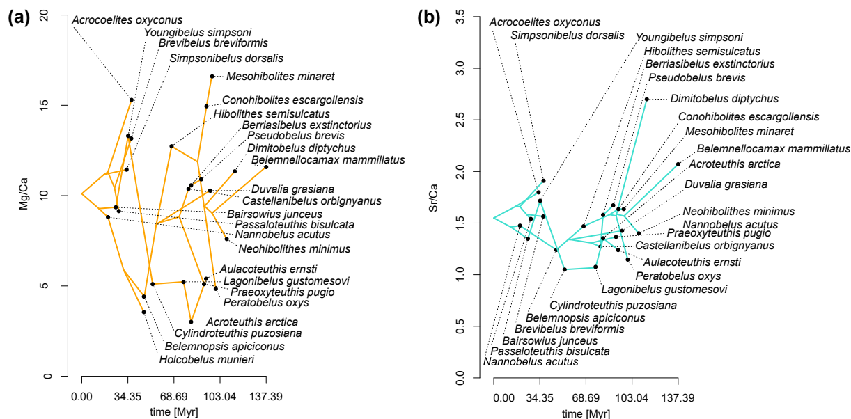
Figure 7. Phenogram of element ratios, plotted to MCC tree. Note that time is represented in million years since the root of the tree, which is set at 216.3 Ma. The youngest taxon in this tree, Belemnellocamax mammillatus , occurs at 78.9 Ma. (a) Mg/Ca ratio. (b) Sr/Ca ratio.
