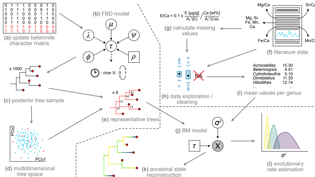
Figure 1. Workflow of the present study. (a) Collecting additional data for character matrix to include taxa for which element ratio data are available. (b) Inference of tree topology ( \tau ) in RevBayes using the fossilised birth-death (FBD) model, consisting of extinction rate ( \mu ), speciation rate ( \lambda ), fossilisation rate ( \psi ), extant sampling rate ( \rho ) and origin time ( \phi ) in combination with the clock and character models (see Höhna et al. 2014 for details on graphical model representation). (c) Reduction of posterior trees to random sample of 1000 trees. (d) Multidimensional scaling (= principal coordinate analysis, PCo) of tree space to investigate topological differences between trees. (e) Choose representative trees from posterior tree sample, based on multidimensional scaling. (f) Literature survey, extracting element ratios and raw element concentrations. (g) Calculate element ratios where only raw values were given. (h) Remove non-informative values, compare element ratios between genera, localities, etc. (i) Calculate mean values for each genus. (j) Brownian Motion (BM) model consisting of the single parameter \sigma^2 and a fixed tree topology from previous steps. (k) Ancestral state reconstruction of element ratios in R. (l) Estimation of evolutionary rates in RevBayes.
