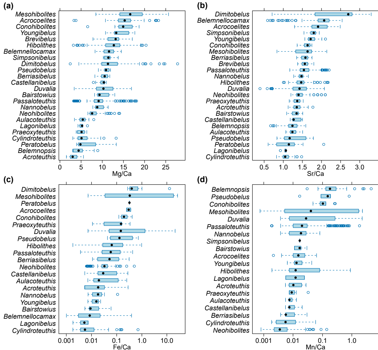
Figure 2. Belemnite rostrum element ratio distributions per genus. (a) Mg/Ca ratios. (b) Sr/Ca ratios. (c) Fe/Ca ratios, log scale. (d) Mn/Ca ratios, log scale. Data taken from entire literature dataset, see text for references.
