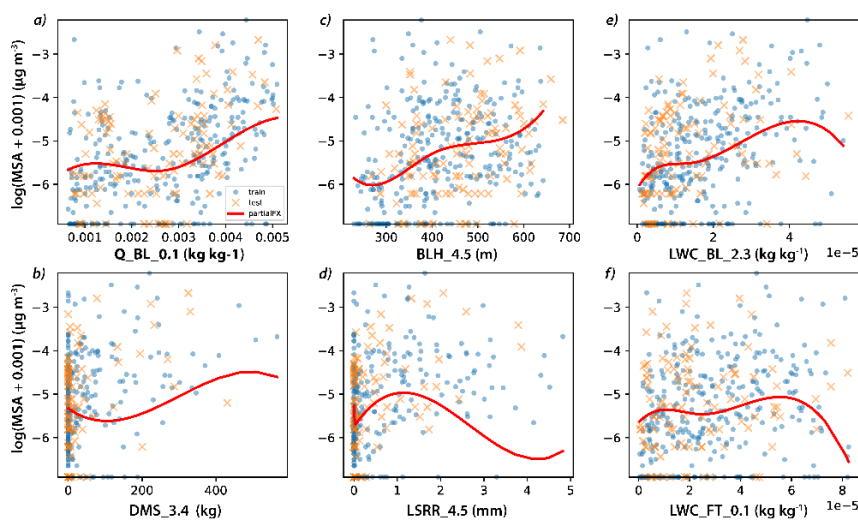
Figure 8: AM-St partial effects for the selected features at Utqiagvik/Barrow. (a) Q BL_0.1 , (b) DMS 3.4 , (c) BLH 4.5 , (d) LSRR 4.5 , (e) LWC BL_2.3 , and (f) LWC FT_0.1 . The red solid line is the partial effect for a different feature in each panel, the blue points are the training observations, and the orange crosses are the test data. Feature abbreviations are defined
