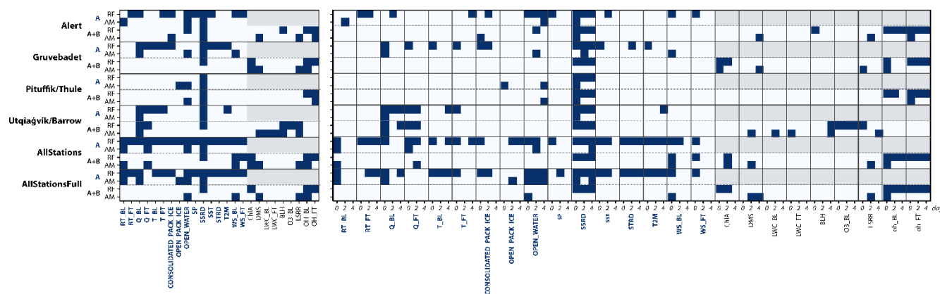
910 Figure 6: Overview of features selected by the RF and AM based on Group A and Group B, by station. The left panel shows selected features grouped over the 0–5 days prior to each MSA_p measurement, and the right panel shows the features grouped for 0–1 (0), 2–3 (2), and 4–5 (4) days before each MSA_p measurement. Features in Group A have their name in boldface and blue type, while the additional features that are only in Group B are in regular black typeface. The grey shaded area indicates that Group B features cannot be chosen in these model runs. St refers to a model trained and tested on the specified station, AS refers to a subset of the data with an equal number of observations from each station, and ASF refers to all data from all four stations and tested only on the specified station. Feature abbreviations are defined in Table 2. Only 915 features selected at least once by a model/station combination are presented in this figure (i.e., if a feature is not included in the figure then it was not selected).
