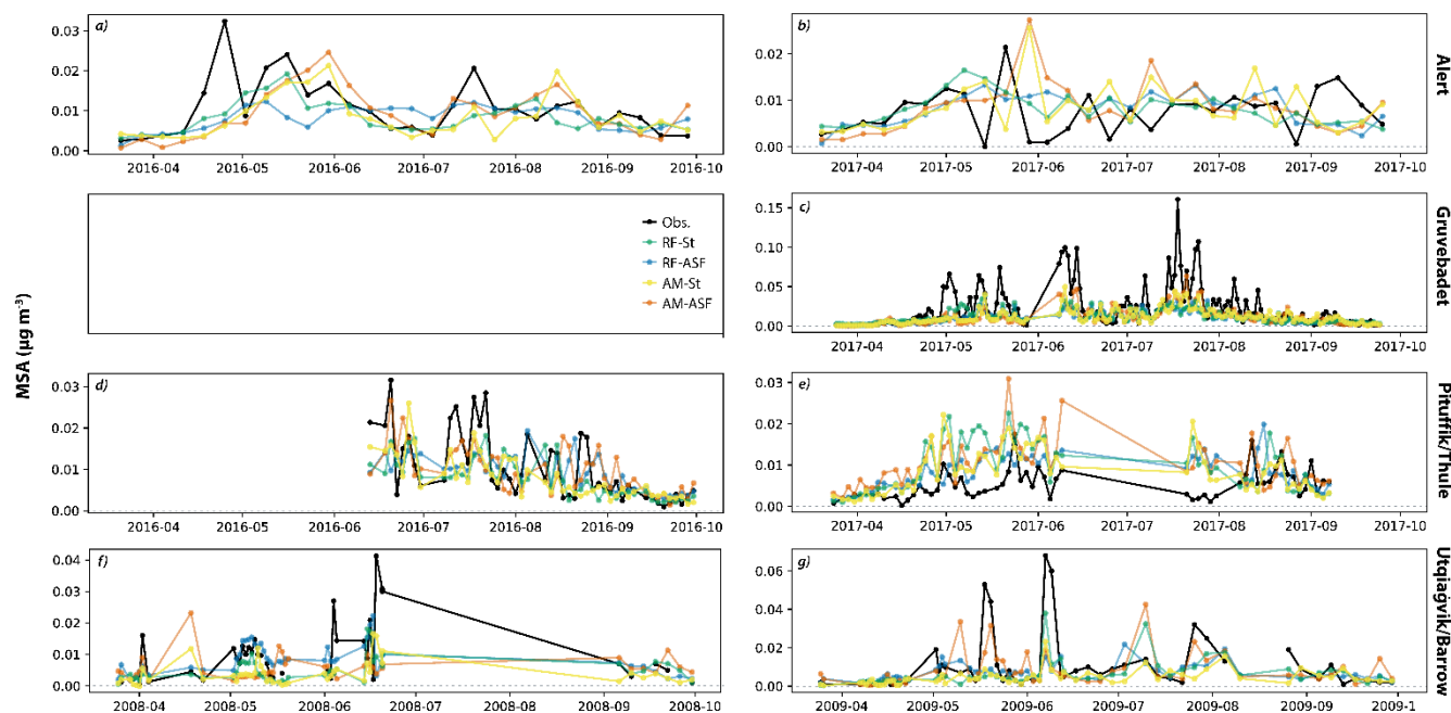
755 Figure 5: Observed and modeled time series of MSA_p for the test dataset at all four stations. (a) and (b) Alert, (c) Gruvebadet, (d) and (e) Pituffik/Thule, and (f) and (g) Utqiagvik/Barrow. St refers to a model trained and tested on the specified station and ASF refers to all data from all four stations and tested only on the specified station. The observations are shown in black. Data from Gruvebadet during 2016 is not available.
