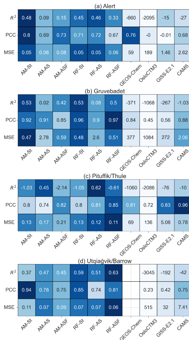
1105 Figure 10. Prediction performance for the data-driven and numerical models on the test set for the four stations for the random forest (RF) and additive model (AM). (a) Alert (b) Gruvebadet, (c) Pituffik/Thule, and (d) Utqiagvik/Barrow. In each panel, R^2 is shown in the top sub-panel, the Pearson correlation coefficient (PCC) in the middle sub-panel, and the mean squared error (MSE) at the bottom. St refers to a model trained and tested on the specified station, AS refers to a subset of the data with an equal number of observations from each station, and ASF refers to all data from all four stations and tested only 1110 on the specified station. MSE is multiplied by 10^4 to display three significant digits. The color scale indicates performance, where the darkest blue signifies the best performance (lowest MSE, highest R^2 - and highest PCC within each row). The MSE, R^2 , and PCC values are calculated according to Eqs. (1), (2), and (3), respectively.
