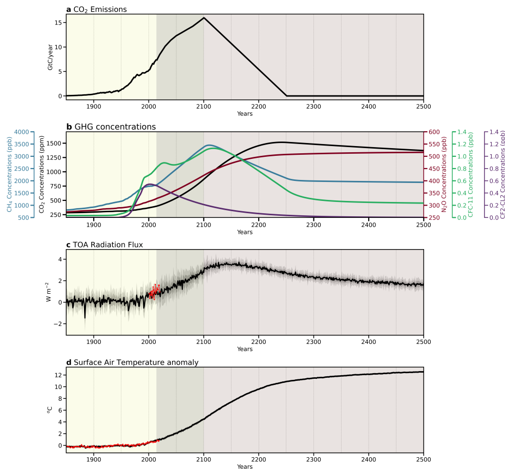
Figure 1: Time series of global mean (a) fossil fuel and industrial CO 2 emissions and (b) greenhouse gas mole fractions over 1850-2500 for the CESM2-LE extension simulations. Values are taken from Meinshausen et al. (2020). Time series of global fields over
