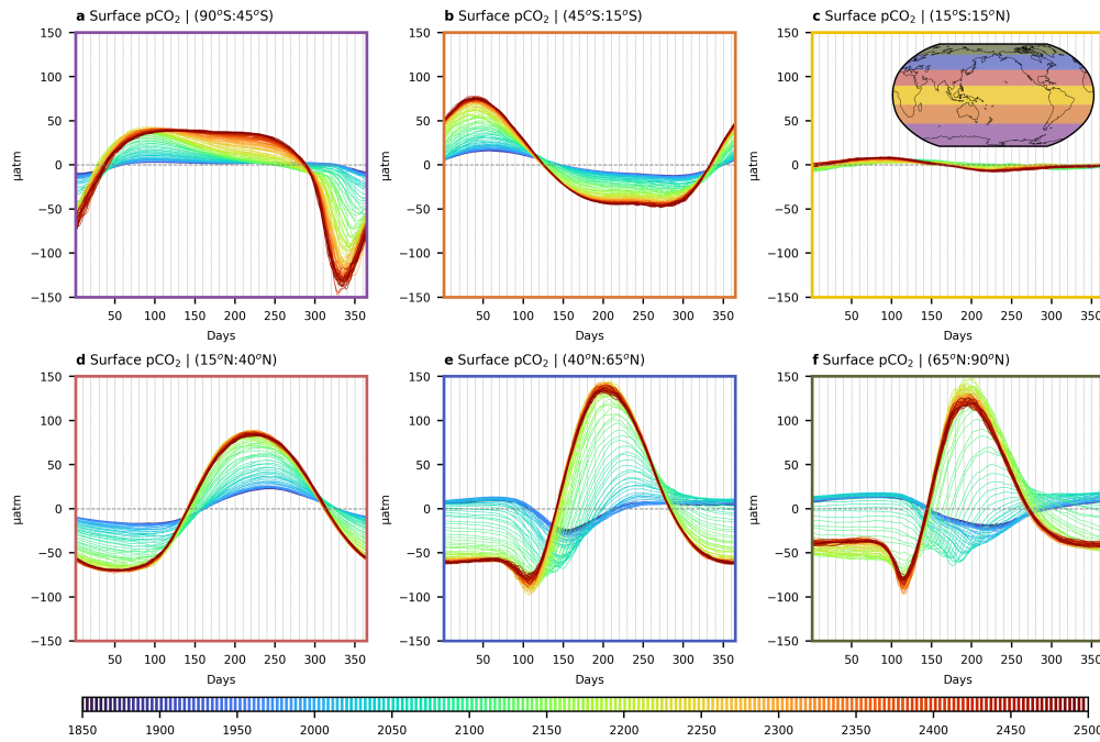
405 Figure 7: Seasonal cycle of ocean p\text{CO}_2 ( \mu\text{atm} ) along latitudinal bands in 5-year intervals. (a) 90°S-45°S, (b) 45°S-15°S, (c) 15°S-15°N, (d) 15°N-40°N, (e) 40°N-65°N, and (f) 65°N-90°N.
