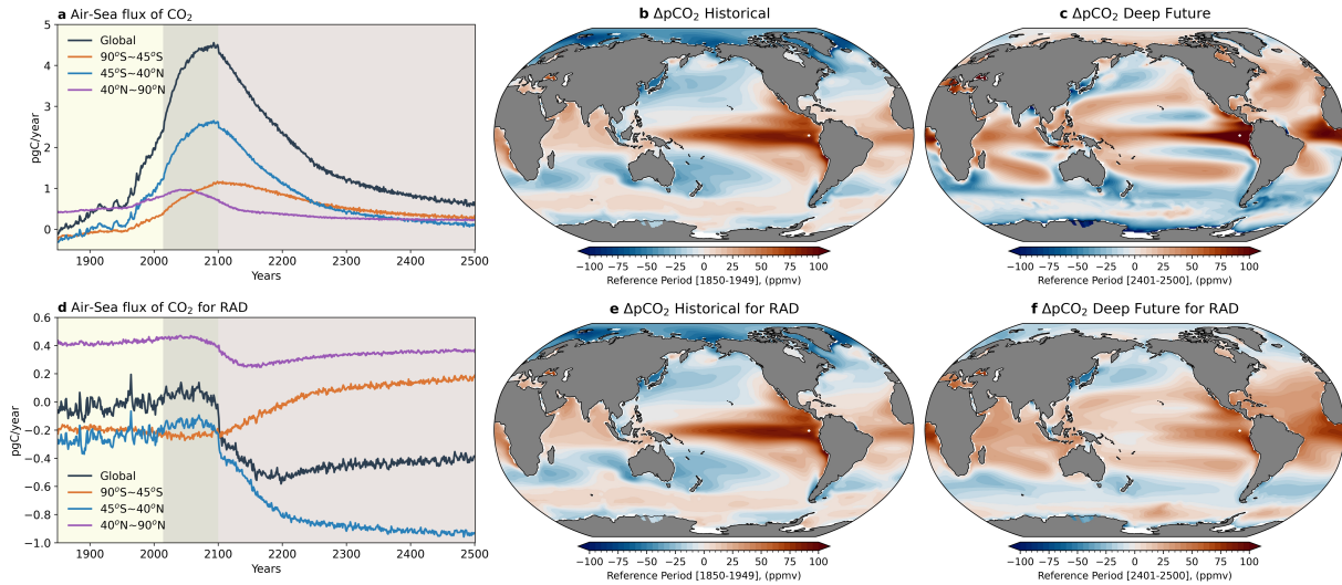
Figure 12: Changes in surface ocean carbon state and fluxes. (a) Spatially integrated air-sea CO 2 fluxes (PgC year -1 ) for the ensemble mean considered globally (black), 90°S-45°S (orange), over 45°S-40°N (blue), and over 40°N-90°N (purple), where a 12-month running mean has been applied to the ensemble mean to remove seasonal variations, and positive values indicating ocean uptake of carbon. (b) ΔpCO 2 (ppmv) averaged over the 1850-1949, taken as the difference between oceanic and atmospheric pCO 2 and (c) ΔpCO 2 averaged over the 2401-2500. Positive values occur where there is outgassing. (d-f) Same as (a-c) except for RAD case (i.e., the system is radiatively coupled, but pre-industrial CO 2 concentrations are maintained for air-sea gas exchange).
