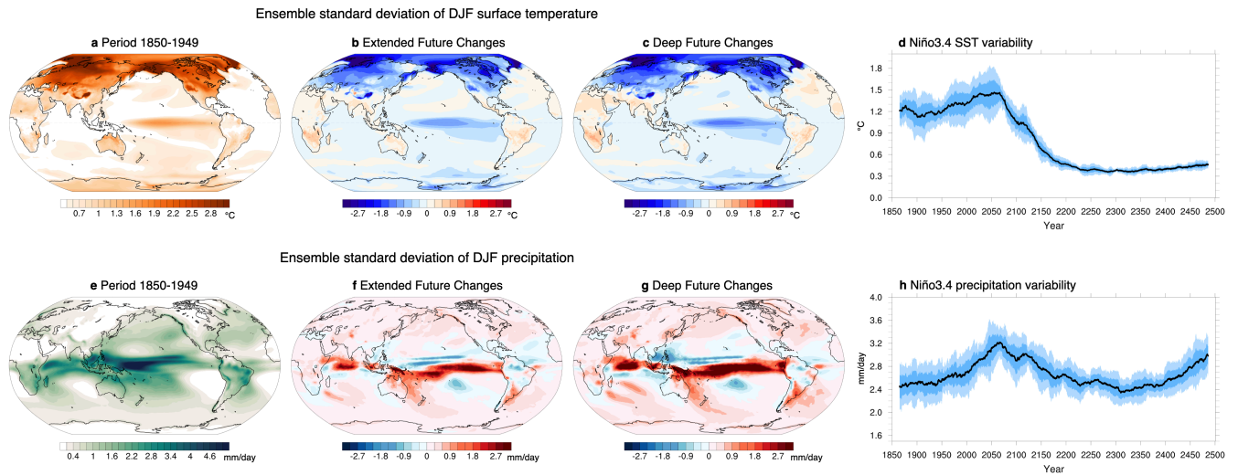
295 Figure 4: Time-averaged across-ensemble standard deviation of the boreal winter (DJF) mean (a) surface temperature (°C) and (e) precipitation (mm day -1 ) over the period 1850-1949. Future changes of the standard deviation values of (b, c) surface temperature and (f, g) precipitation over the period 2150-2249 and over the period 2401-2500, respectively, relative to 1850-1949. These calculations involve first determining the standard deviation across all ensemble members for the same time period, followed by averaging across time. (d, h) 30-year running standard deviations of monthly Niño3.4 SST and precipitation, respectively.
