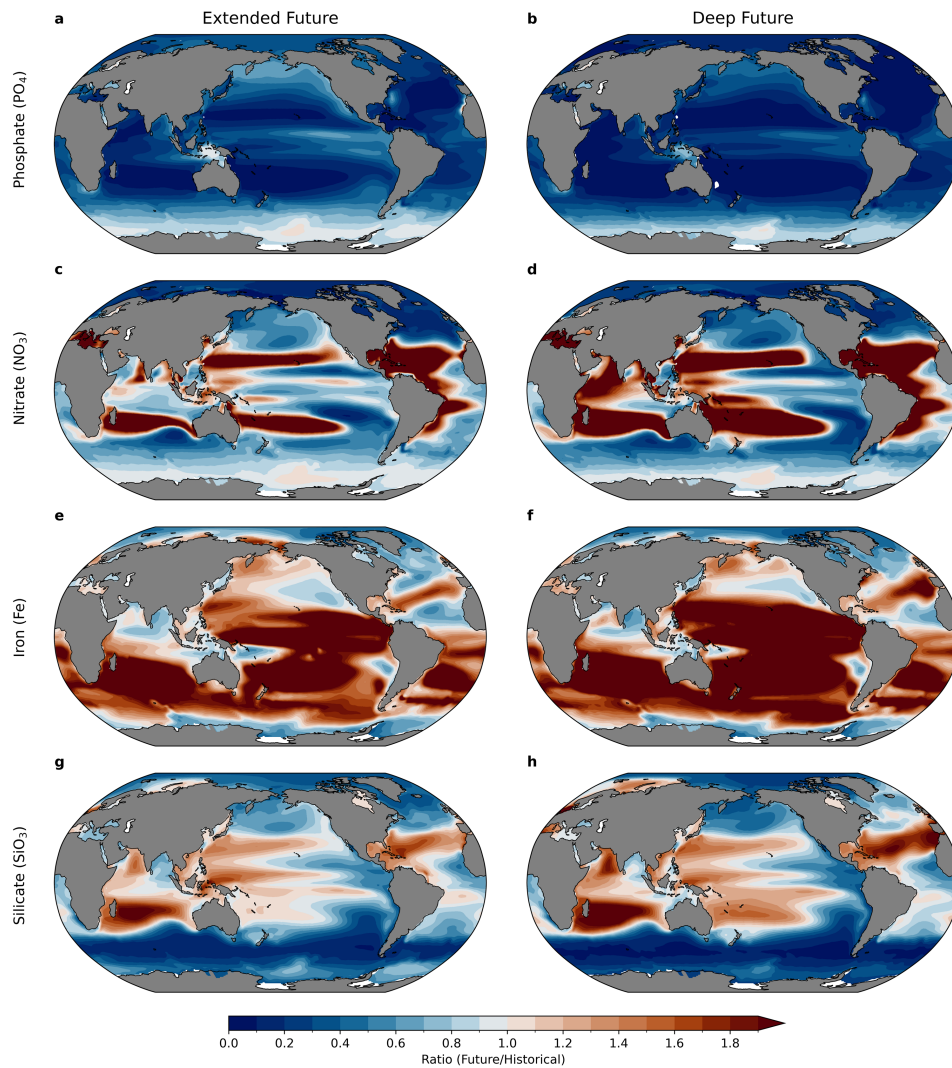
495 Figure 10: The changes in the future period 2150-2249 (first column) and period 2401-2500 (second column) relative to the historical period 1850-1949. (a, b) \text{PO}_4 ( \text{mmol m}^{-3} ), (c, d) \text{NO}_3 ( \text{mmol m}^{-3} ), (e, f) \text{Fe} ( \text{mmol m}^{-3} ), and (g, h) \text{SiO}_3 ( \text{mmol m}^{-3} ). The changes were calculated as the ratio of future to historical periods. Blue ( <1.0 ) and red ( >1.0 ) indicate future decreases and increases, respectively, relative to the historical period. All values are averaged over the upper 100 m depth.
