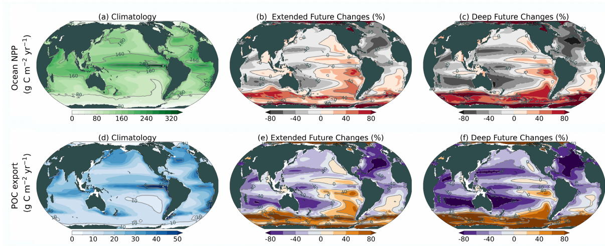
Figure 9: Historical climatology (period 1850-1949) (first column), and future perturbations over the period 2150-2249 (second column) and over the period 2401-2500 (third column), relative to 1850-1949. (a-c) Ocean NPP ( \text{gC m}^{-2} \text{yr}^{-1} ) and (d-f) POC export ( \text{gC m}^{-2} \text{yr}^{-1} ).
