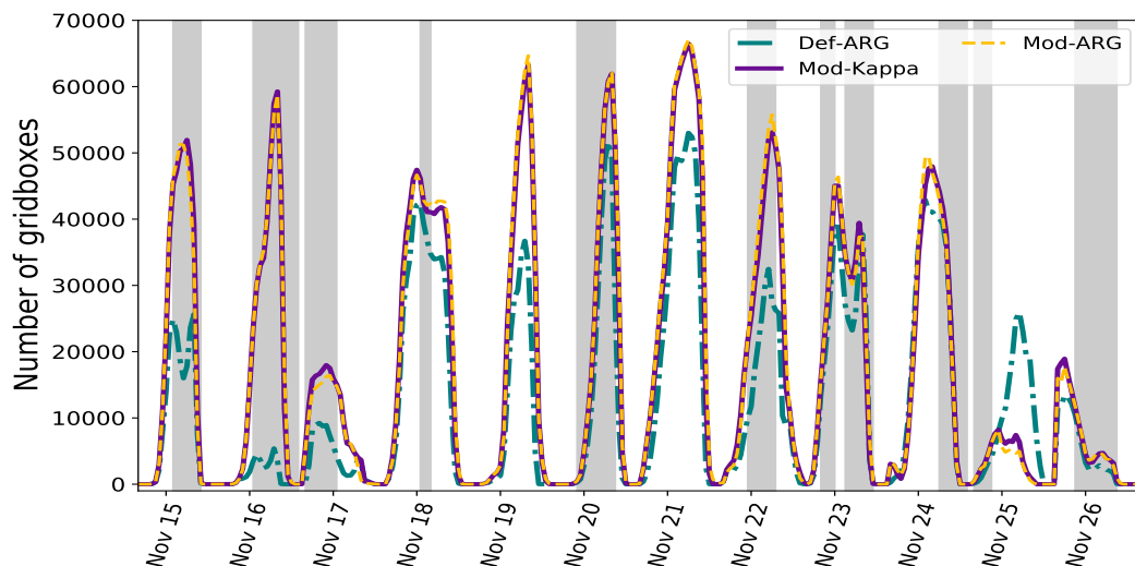
Figure 4. Timeseries of number of foggy gridboxes (at the surface) from the 500 m-resolution model for simulations Def-ARG, Mod-ARG and Mod-Kappa. If the entire domain was foggy, the total would be 67600 ( 260 \times 260 ). Foggy periods in the observations are shown in shaded grey. Tick marks on the x axis are at midnight UTC time.
