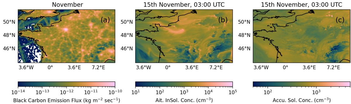
Figure 7. Subfigure (a) shows the black carbon emission flux at the surface from the high resolution EDGAR-HTAP inventory, in the 4 km model for the month of November. Hotspots such as London and Paris can be identified. Subfigure (b) shows the Aitken insoluble mode number concentration and (c) shows the accumulation soluble mode particle number concentration, as simulated by the 4 km model in simulation Def-ARG near the surface at 03:00 UTC on 15 th Nov.
