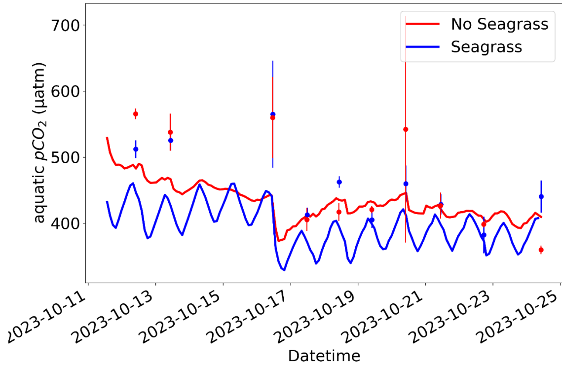
Figure S 2. pCO 2 water sample results plotted on top of the equilibrated water side points for SEACOW1 and 4. SEACOW1 was in the control tank (red), and SEACOW4 was in the seagrass tank (blue). The error bars are the standard deviation of the pCO 2 values.
