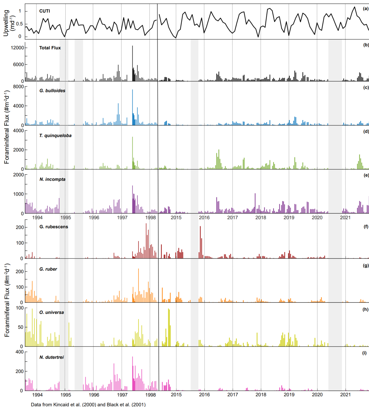
360 Figure 7: Timeseries of CUTI (a) and SBB sediment trap foraminiferal flux from Kincaid et al. (2000) and Black et al. (2001) (left) and this study (right). Total flux (b) and the three most abundant species, G. bulloides (c), T. quinqueloba (d), and N. incompta (e). Major subtropical species are shown in warm colors: G. rubescens (f), G. ruber (g), O. universa (h), and N. dutertrei (i). Gray shading indicates periods without sample collection.
