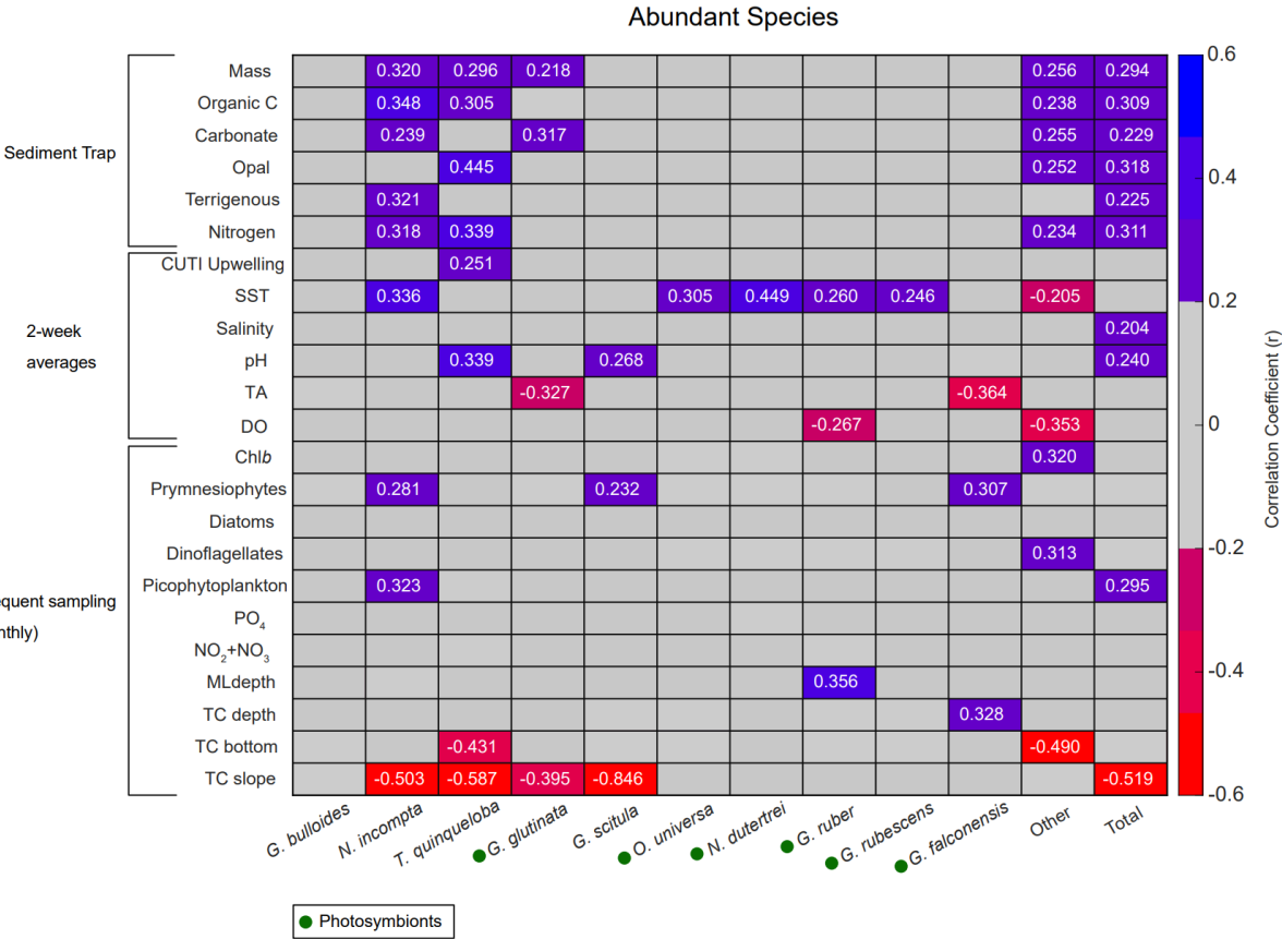
Figure 5: Correlation matrix of abundant species flux (x axis) with environmental parameters (y axis). Pearson correlation coefficients (r) for statistically significant correlations ( p < 0.05 ) are listed as numbers. Blue shades represent positive correlations, and red shades represent negative correlations. Gray represents correlation coefficients < 0.2 . Presence of photosymbionts based on Takagi et al. (2019), Schiebel and Hemleben (2017), and Meilland et al. (2022) is represented by green circles.
