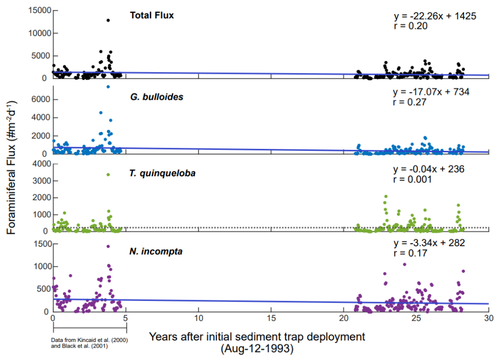
705 Figure A3: Linear regression from 1993-2021 for total foraminiferal flux and the three most abundant species in SBB. Best fit lines represent rate of change of foraminiferal flux in units of foraminiferal flux per year.
