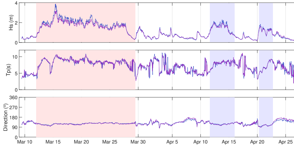
Figure 6. Hydrodynamic analysis of the campaign. Blue line corresponds to M1-T1 and purple line to M2-T2 . Red rectangle shows the period when Celia storm Celia hit the coast. Blue rectangles show the two minor storms that occurred during the campaign period.
