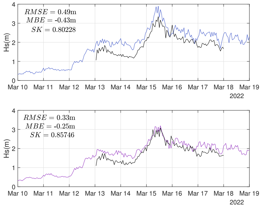
Figure 8. Hydrodynamic response validation of the model. Top panel and the light blue line corresponds to M1-T1 while bottom panel and purple line to M2T2 . Black lines show the model output for each point.
