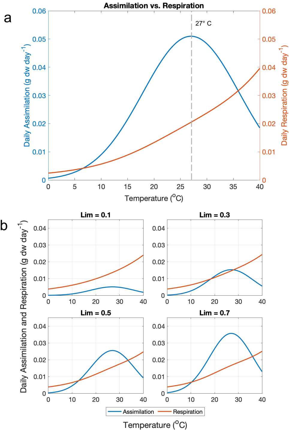
Figure S1. Daily assimilation and respiration rates of Eastern oysters as a function of temperature as simulated by the EcoOyster model. Rates are shown (a) assuming no limitation on filtration ( \text{Lim} = 1 ) and (b) when filtration is limited by other environmental conditions. ( \text{Lim} = a dimensionless product of limiting functions of salinity, TSS, dissolved oxygen, and chl a ).
