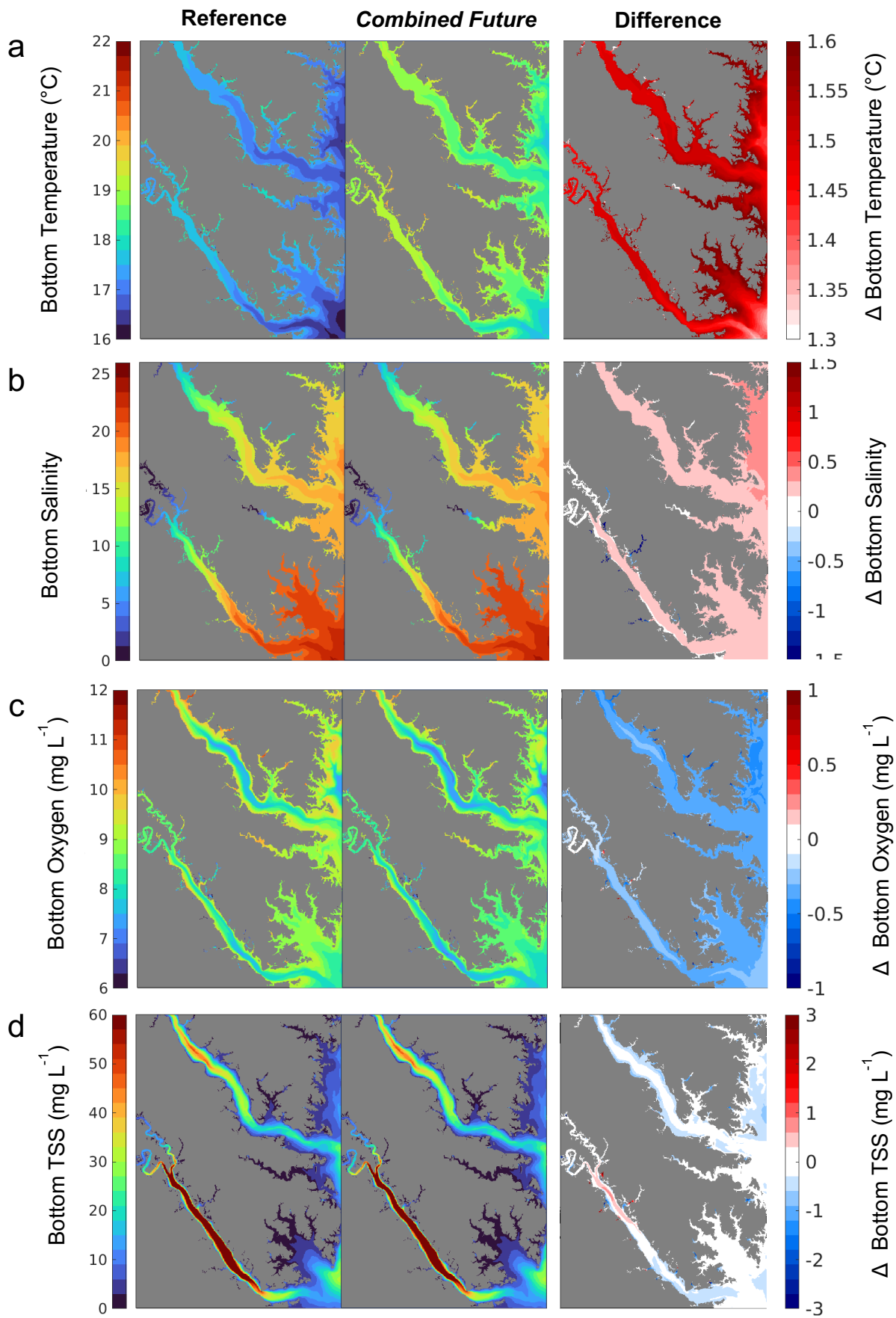
Figure S3. Annual mean ROMS-ECBO bottom (a) temperature, (b) salinity, (c) \text{O}_2 , and (d) TSS from the reference run, the Combined Future simulation, and Combined Future minus reference.
