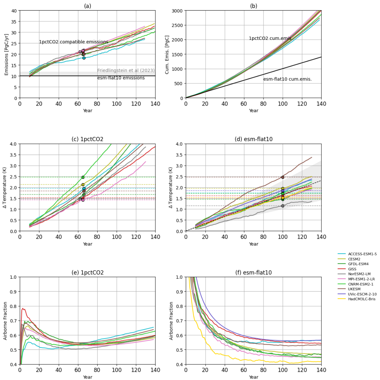
355 Figure 6: Comparative ESM results for TCRE calculation using 1pctCO 2 and esm-flat10, showing [a,b] compatible [annual,cumulative] emissions in 1pctCO 2 compared with the constant 10PgC/yr flux in esm-flat10. Annual total anthropogenic carbon emissions in 2023 are shown for context . [c,d] show temperature evolution in [1pctCO 2 ,esm-
