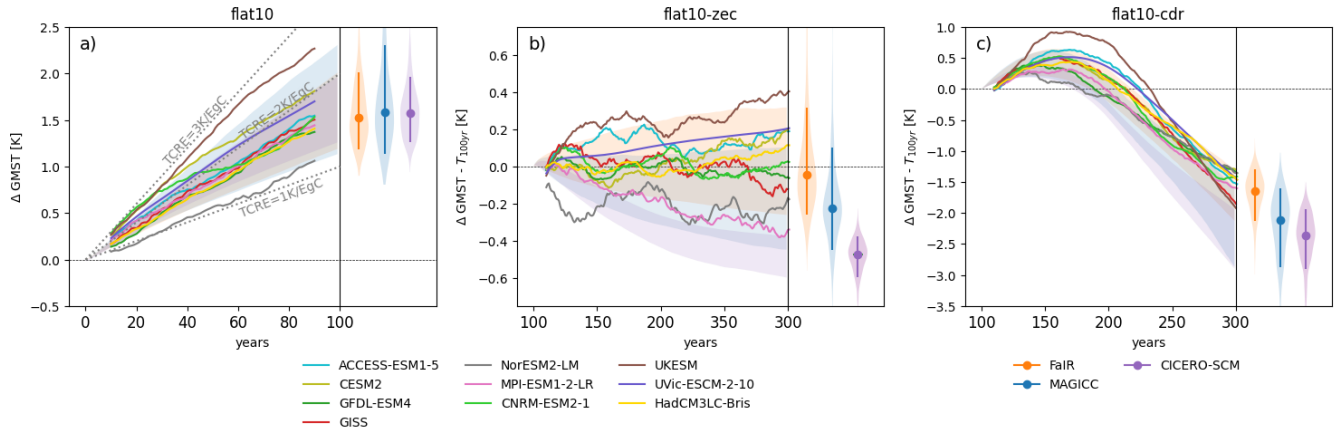
Figure 3: Summary results for global mean surface temperature (GMST) response in the trial flat10MIP. Colored lines indicate temperature change from (a) pre-industrial levels (b,c) T_{100\text{yr}} (the average temperature in years 91-110 in esm-flat10 ) in each of the participating ESMs. Shaded regions refer to the Simple Climate Models' probabilistic distribution ranging the 10th-90th percentiles. This distribution is shown as violin plots for the last time step of each scenario, where the shading shows the full range of results, and the vertical line indicates the 10th-90th percentiles with the median in the center. A 20-year moving average is applied to all time series.
