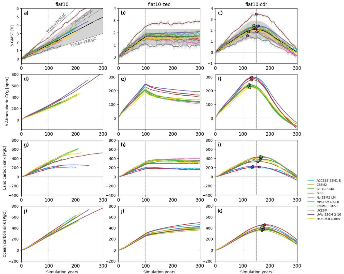
Figure 4: ESM results. Columns represent global indicators from ESM simulations running esm-flat10 (left), esm-flat10-zec (center) and esm-flat10-cdr (right). Panels a)–c) show changes in GMST with the dashed black line and gray shading denoting central estimate and range derived from cumulative emissions assuming a linear TCRE relationship as given in AR6 (TCRE=1.65 K, likely range 1.0 – 2.3 K) for reference. Panels d)–f) illustrate changes in atmospheric CO 2 concentrations as a function of time. Panels g)–i) show cumulative carbon absorption by the land surface. Panels j)–l) show cumulative absorption of carbon by the ocean over time. The circles for the esm-flat10-cdr experiments indicate the maximum of each time series. A 20-year moving average is applied for the GMST time series (bold line), faint line shows original data.
