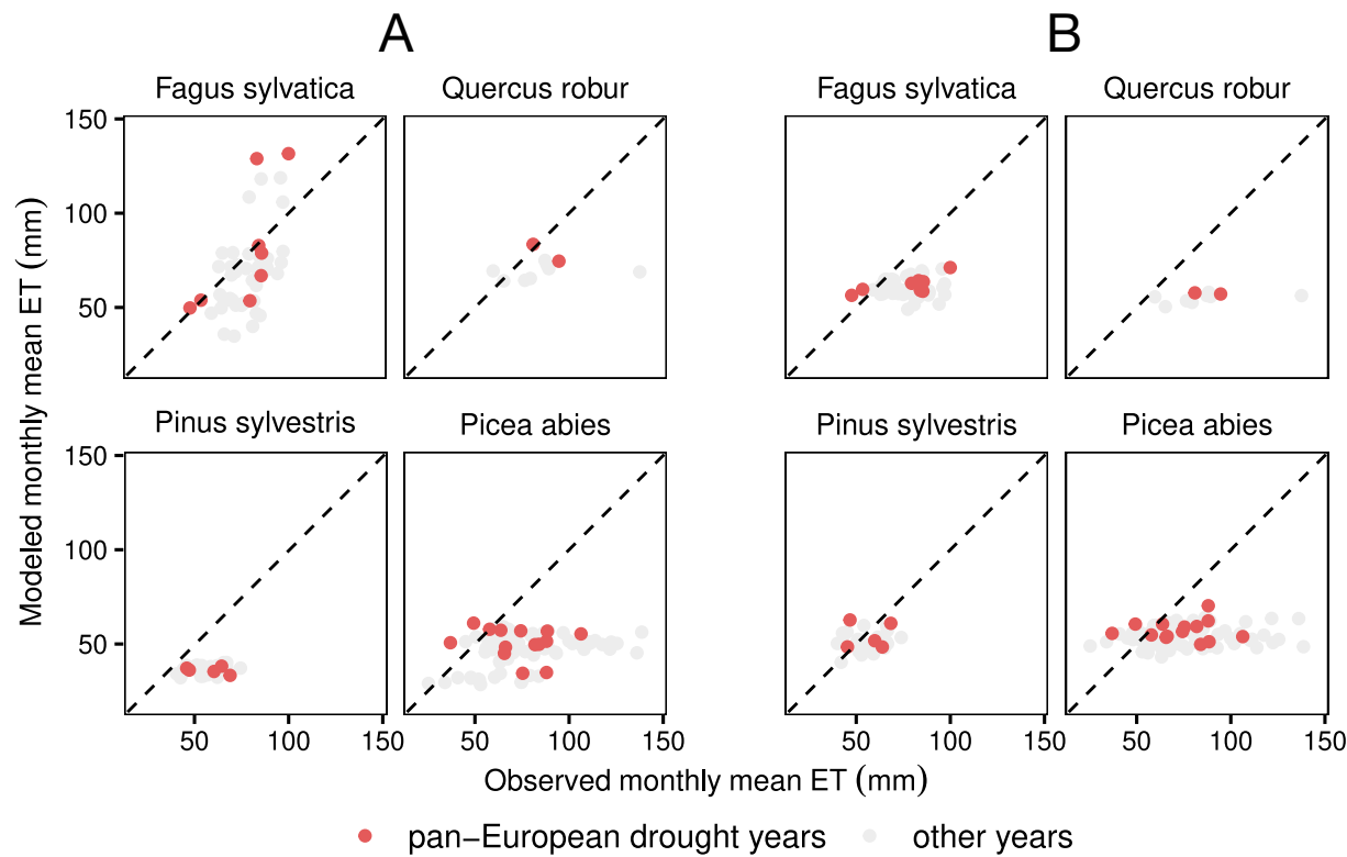
A1: Species-specific comparison of modeled evapotranspiration and evapotranspiration from eddy-covariance flux towers
