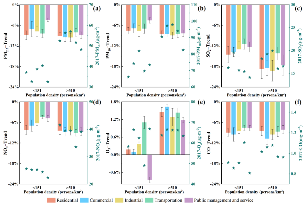
Figure 10. Annual variation trend of PM_{2.5} (a), PM_{10} (b), SO_2 (c), NO_2 (d), O_3 (e), and CO (f) concentrations in various functional zones in different urban scale. (The left y-axis presents the temporal variation in pollutant concentrations from 2017 to 2022, the right y-axis displays the pollutant concentrations in 2017.)
