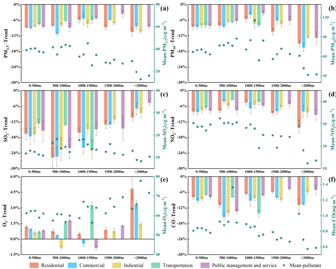
Figure 9. Annual variation trend of PM_{2.5} (a), PM_{10} (b), SO_2 (c), NO_2 (d), O_3 (e), and CO (f) concentrations in various functional zones at different altitudes. (The left y-axis presents the temporal variation in pollutant concentrations from 2017 to 2022, the right y-axis displays the mean pollutant concentrations over the same period.)
