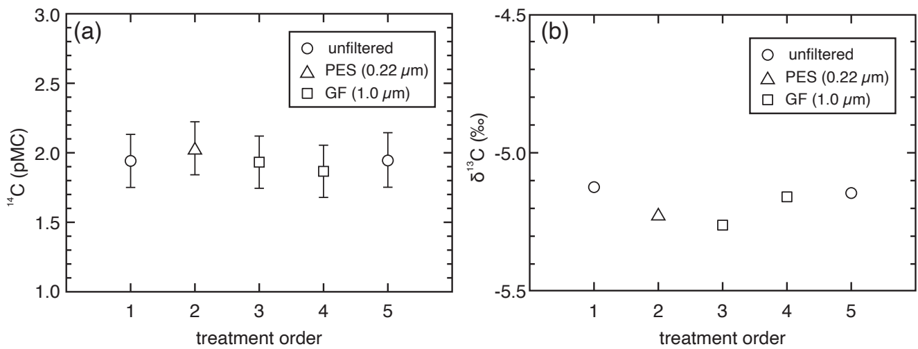
190 Figure 1: Comparisons of ^{14}\text{C} (a) and \delta^{13}\text{C} (b) among the unfiltered and filtered solutions of 1 \text{ mmol}\cdot\text{L}^{-1} of \text{NaHCO}_3 . PES: filtered by PES disk filter (25 mm in diameter, 0.22 \mu\text{m} in pore size), GF: filtered by GF disk filter (25 mm in diameter, 1.0 \mu\text{m} in pore size). Each value of ^{14}\text{C} and \delta^{13}\text{C} represents a single treatment occasion. The bars of ^{14}\text{C} concentration represent the measurement error of the AMS analysis. The \delta^{13}\text{C} error is smaller than the size of the plotting symbols.
