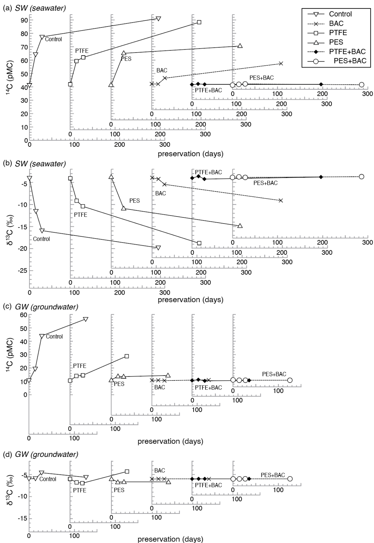
240 Figure 2: Changes in ^{14}\text{C} and \delta^{13}\text{C} during the preservation of SW and GW mixed with \text{NaHCO}_3 solution and beet sugar. Changes in DIC were augmented by the addition of beet sugar. (a) ^{14}\text{C} of SW, (b) \delta^{13}\text{C} of SW, (c) ^{14}\text{C} of GW, (d) \delta^{13}\text{C} of GW. The time series of DIC change for the respective treatments were derived from each experiment conducted on a single sample with varying preservation periods. The errors of ^{14}\text{C} and \delta^{13}\text{C} are equivalent to or smaller than the size of the plotting symbols.
