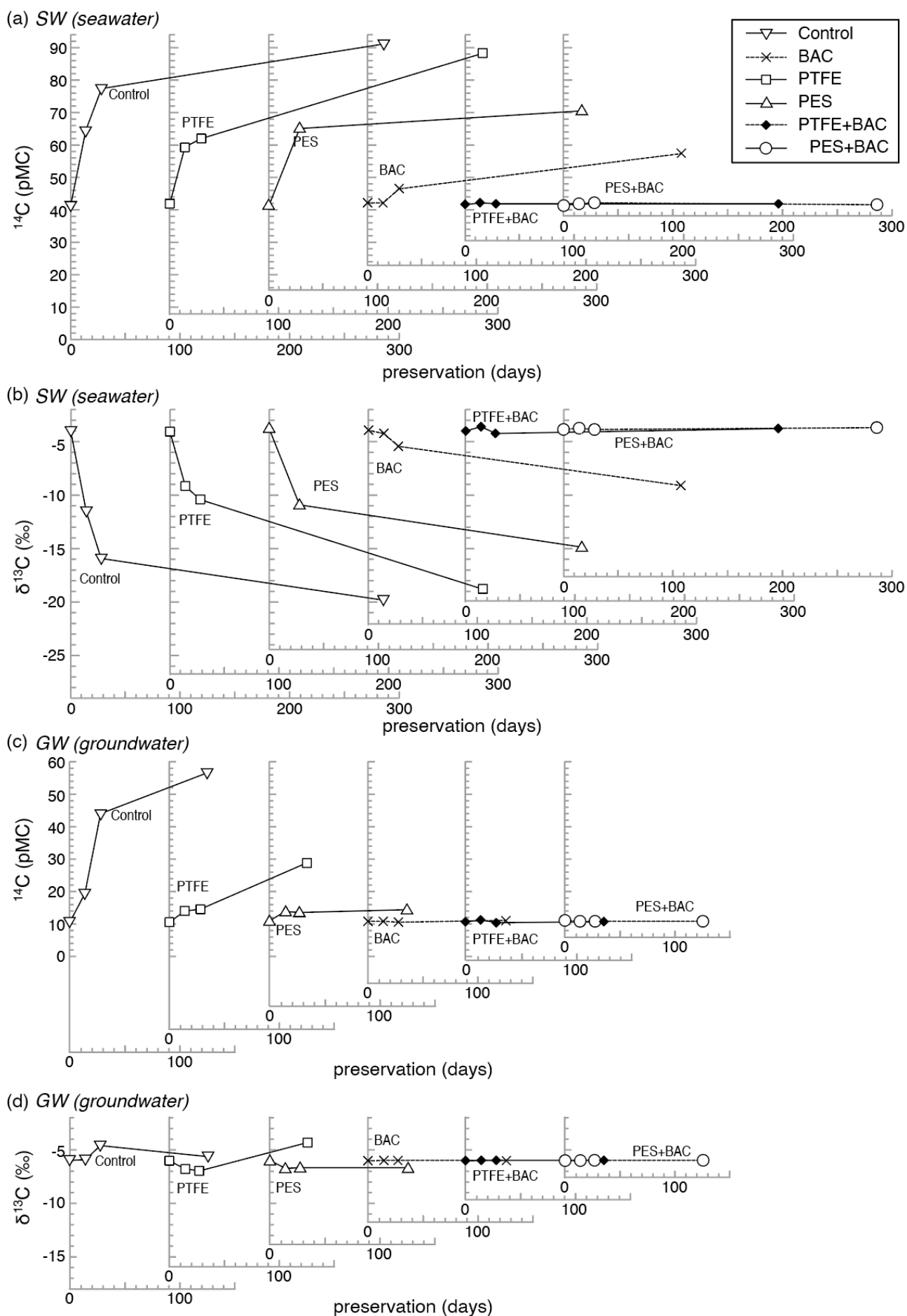
Figure 2: Changes in ^{14}\text{C} and \delta^{13}\text{C} during the preservation of SW and GW mixed with \text{NaHCO}_3 solution and beet sugar. Changes in DIC were augmented by the addition of beet sugar. (a) ^{14}\text{C} of SW, (b) \delta^{13}\text{C} of SW, (c) ^{14}\text{C} of GW, (d) \delta^{13}\text{C} of GW. The time series of DIC change for the respective treatments were derived from each experiment conducted on a single sample with varying preservation periods. The errors of ^{14}\text{C} and \delta^{13}\text{C} are equivalent to or smaller than the size of the plotting symbols.
