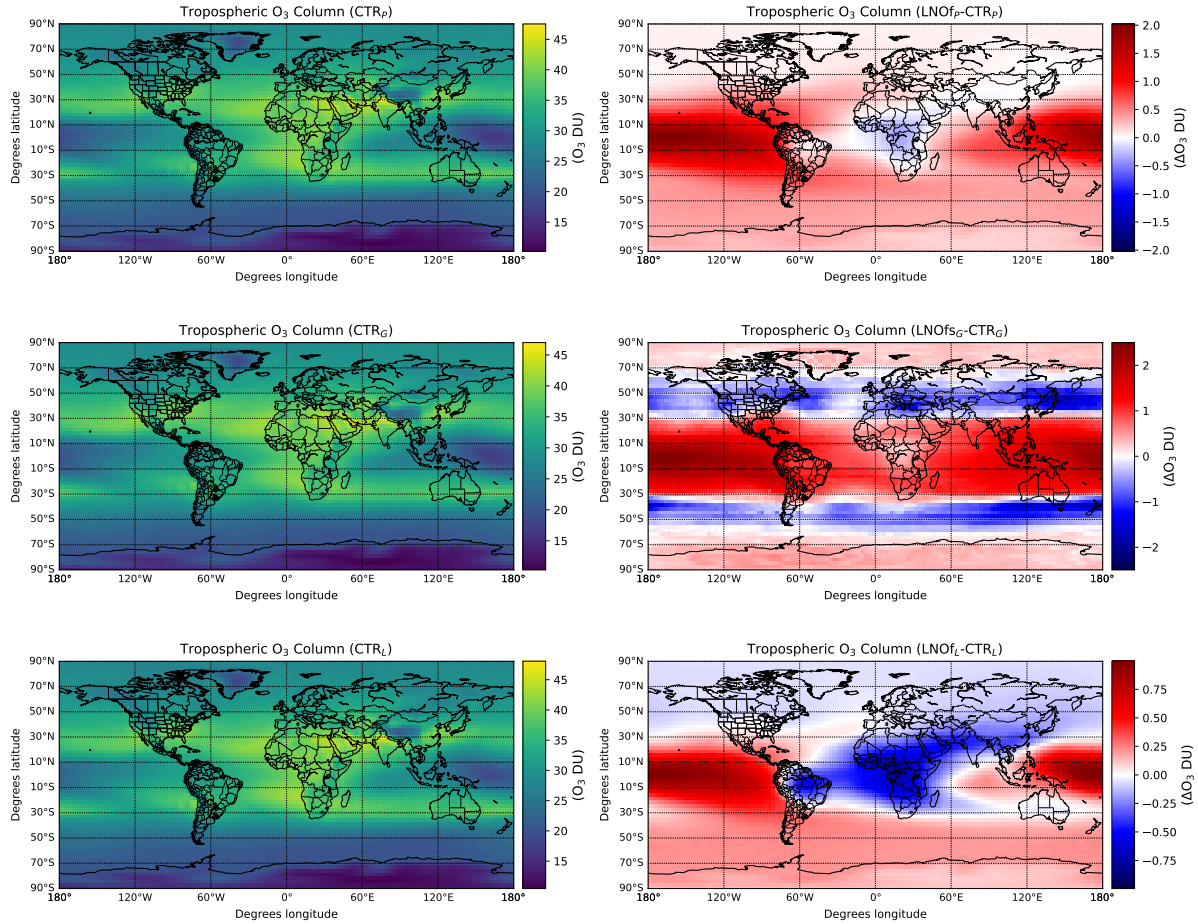
Figure 15. Annually (2002-2007) and globally averaged tropospheric column of O_3 in the CTR simulations (left panels) and differences of the O_3 total column (integrated between the ground and the top of the troposphere) between the simulations LNOFs and CTR (right panels). The values are given in Dobson Units (DU). The subscript indicates the used lightning parameterization: P : Price and Rind (1992), G : Grewe et al. (2001), and L : Luhar et al. (2021) (see Table 1). The monthly total O_3 column from the CTR_G simulation can be seen in Figures S14-S25.
