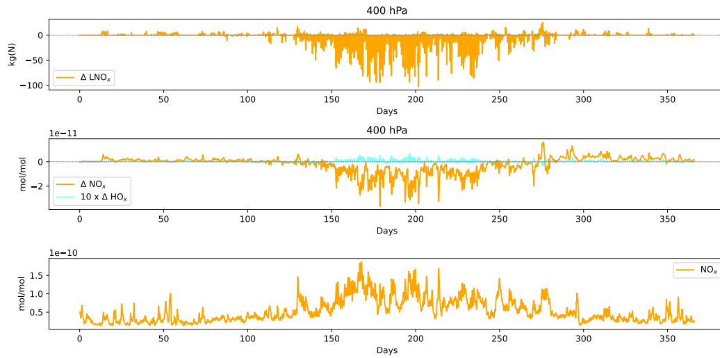
Figure 10. (Upper panel): Difference in the hourly total column production of \text{LNO}_x between the \text{LNOfs}_L and \text{CTR}_L simulations over a 1-year period (day 1 corresponds to 1 January, 2000). (Middle panel): Hourly differences in the mixing ratios of \text{NO}_x and \text{HO}_x at the 400 hPa. (Lower panel): Hourly background mixing ratio of \text{NO}_x at the 400 hPa level in the \text{LNOfs}_L simulation. The three panels correspond to a spatial average over Europe (bounded by 42^\circ\text{N} and 52^\circ\text{N} latitude degrees, and 0^\circ to 24^\circ\text{E} longitude degrees). The subscript P indicates the used lightning parameterization: Price and Rind (1992).
