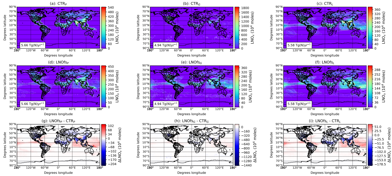
Figure 2. Daily mean LNO x production ( \times 10^4 moles) in June-July-August (JJA) per 2.8^\circ latitude \times 2.8^\circ longitude box obtained from the CTR (a-c) and the LNOs (d-f) simulations. Panels (g-i) shows the difference between CTR and the LNOs simulations. Note that the color scales are different in each panel.
