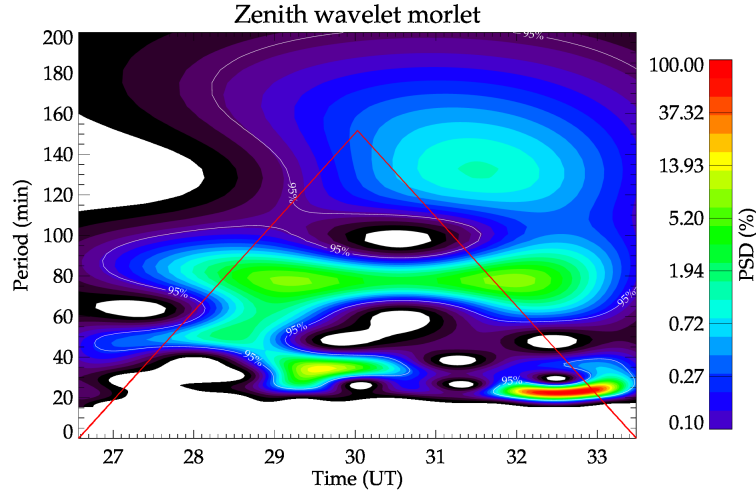
Figure 7. The wavelet power spectrum of the zenith time series for the keogram depicted in Figure 2b illustrates all the recorded MSGW periods. The power spectrum is normalized as a percentage relative to its maximum and minimum values.
