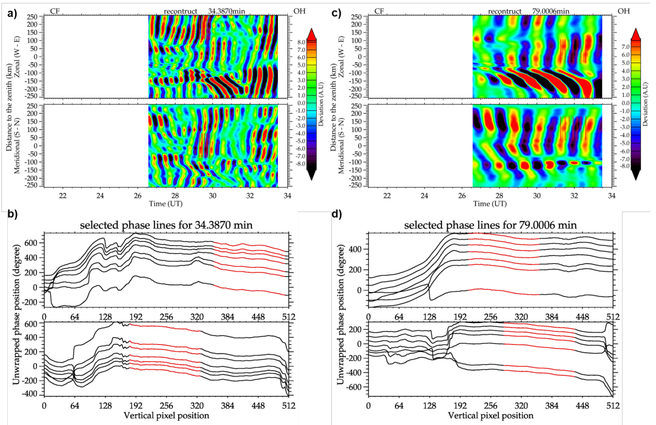
Figure 8. Reconstructed keogram for the 35-minute and 79-minute peak periods, visible between 29 and 30 UT and 31 and 33 UT. The red lines depicted in panels a) and c) are highlighted in panels b) and d). They were used to calculate the MSGW parameters.
