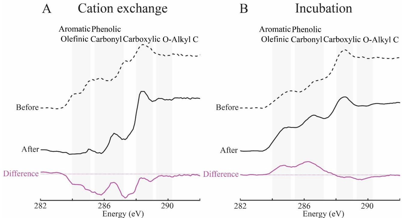
Fig. 2. Targeted experiments demonstrate the importance of decomposition processes in the formation of the co-location of Ca with a characteristic fraction of soil organic carbon. A.) The exchange of Ca with potassium (KCl) disrupted the carbon co-located with Ca (Fig. S8), reducing the associated aromatic and phenolic carbon in the C_{1s} near-edge X-ray absorption fine structure (NEXAFS) spectra, and upon addition ( CaCl_2 ), Ca re-associates with the remaining carbon (Fig. S8 & S9A). This remaining carbon has a spectrum like the carbon co-located with iron in unaltered samples (Fig. 1C), which was ultimately resistant to cation-exchange. B.) Incubation with added Ca reduced the O-alkyl carbon content in NEXAFS spectra while increasing the relative abundance of aromatic and phenolic carbon in the remaining sample (Fig. S9B). Thereby, microbial decomposition in the presence of added Ca reproduced a spectrum that was like the Ca-carbon spectrum of unaltered samples at the Grassland and Forest (Fig. 1C; Fig. S6). These experiments were run on two different samples from the same site explaining slight differences in the initial NEXAFS spectra, see methods for details.
