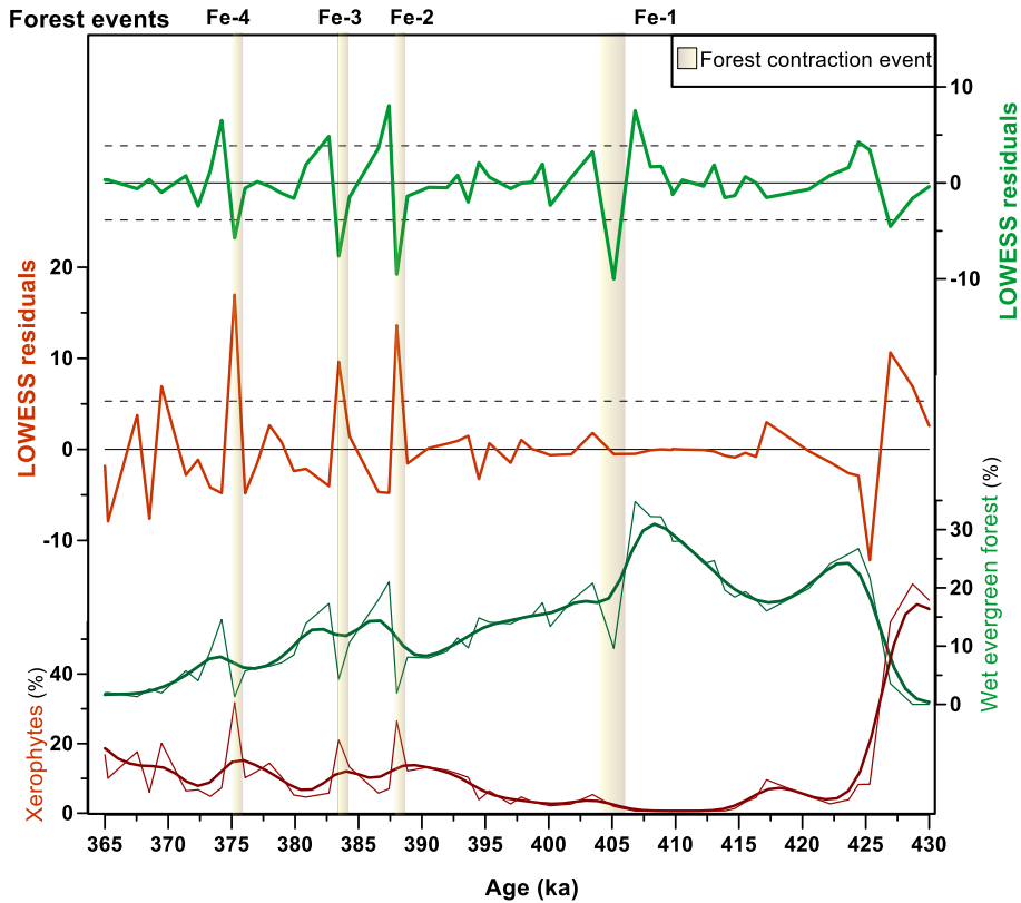
Fig. 3. Pollen percentage curves of the xerophyte plants and the wet evergreen forest (bottom panel) along with the respective Gaussian smoothing filter LOWESS smoothing (7 ky-Gaussian filter \alpha = 0.2 , bold line) and the residuals (top panel) during MIS 11. Millennial-scale forest expansion and contraction events (green and brown bands, respectively) were identified when at least one sample of the model residuals exceeded the threshold of one standard deviation ( \pm 1\sigma ). Significant forest contractions occurring during the glacial inception were also concomitant with pronounced increases in xerophyte taxa percentages surpassing 1\sigma of their residual values, and were followed by significant expansions of wet evergreen tropical forest taxa.
