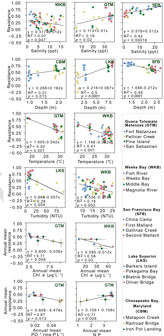
Figure 4. Relationships between resistance and physicochemical factors for each estuary. Significant correlations ( p < 0.05 ) are shown with black lines. Standard errors of the mean are shown in vertical and horizontal black lines for relationships using annual means for chlorophyll a (Chl a ), \text{PO}_4^{3-} , and N:P. For additional results see Figs. S11, S12, and S14.
