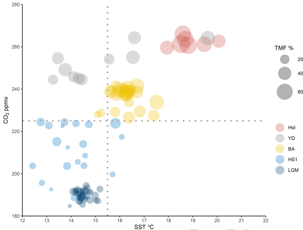
Figure 5. Dispersion plot showing the relation between CO 2 (Marcott et al., 2014) and SST in relation to TMF % across the different intervals of the Last deglaciation, following the pollen zones boundaries.
