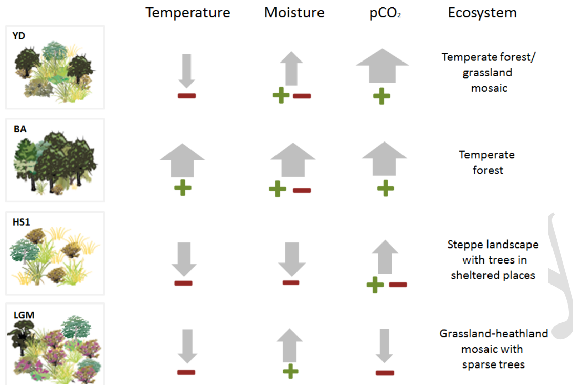
Figure 4. Schematic representation of the relative change of climatic inferred parameters (precipitation and temperature) based on pollen-vegetation groups, biomarkers, SST as well as the physiological contribution of CO 2 for each period showing a schematic reconstruction of the potential ecosystem scenarios. The perceived temperature used the interpretation of pollen (TMF and STE groups), SST and n -alkanes; the plant available moisture (ERI, TMF and STE).
