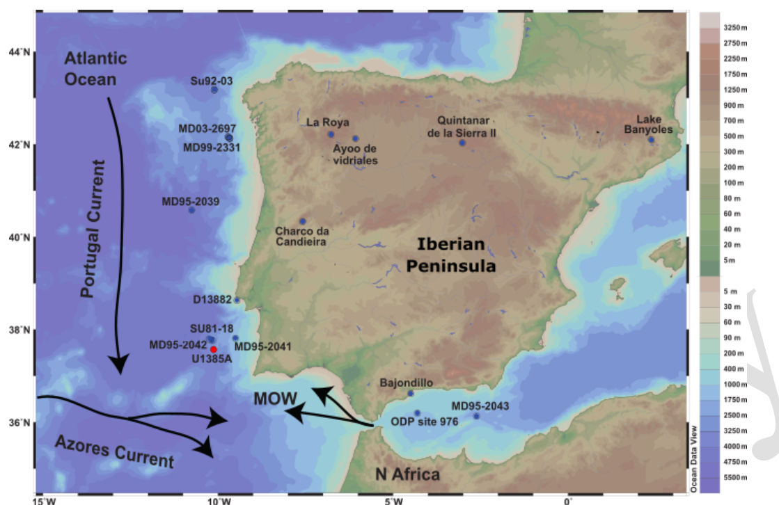
Figure 1. Location of IODP Site U1385 and of the marine and terrestrial pollen records discussed in the text. Marine sedimentary records: MD03-2697 (Naughton et al., 2016); MD99-2331 (Naughton et al., 2007); MD95-2039 (Roucoux et al., 2005); D13882 (Gomes et al., 2020); MD95-2043 (Fletcher and Sánchez Goñi, 2008); MD95-2042 (Chabaud et al., 2014); SU81-18 (Turon et al., 2003); ODP Site 976 (Comboureu Nebout et al., 2009); Continental sedimentary records: Lake de Banyoles (Pèrez-Obiol and Julià, 1994); Quintanar de la Sierra II (Peñalba et al., 1997); La Roya (Allen et al., 1996); Ayoo de vidriales (Morales-Molino and García-Anton, 2014); Charco da Candieira (Van der Knaap and van Leeuwen, 1997); Padul 15-05 (Camuëra et al., 2019). Black arrows represent the surface water circulation (MOW, Portugal and Azores Current). Note that coastline boundaries are for the present day. From: Schlitzer, Reiner, Ocean Data View, https://odv.awi.de , 2019 (last access: 9 May 2020).
